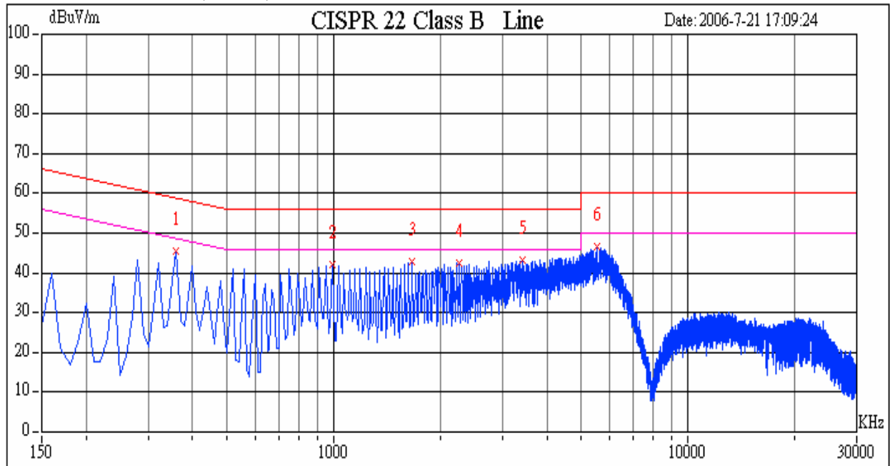
Conducted emissions (Line 2)
