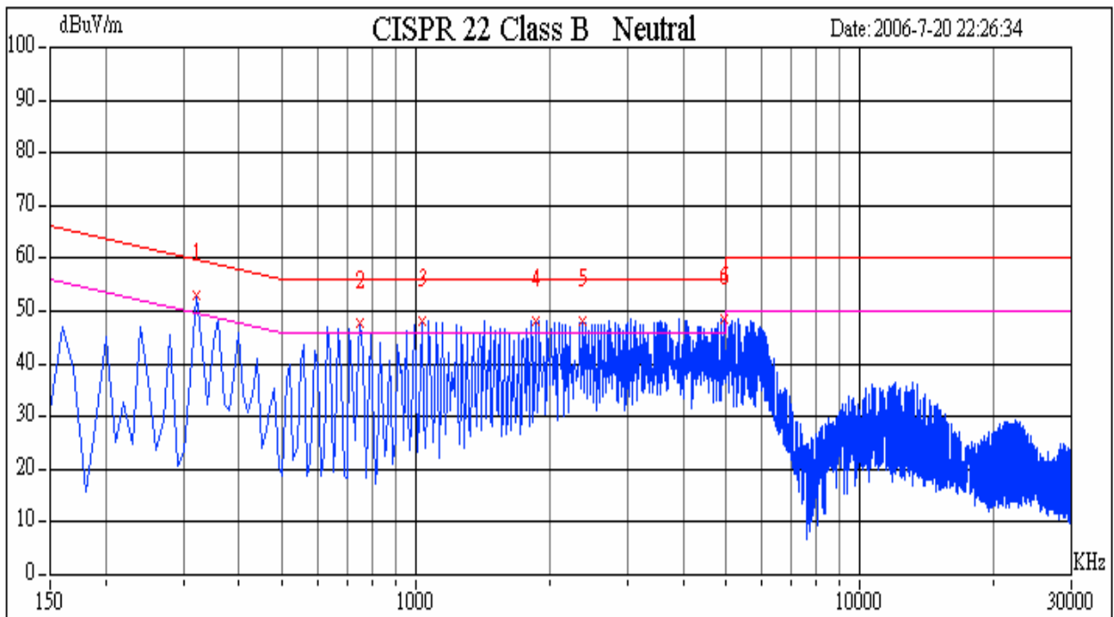
Conducted emissions (Line 2)
