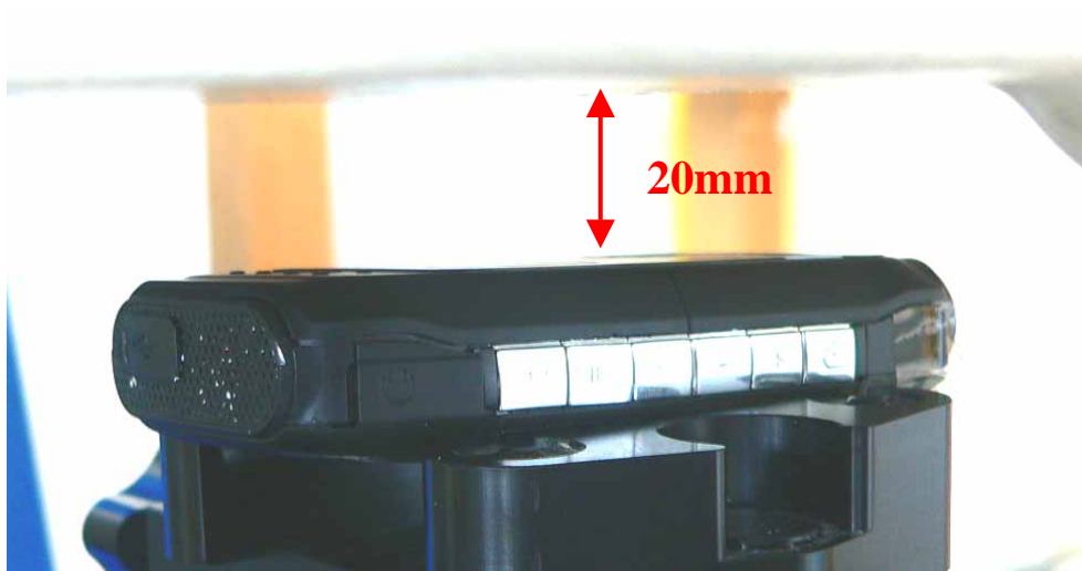
Fig. 21: Body worn configuration, GPRS (Class 10), antenna towards the phantom.
