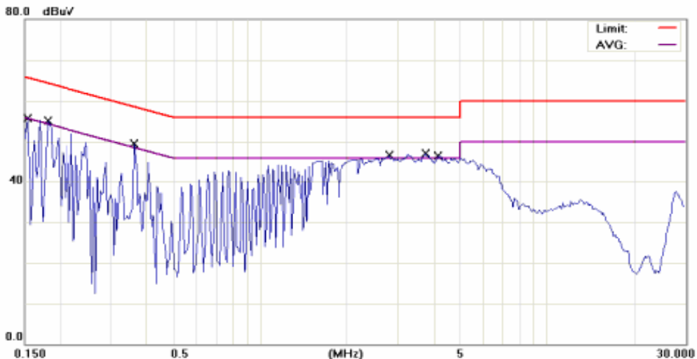
Conducted Emission Measurement
