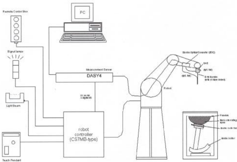
Fig. a SAR System Configuration
