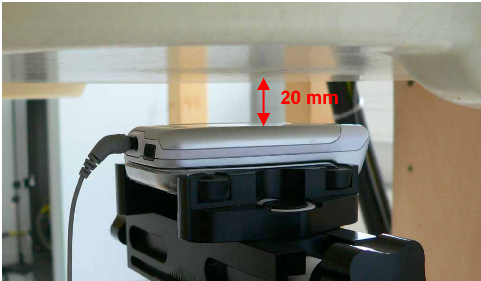
Fig. 24: Body worn configuration, GSM mode with headset, antenna towards the phantom.
