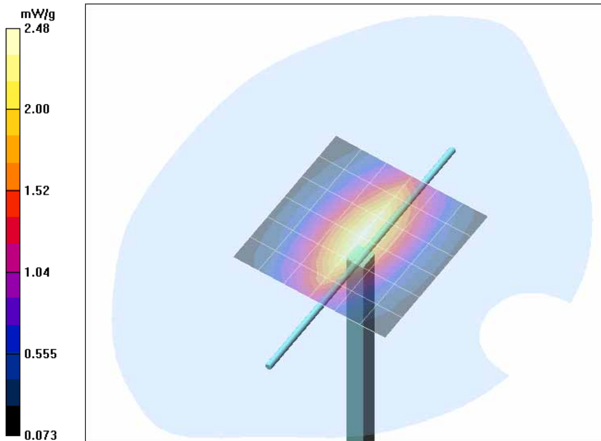
Fig. 12: Validation measurement 835 MHz Head (July 08, 2005), coarse grid. Ambient Temperature: 22.0° C, Liquid Temperature: 21.0° C.
