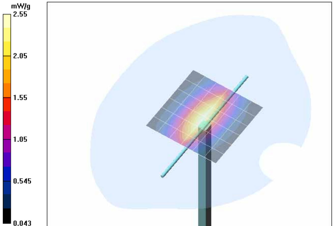
Fig. 13: Validation measurement 835 MHz Body (July 08, 2005), coarse grid. Ambient Temperature: 22.0° C, Liquid Temperature: 21.6° C.
