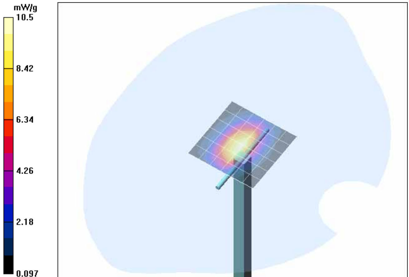
Fig. 14: Validation measurement 1900 MHz Head (July 11, 2005), coarse grid. Ambient Temperature: 22.0° C, Liquid Temperature: 21.5° C.
