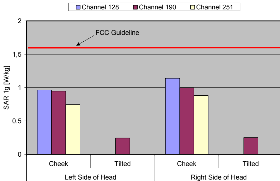
Fig. 8: The measured head phantom SAR values for the Alcatel OT-C652a for GSM 850 in comparison to the FCC exposure limit.
