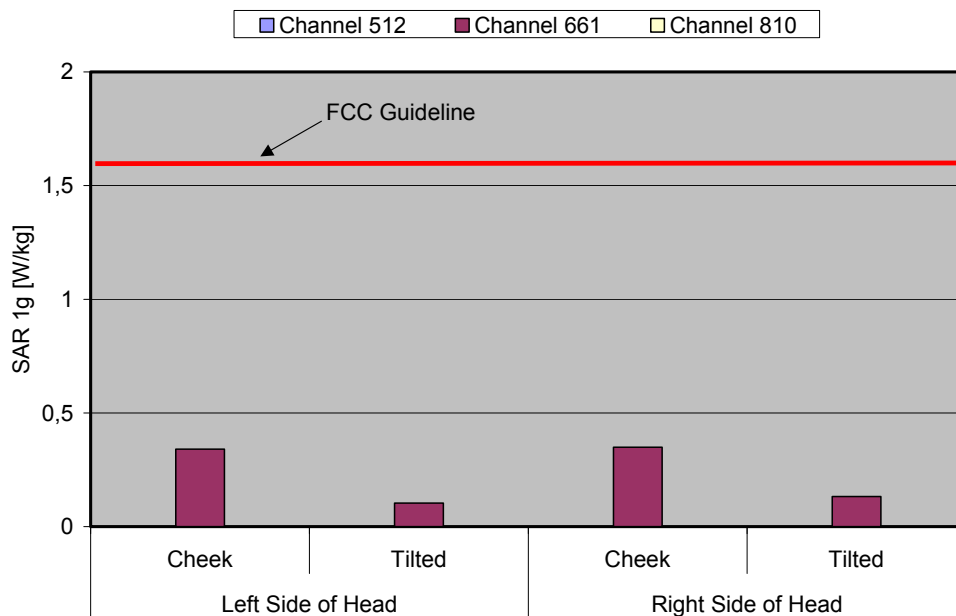
Fig. 9: The measured head phantom SAR values for the Alcatel OT-C652a for PCS 1900 in comparison to the FCC exposure limit.
