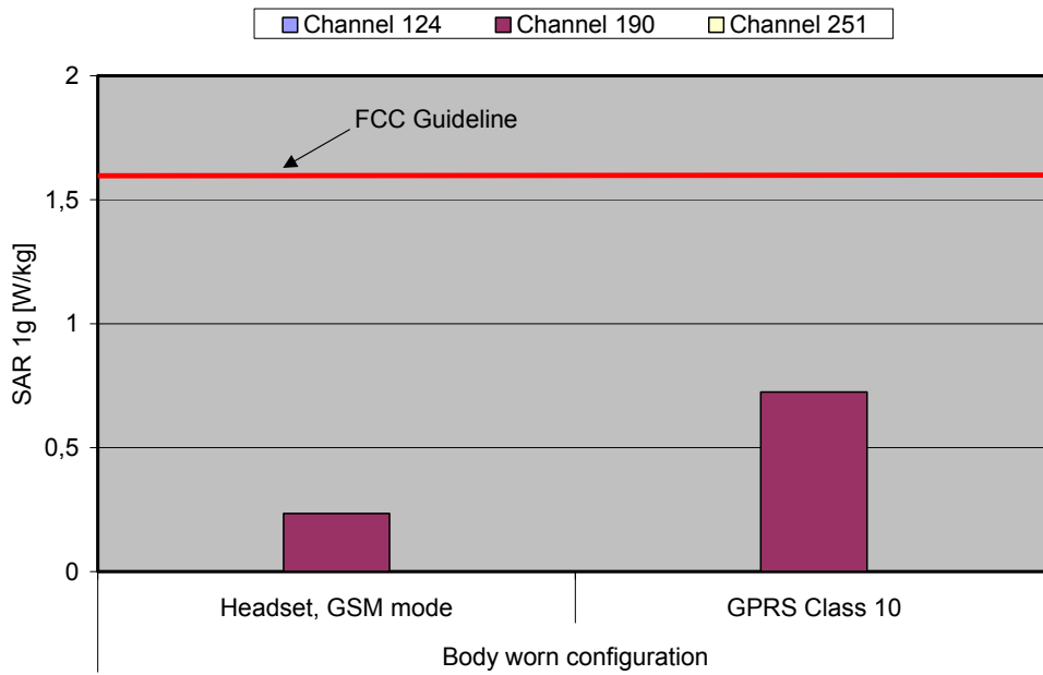
Fig. 10: The measured SAR values in body-worn configuration for the Alcatel OT-C652a for GSM 850 in comparison to the FCC exposure limit.
