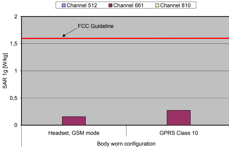
Fig. 11: The measured SAR values in body-worn configuration for the Alcatel OT-C652a for PCS 1900 in comparison to the FCC exposure limit.
