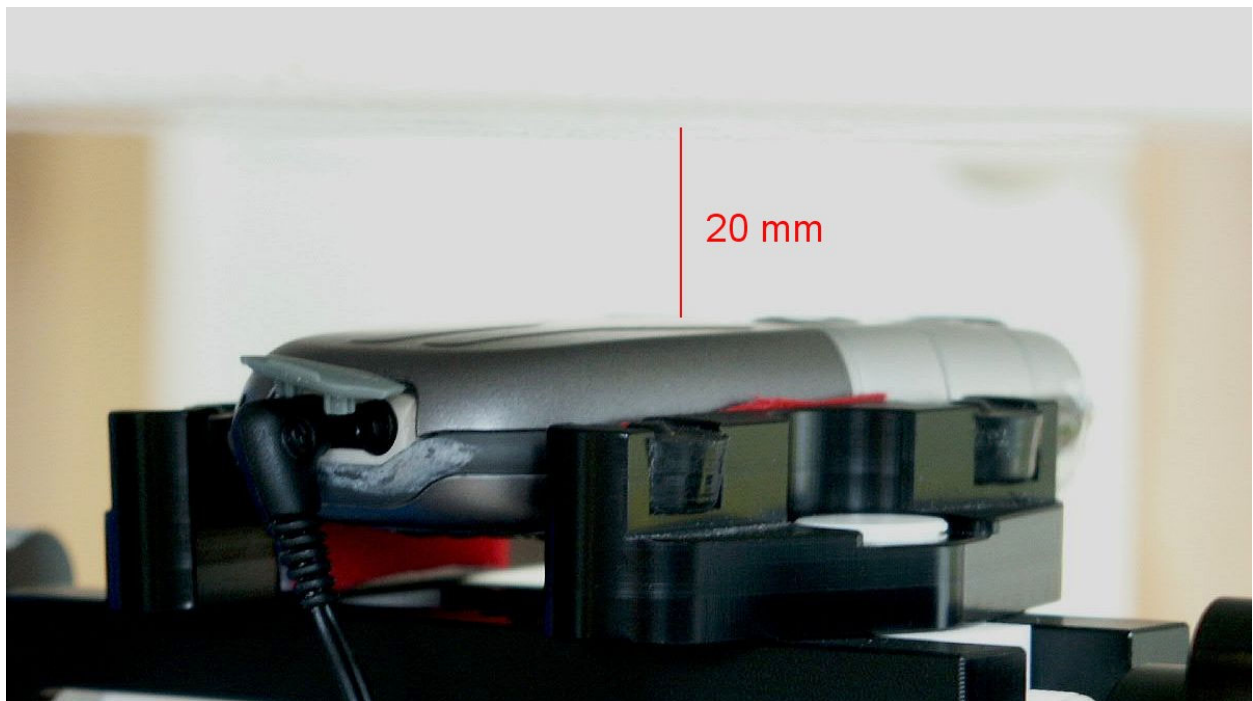
Fig. 18: Body worn configuration, GSM mode (1 TX slot) with headset, antenna towards the phantom.
