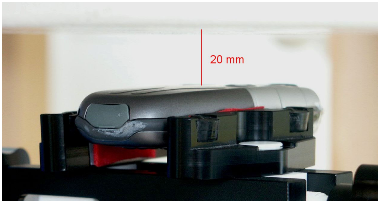
Fig. 17: Body worn configuration, GPRS mode (2 TX slots), antenna towards the phantom.
