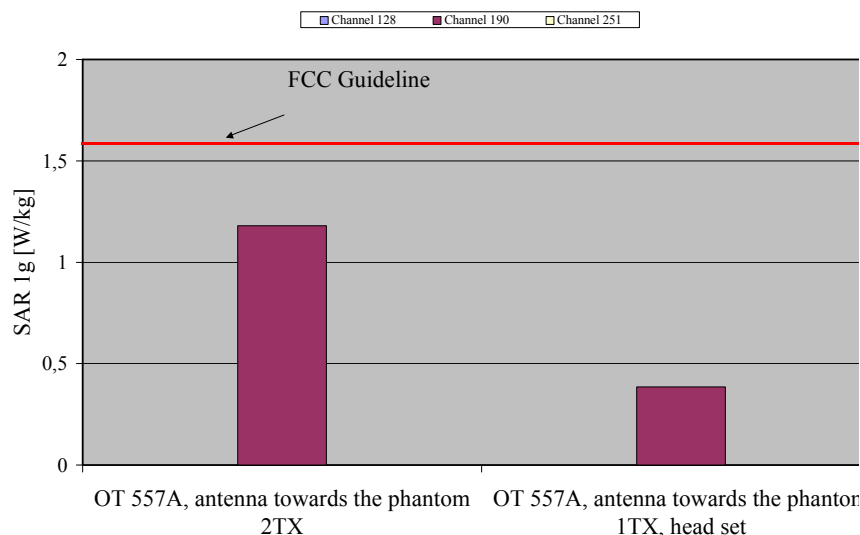
Fig. 10: The measured SAR values in body-worn configuration for the Alcatel One Touch 557A for GSM 850 (1 TX and 2 TX slots, gap = 20 mm) in comparison to the FCC exposure limit.
