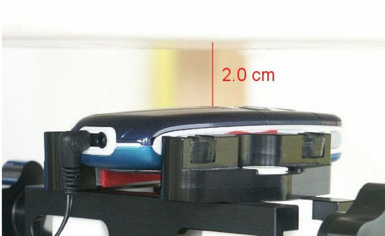
Fig. 25: Body worn configuration, GSM mode (1 TX slot) with headset, antenna towards the phantom.
