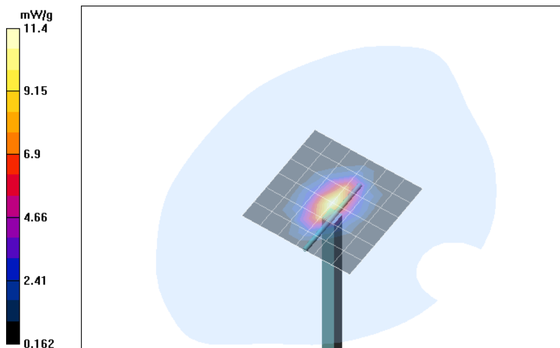
Fig. 10: Validation measurement 1900 MHz Head (April 21, 2004), coarse grid. Ambient Temperature: 22.0° C, Liquid Temperature: 20.6 C.
