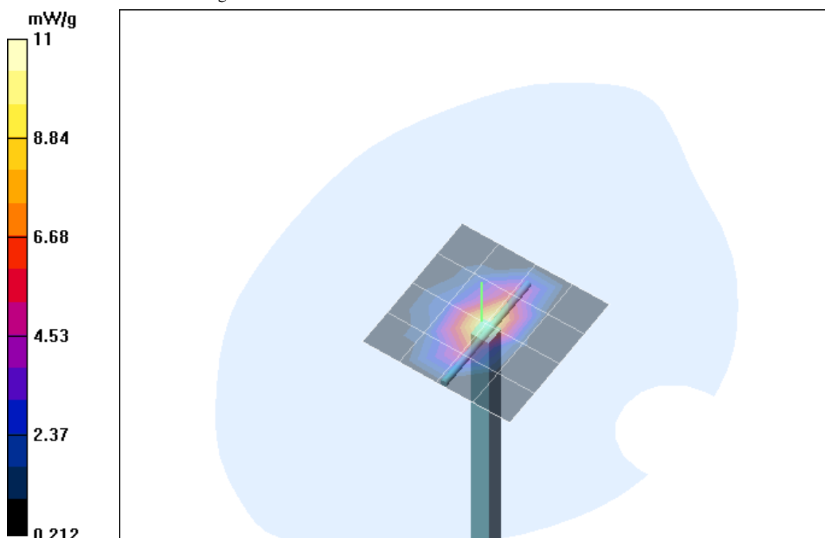
Fig. 16: Validation measurement 1900 MHz Head (October 09, 2003), coarse grid. Ambient Temperature: 20.8° C, Liquid Temperature: 20.4° C.
