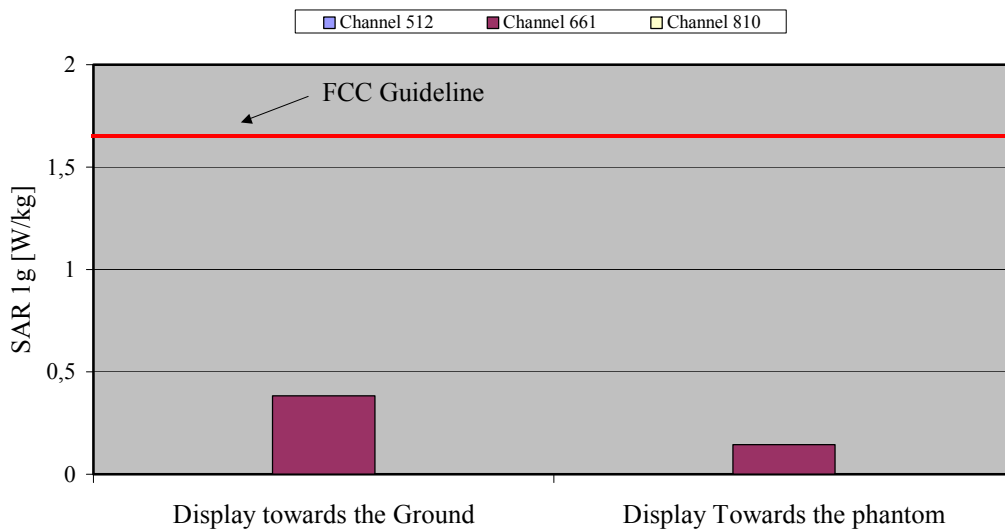
Fig. 9: The measured SAR values in body-worn configuration for the Alcatel One Touch 331P for PCS 1900, with belt clip and headset, in comparison to the FCC exposure limit.
