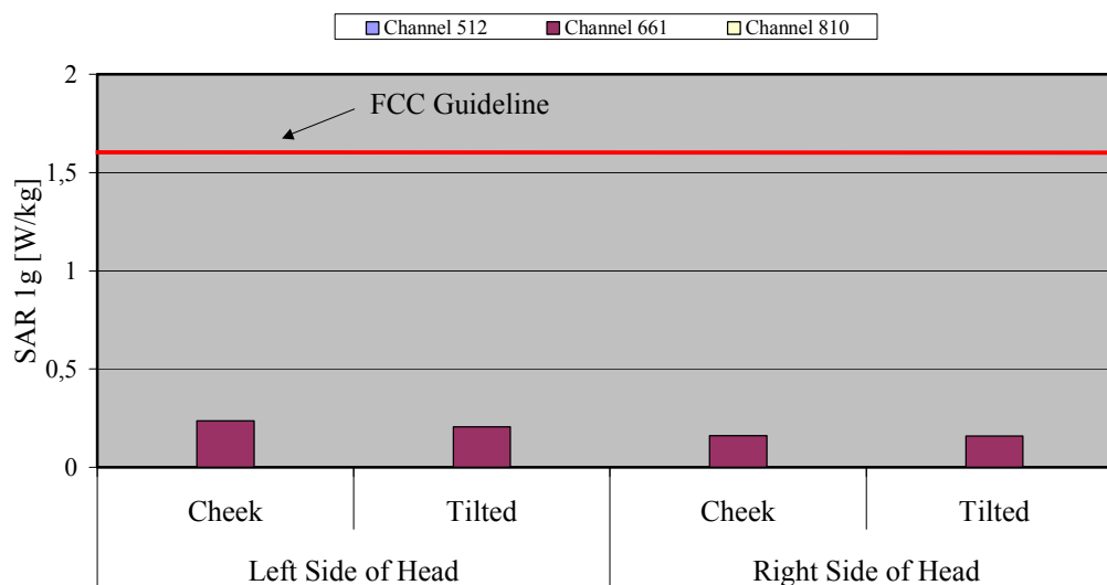
Fig. 8: The measured head phantom SAR values for the Alcatel One Touch 331P for PCS 1900 in comparison to the FCC exposure limit.
