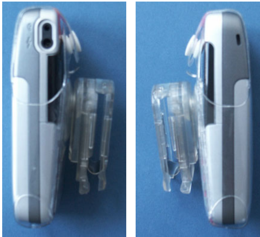
Fig. 18: Phone with used belt clip which dictates the closest distance to the body.
