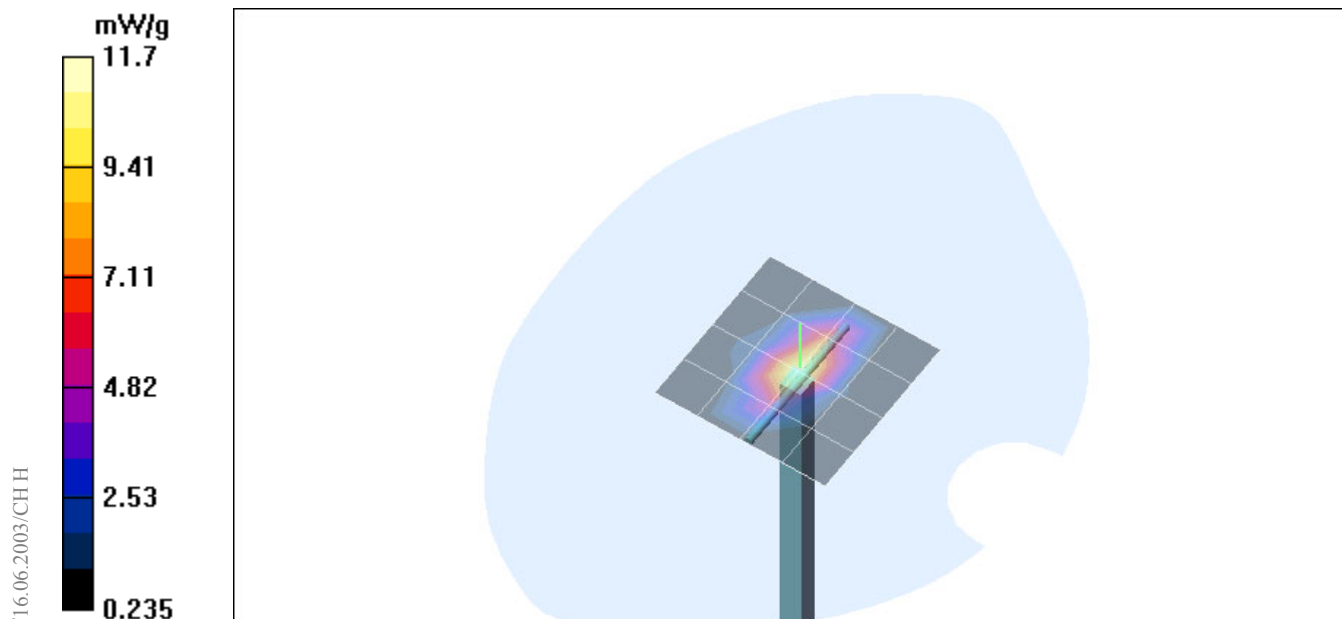
Fig. 12: Validation measurement 1900 MHz body (26.06.2003), coarse grid. Ambient Temperature: 21.0° C, Liquid Temperature: 20.5° C.
