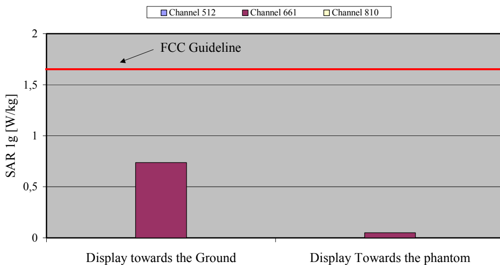
Fig. 10: The measured SAR values in body-worn configuration for the Alcatel One Touch 331P for PCS 1900 , with 1.5 cm distance between mobile and phantom, in comparison to the FCC exposure limit.
