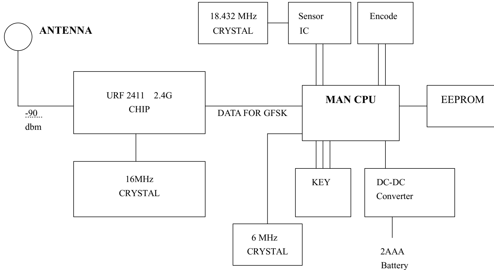
WIRELESS MOUSE (TX) BLOCK DIAGRAM
