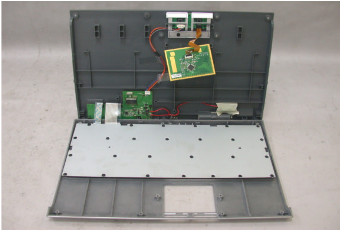
EUT MAIN BOARD VIEW
