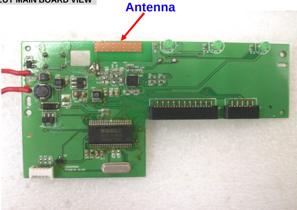
EUT MAIN BOARD VIEW
