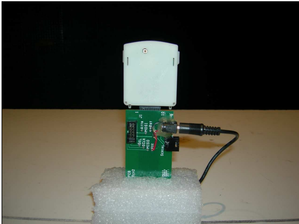
Figure 1: Radiated Emissions
