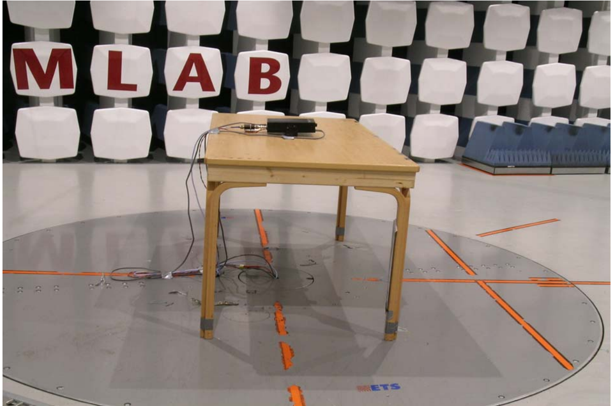
Radiated emission Measurements
