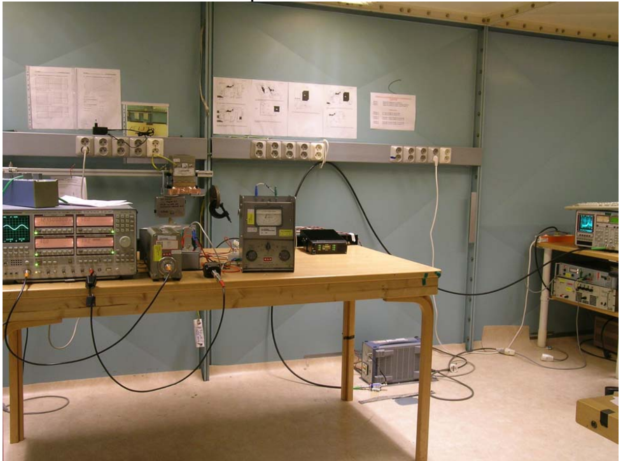
Test set-up for Conducted emission – On DC supply
