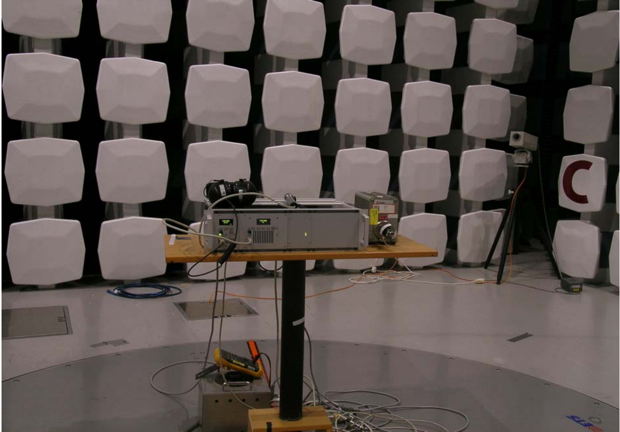
Radiated spurious measurements for both TX & RX
