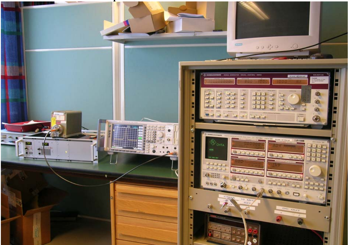
Test set-up for conducted measurements
