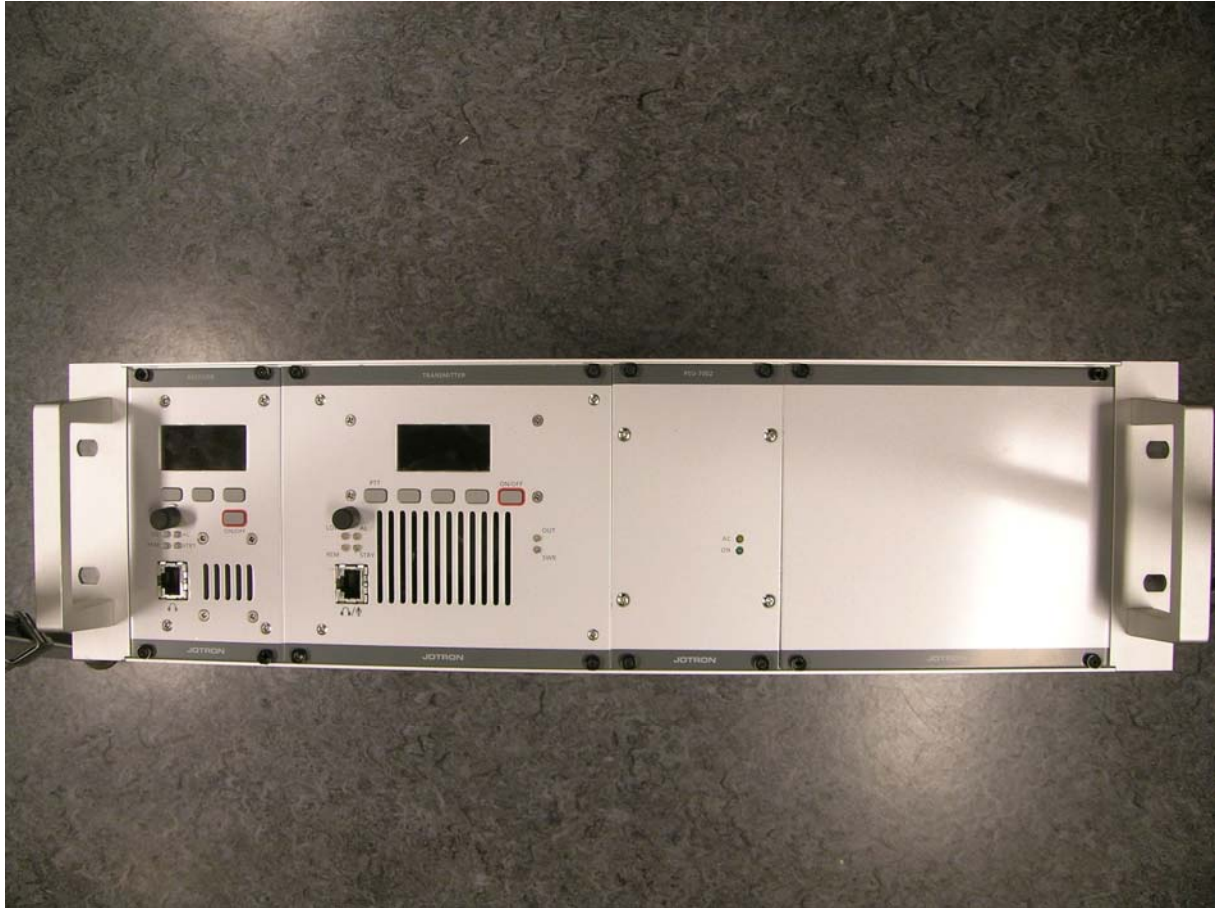
Transmitter/receiver with rack – Front view
