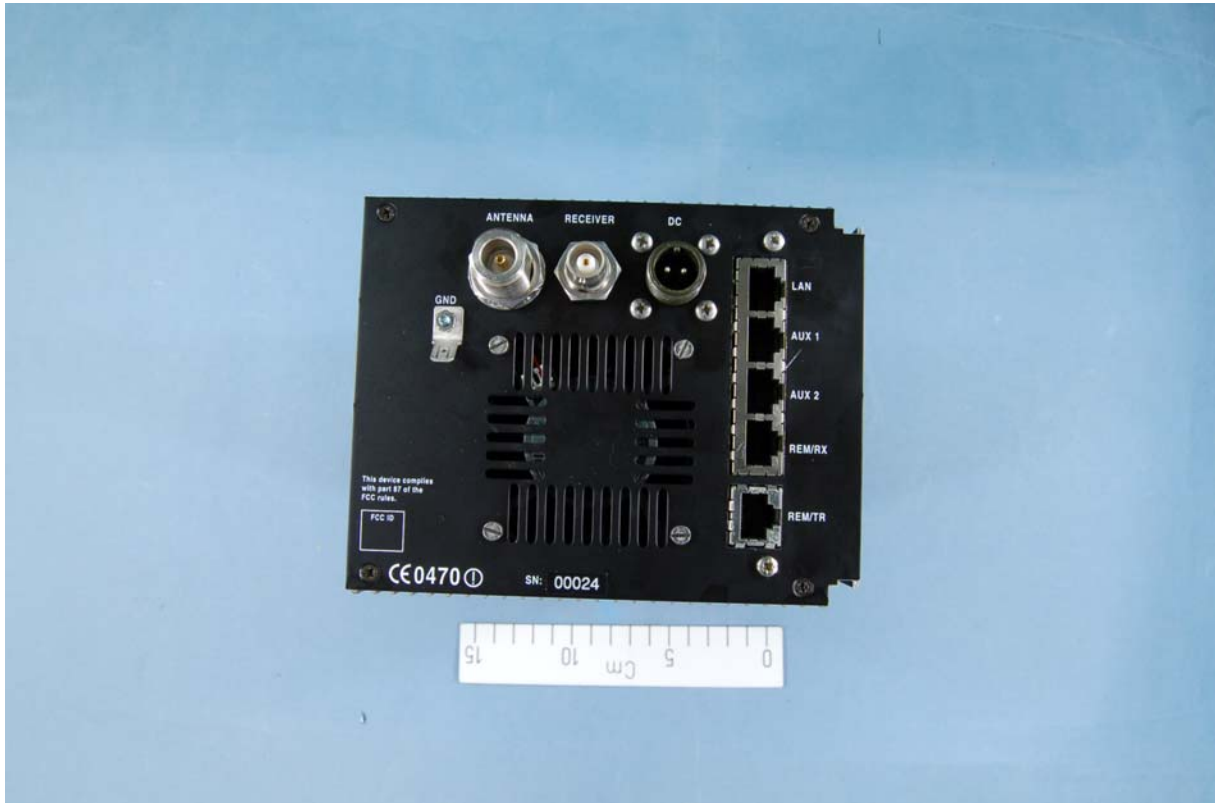
TA7625 Transmitter – Rear View
