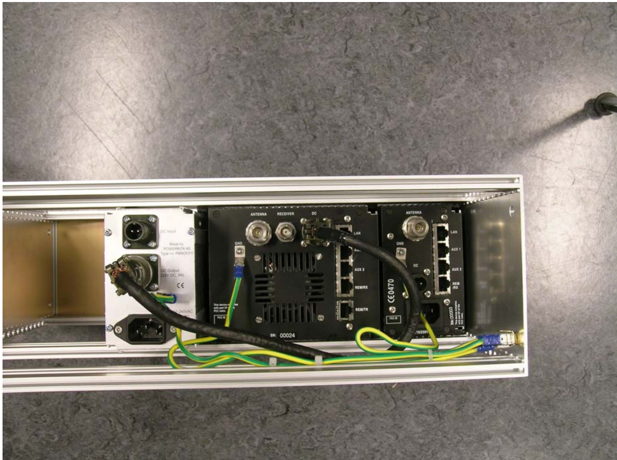
Transmitter/receiver with rack – Rear view
