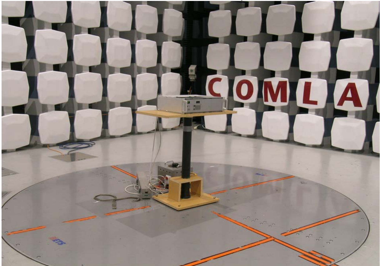
Test set-up for Radiated emission 50 ohm termination
