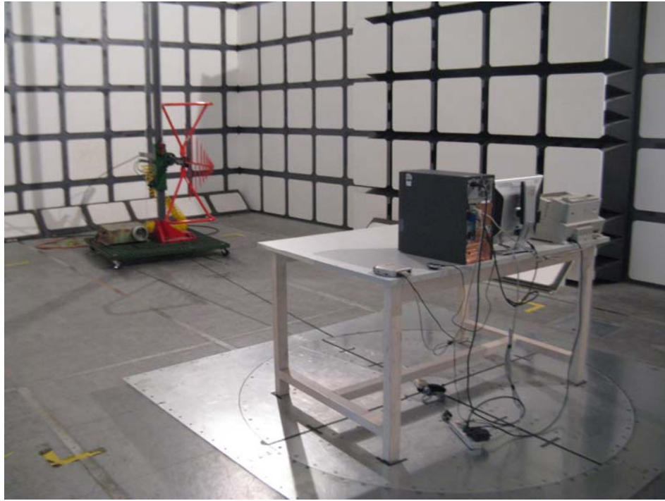
Radiated Emissions - Front View (Charging with PC)
