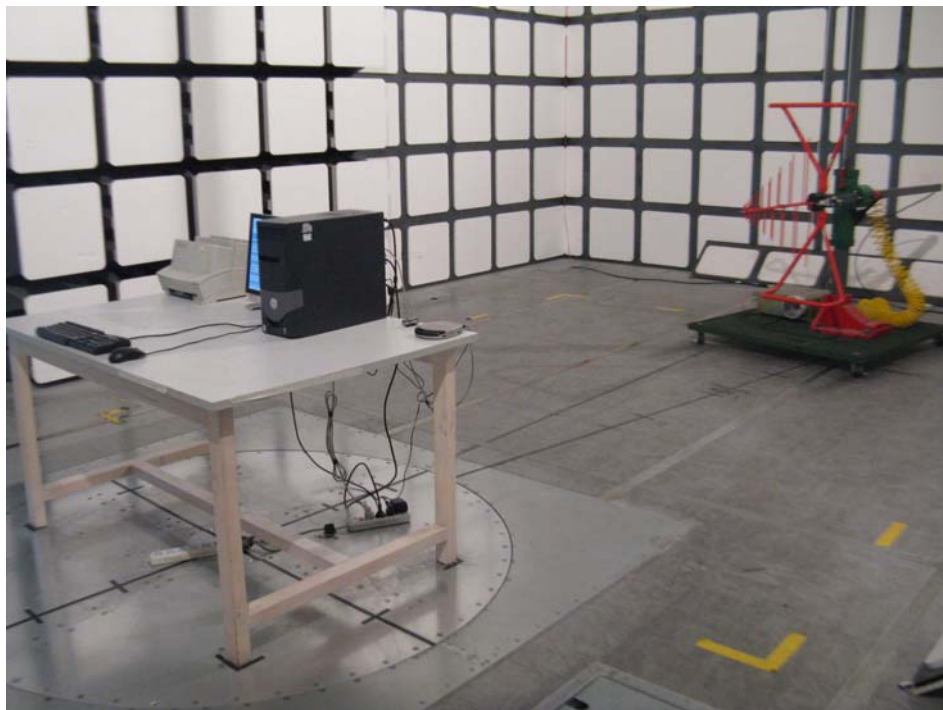
Radiated Emissions - Rear View (Charging with PC)
