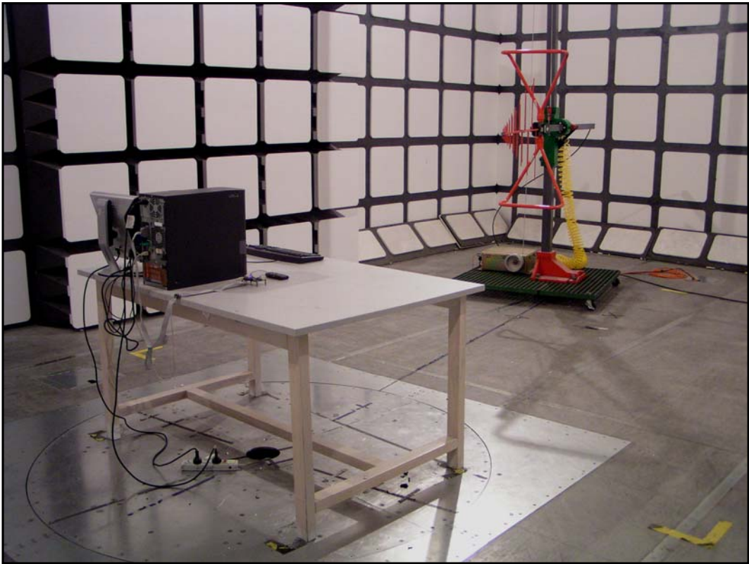
Radiated Emissions - Rear View (Below 1 GHz) for transmitting mode
