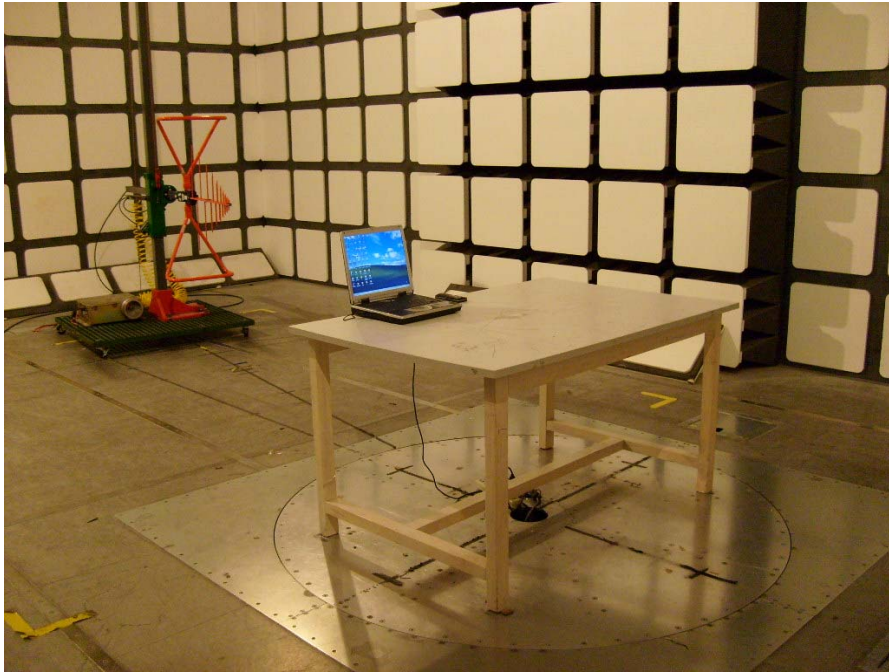
Radiated Emissions - Rear View (USB Charging)
