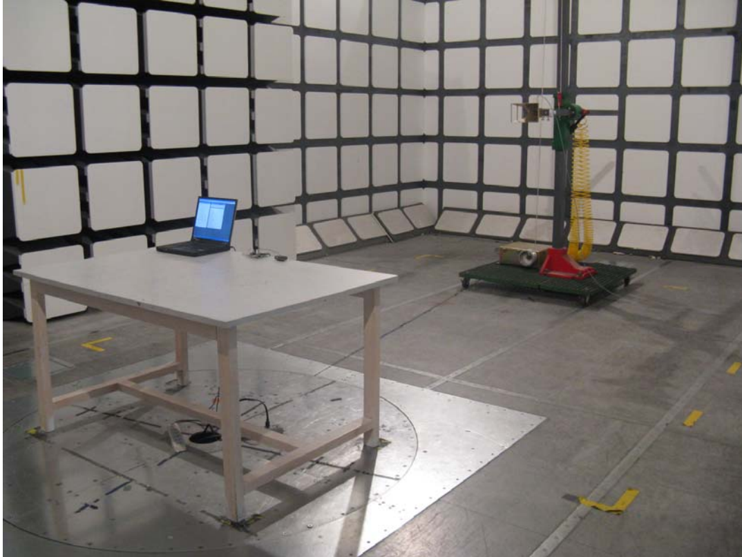
Radiated Emissions - Front View (Above 1 GHz)
