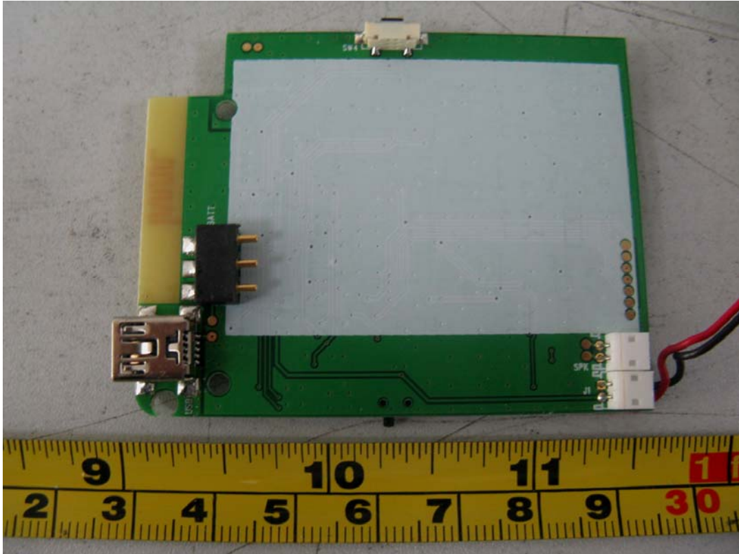
EUT- Main Board Components Bottom View
