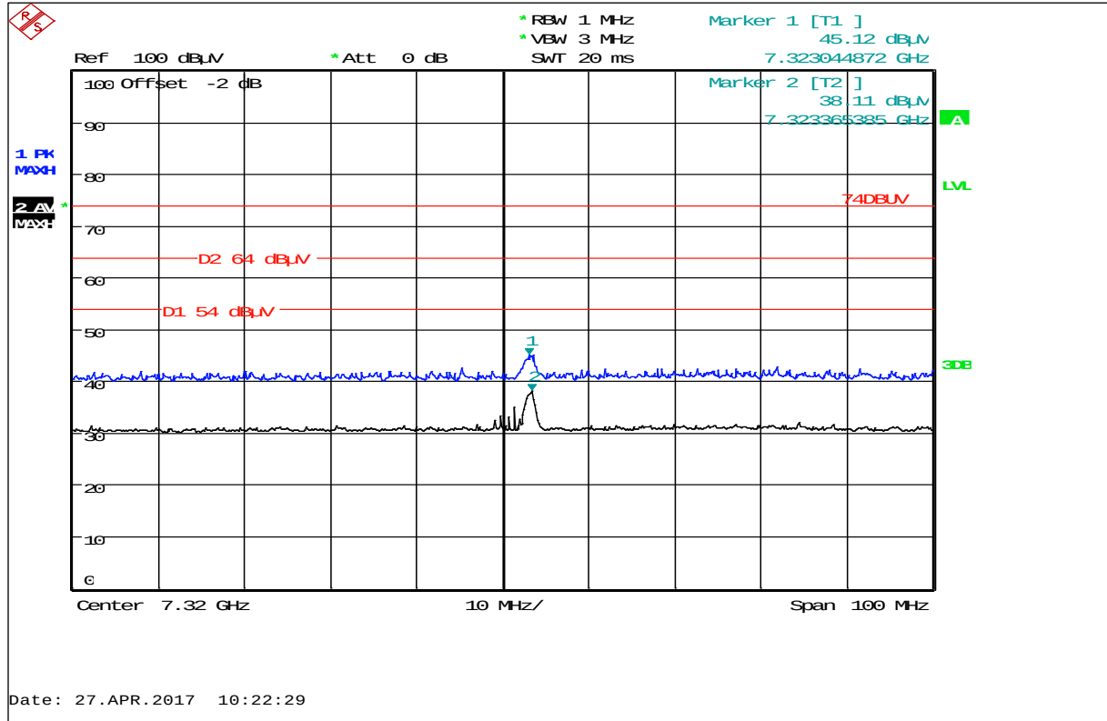
Plot 35: Harmonic 7.32 GHz, LB 565-02 (DC powered) with Tank sensor, horizontal / vertical polarization
