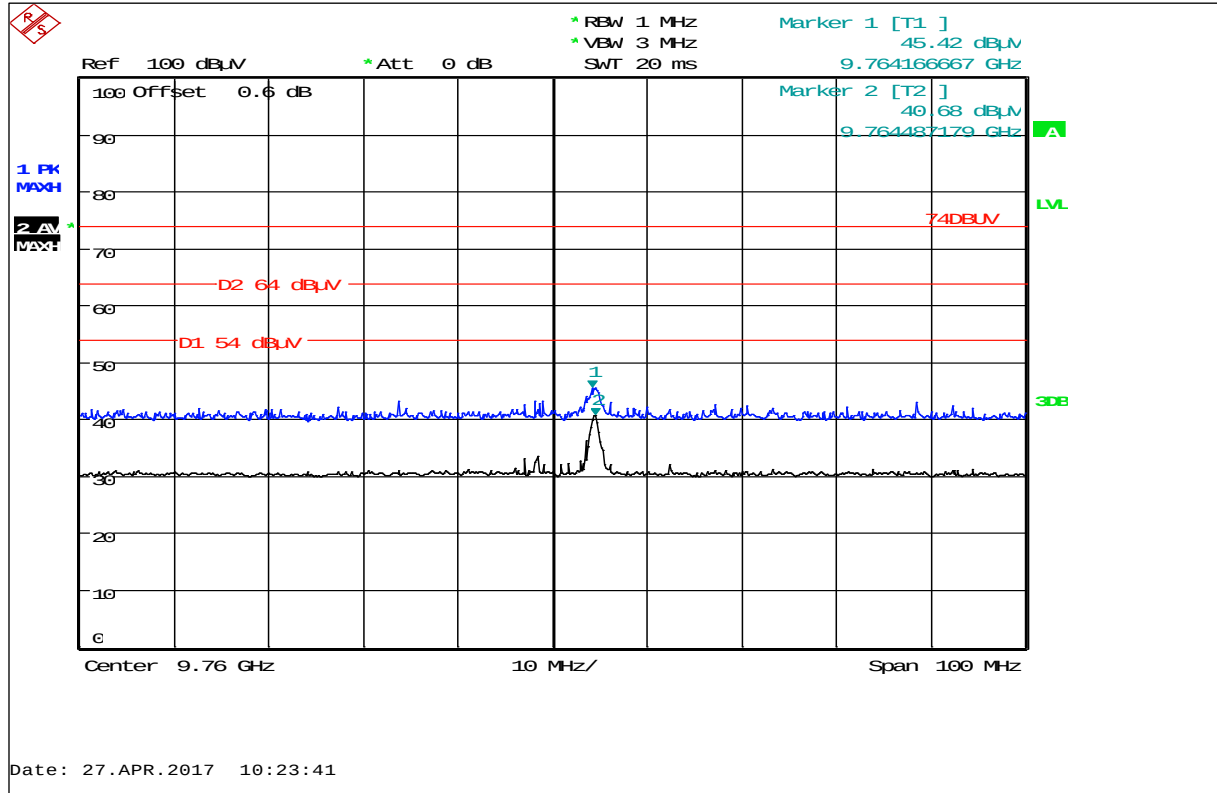
Plot 39: Harmonic 9.76 GHz, LB 565-02 (DC powered) with Tank sensor, horizontal / vertical polarization
