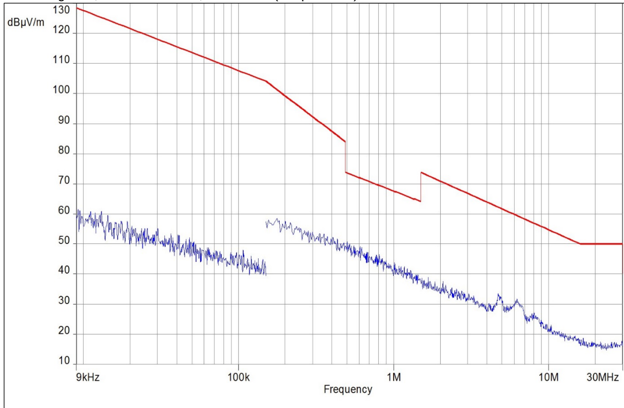
Plot 9: TX Magnetic, 9 kHz – 30 MHz, LB 565-01 (AC powered) with Tank sensor
