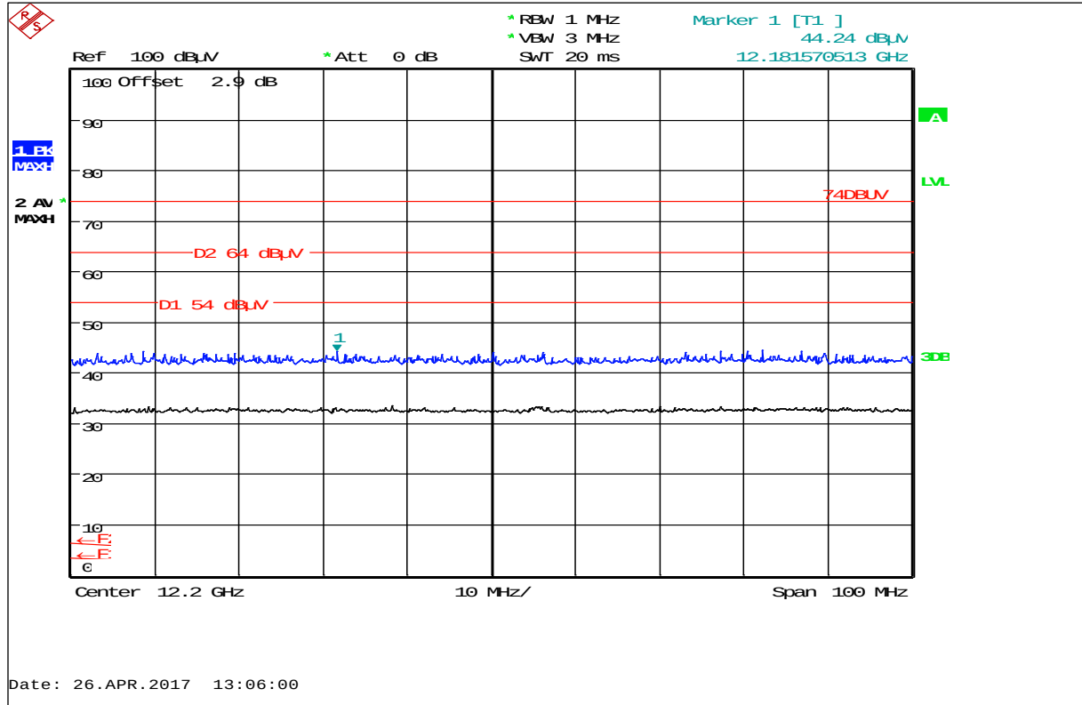
Plot 41: Harmonic 12.2 GHz, LB 565-01 (AC powered) with Tank sensor, horizontal / vertical polarization
