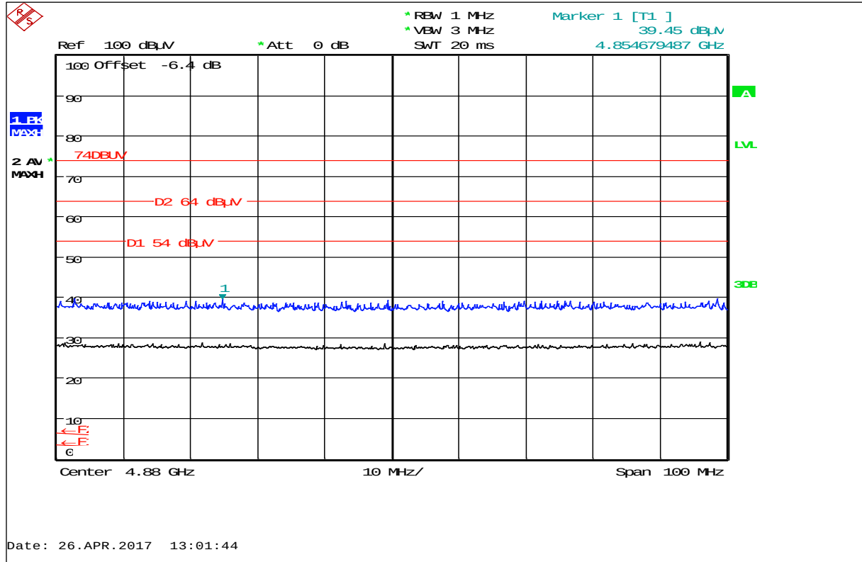
Plot 29: Harmonic 4.88 GHz, LB 565-01 (AC powered) with Tank sensor, horizontal / vertical polarization
