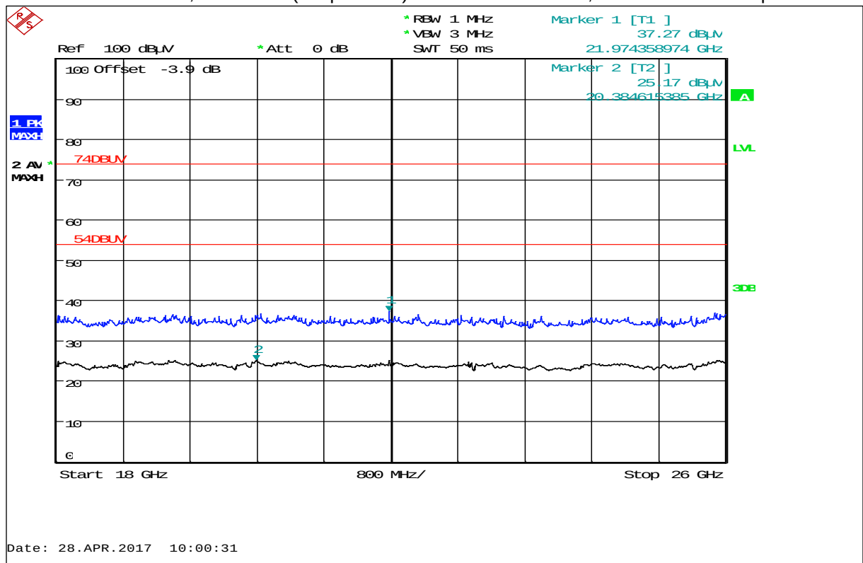
Plot 26: 18 GHz to 26 GHz, LB 565-01 (AC powered) with Flow cell sensor, horizontal / vertical polarization
