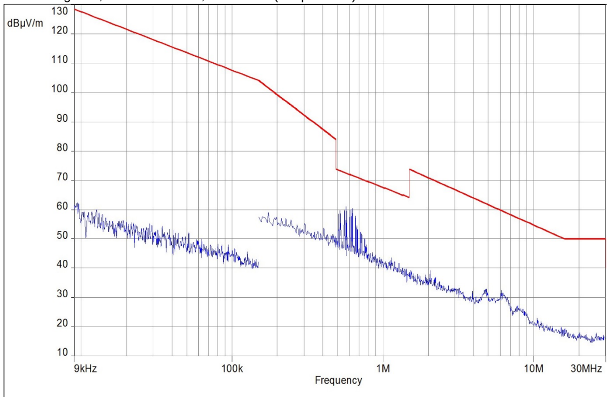
Plot 12: TX Magnetic, 9 kHz – 30 MHz, LB 565-02 (DC powered) with Flow cell sensor
