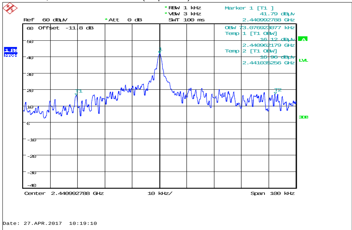
Plot 7: 99% OBW, MicroPolar Brix LB 565-02 (DC powered) with Tank sensor
