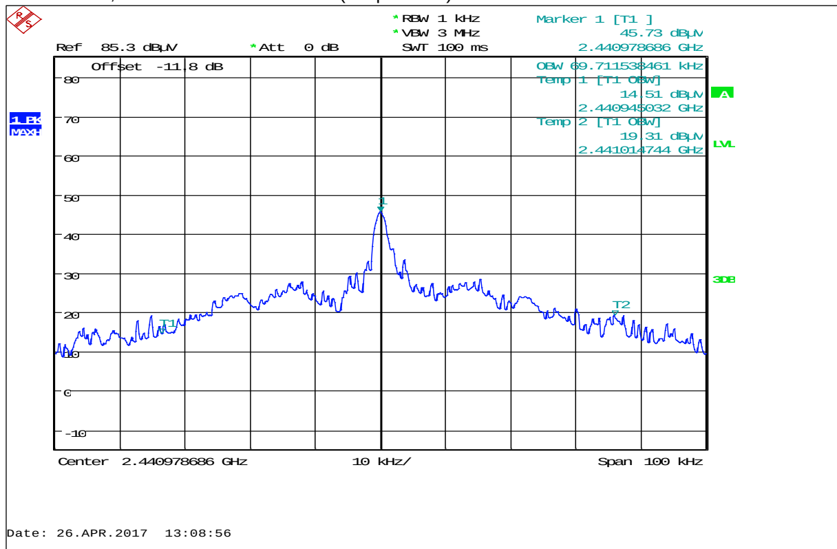
Plot 5: 99% OBW, MicroPolar Brix LB 565-01 (AC powered) with Tank sensor
