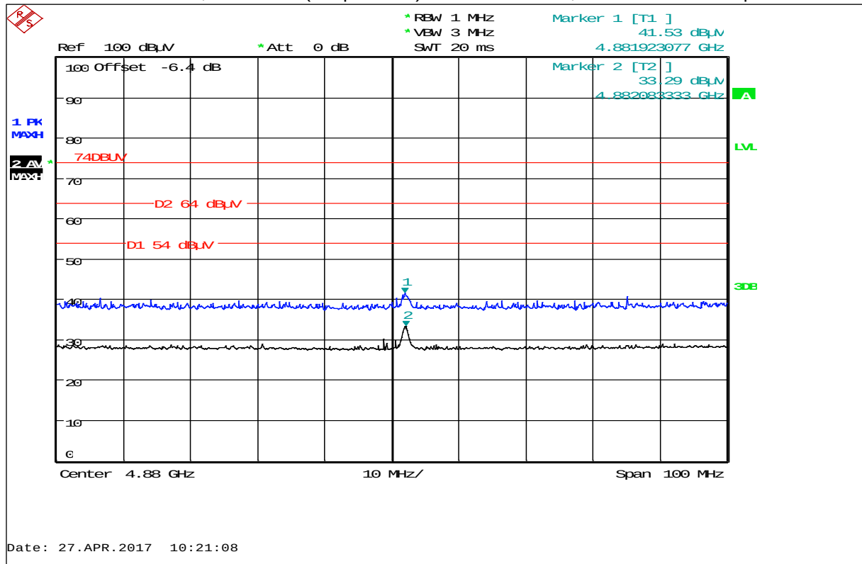
Plot 31: Harmonic 4.88 GHz, LB 565-02 (DC powered) with Tank sensor, horizontal / vertical polarization
