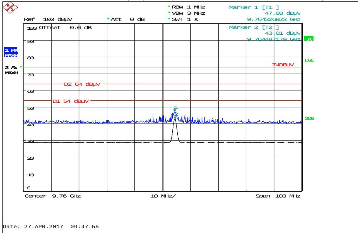
Plot 40: Harmonic 9.76 GHz, LB 565-02 (DC powered) with Flow cell sensor, horizontal / vertical polarization
