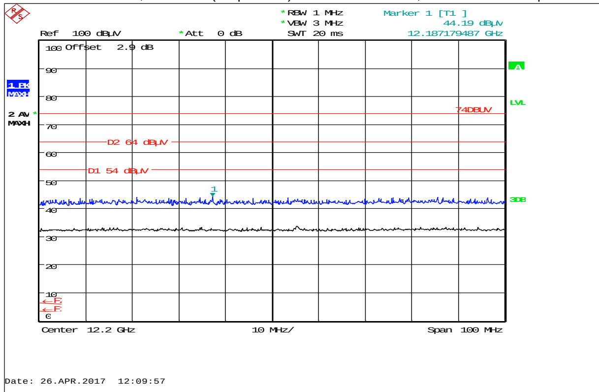
Plot 42: Harmonic 12.2 GHz, LB 565-01 (AC powered) with Flow cell sensor, horizontal / vertical polarization
