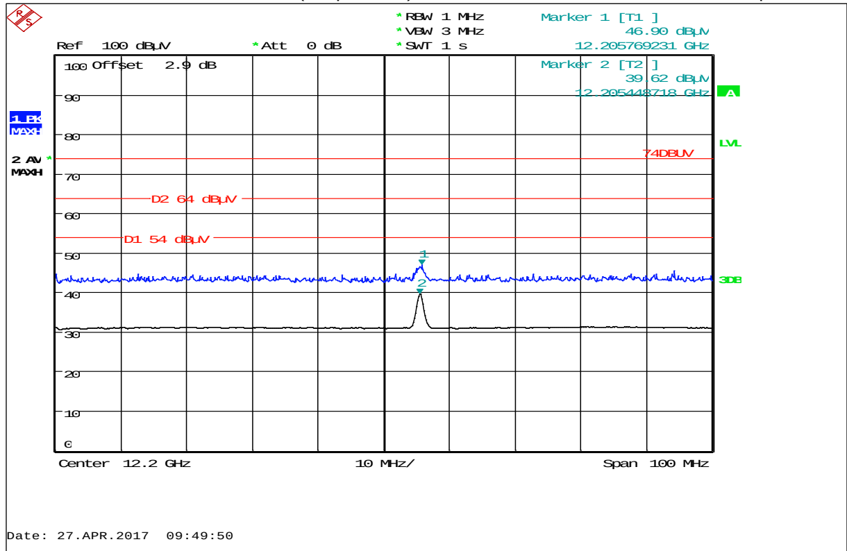
Plot 44: Harmonic 12.2 GHz, LB 565-02 (DC powered) with Flow cell sensor, horizontal / vertical polarization
