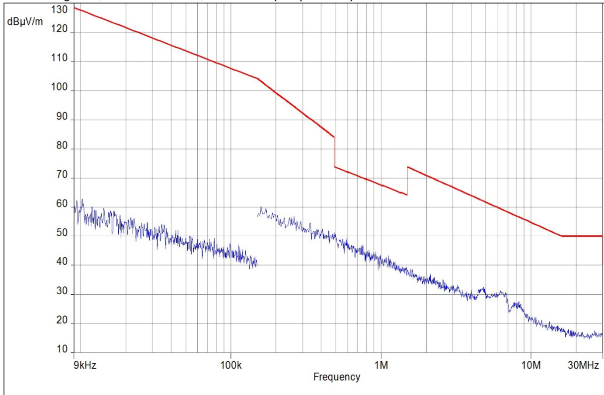
Plot 11: TX Magnetic, 9 kHz – 30 MHz, LB 565-02 (DC powered) with Tank sensor
