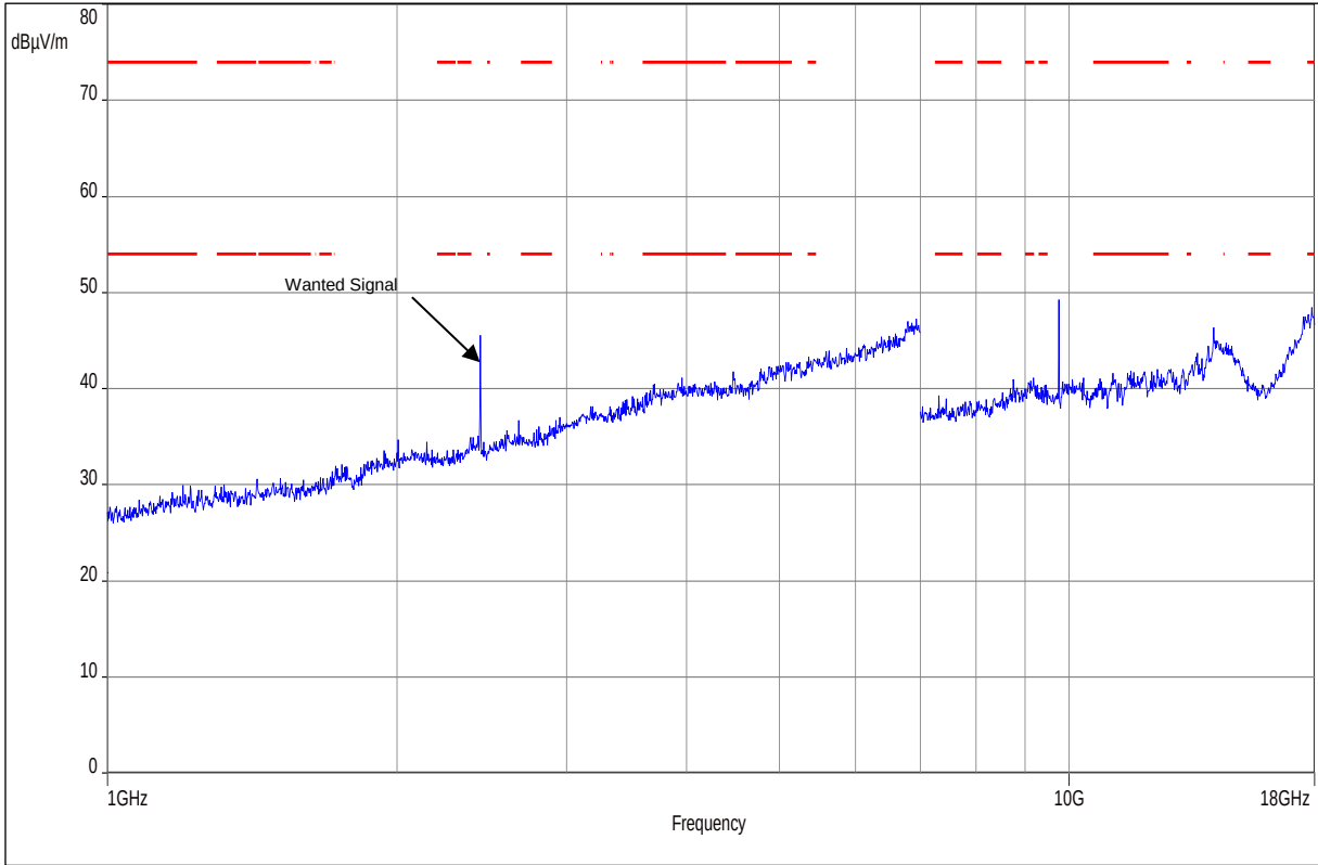
Plot 17: 1 GHz to 18 GHz, LB 565-01 (AC powered) with Tank sensor, horizontal / vertical polarization
