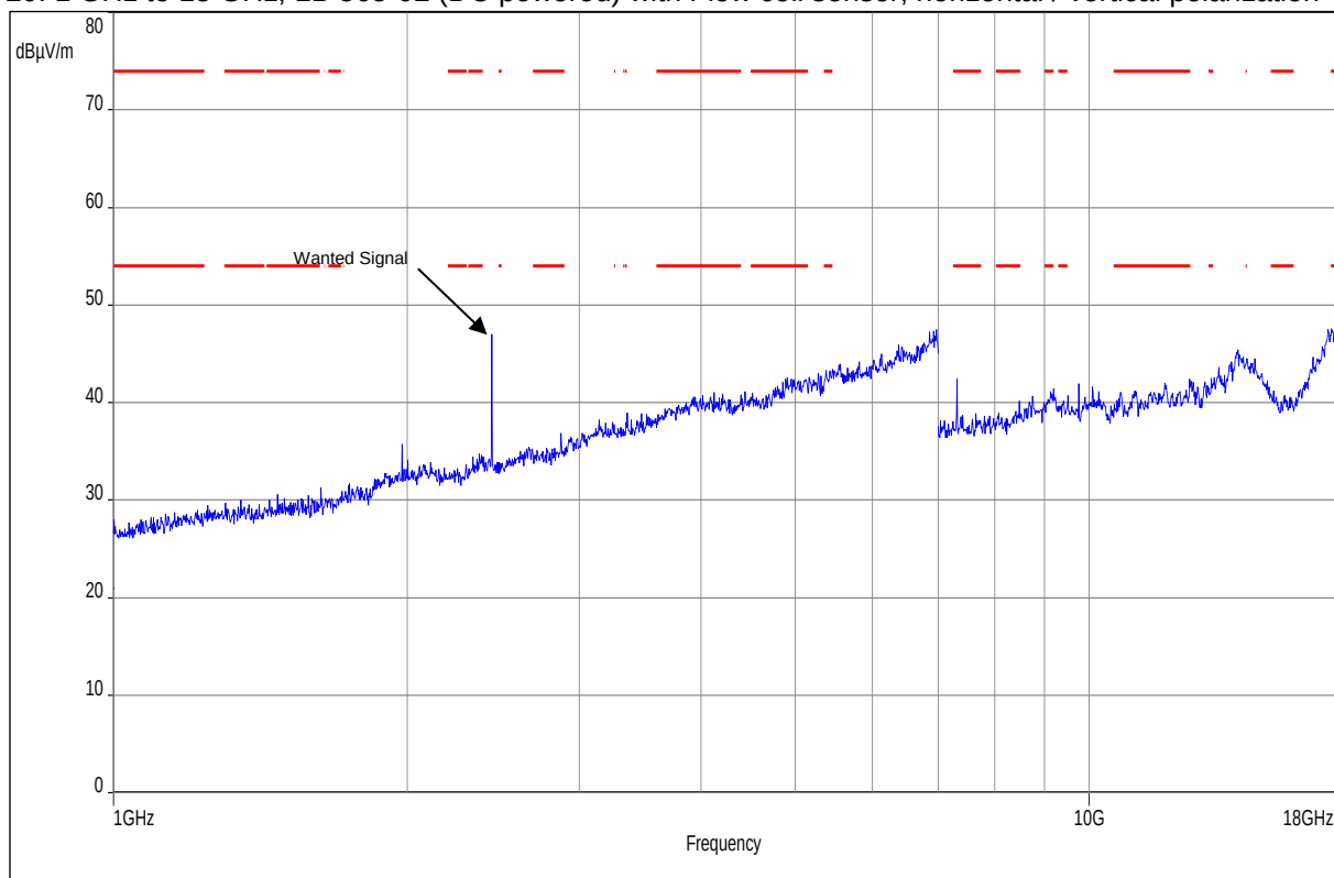
Plot 20: 1 GHz to 18 GHz, LB 565-02 (DC powered) with Flow cell sensor, horizontal / vertical polarization
