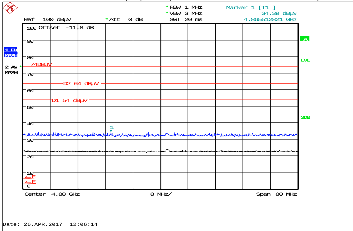
Plot 30: Harmonic 4.88 GHz, LB 565-01 (AC powered) with Flow cell sensor, horizontal / vertical polarization
