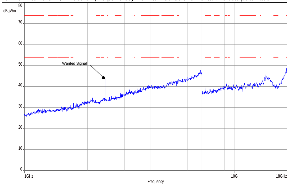
Plot 19: 1 GHz to 18 GHz, LB 565-02 (DC powered) with Tank sensor, horizontal / vertical polarization
