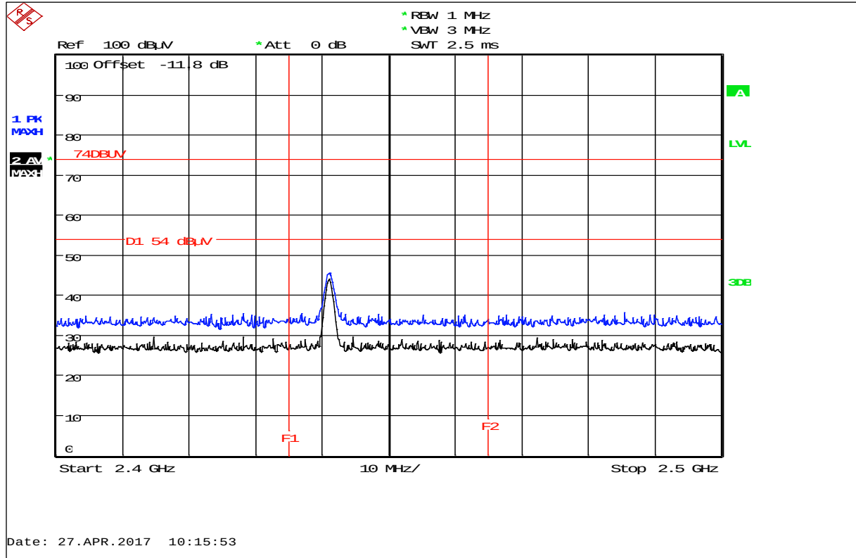
Plot 23: BEC, LB 565-02 (DC powered) with Tank sensor, horizontal / vertical polarization
