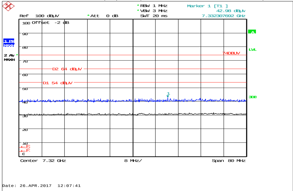
Plot 34: Harmonic 7.32 GHz, LB 565-01 (AC powered) with Flow cell sensor, horizontal / vertical polarization
