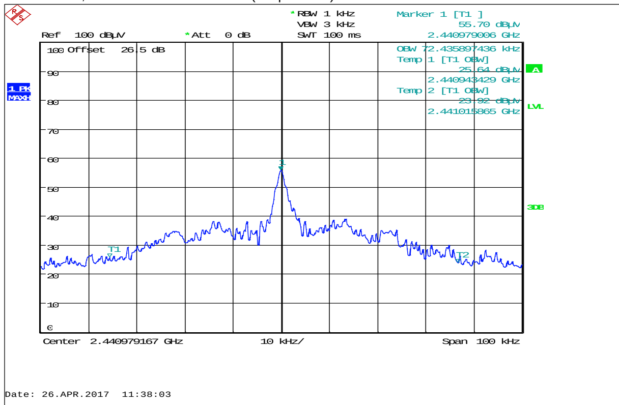
Plot 6: 99% OBW, MicroPolar Brix LB 565-01 (AC powered) with Flow cell sensor
