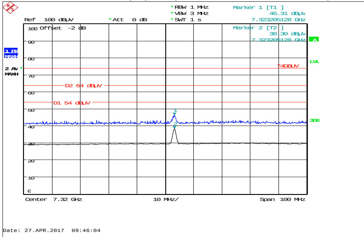
Plot 36: Harmonic 7.32 GHz, LB 565-02 (DC powered) with Flow cell sensor, horizontal / vertical polarization
