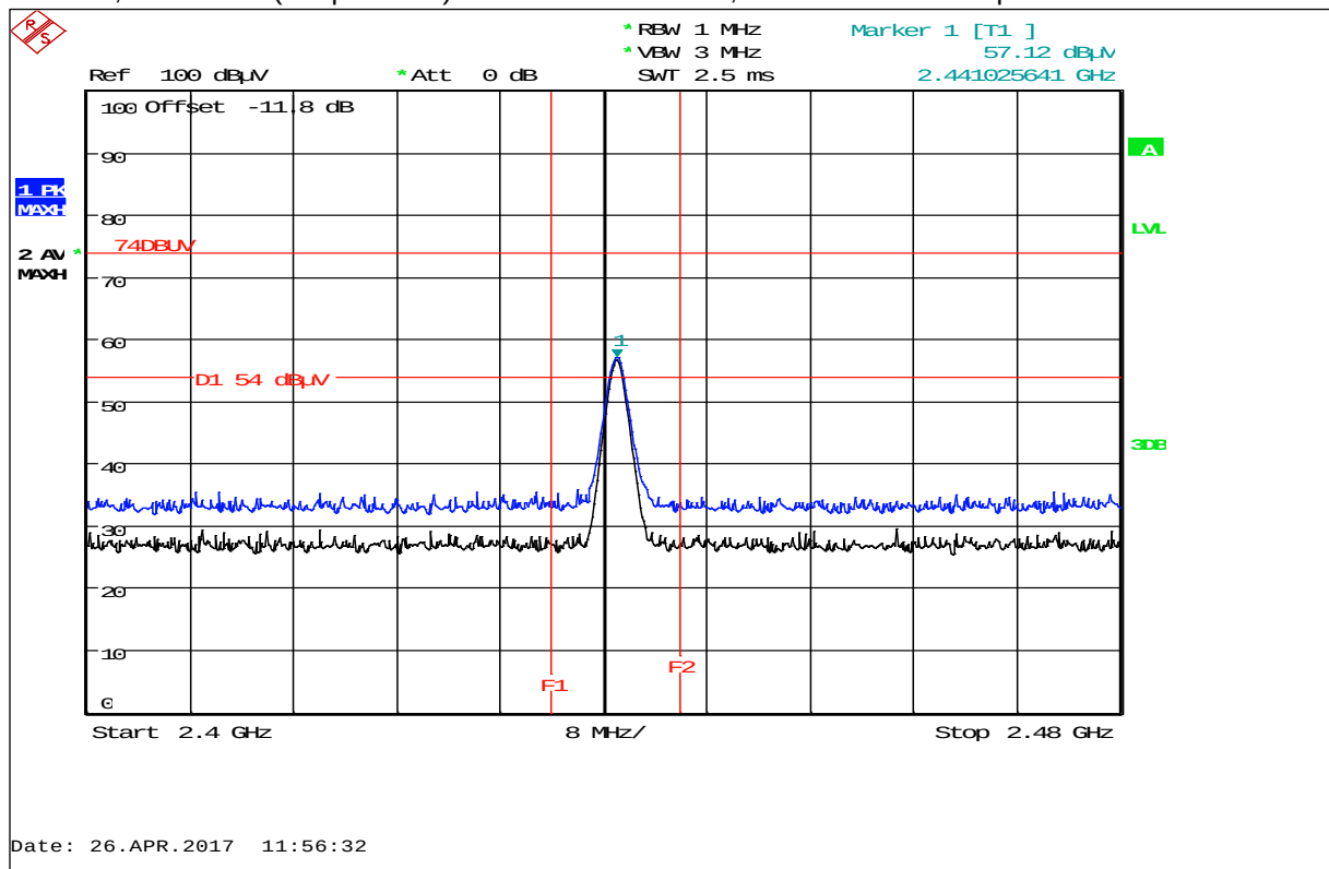
Plot 22: BEC, LB 565-01 (AC powered) with Flow cell sensor, horizontal / vertical polarization
