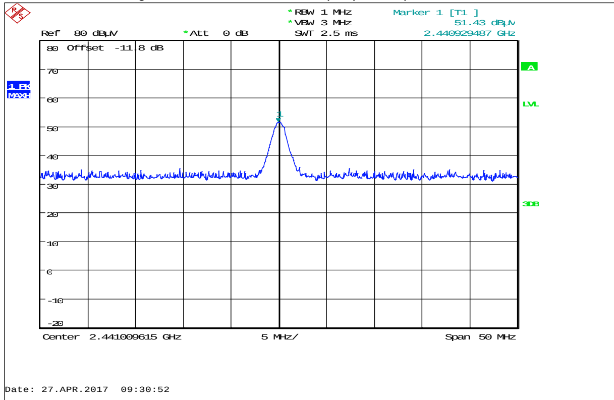
Plot 4: Maximum field strength, MicroPolar Brix LB 565-02 (DC powered) with Flow cell sensor
