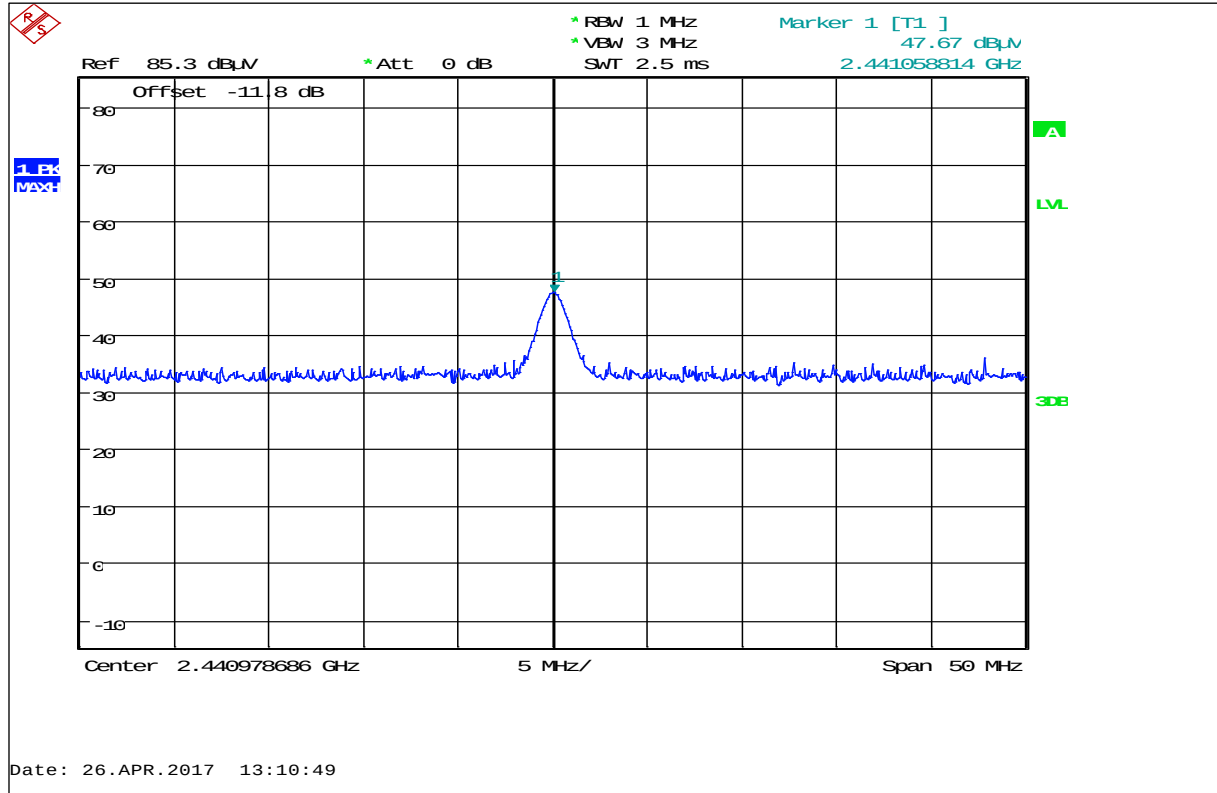
Plot 1: Maximum field strength, MicroPolar Brix LB 565-01 (AC powered) with Tank sensor
