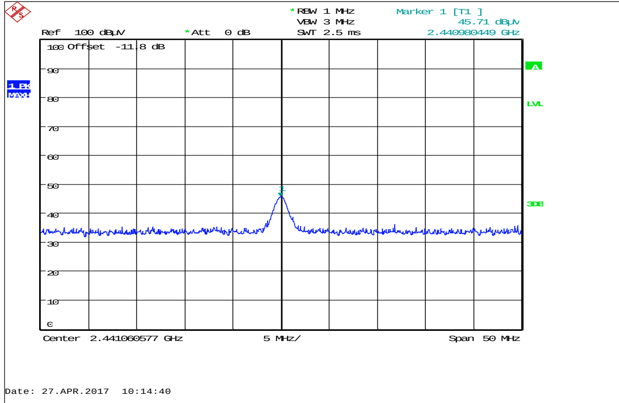
Plot 3: Maximum field strength, MicroPolar Brix LB 565-02 (DC powered) with Tank sensor
