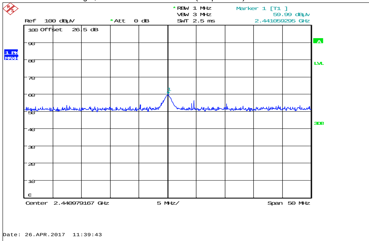
Plot 2: Maximum field strength, MicroPolar Brix LB 565-01 (AC powered) with Flow cell sensor
