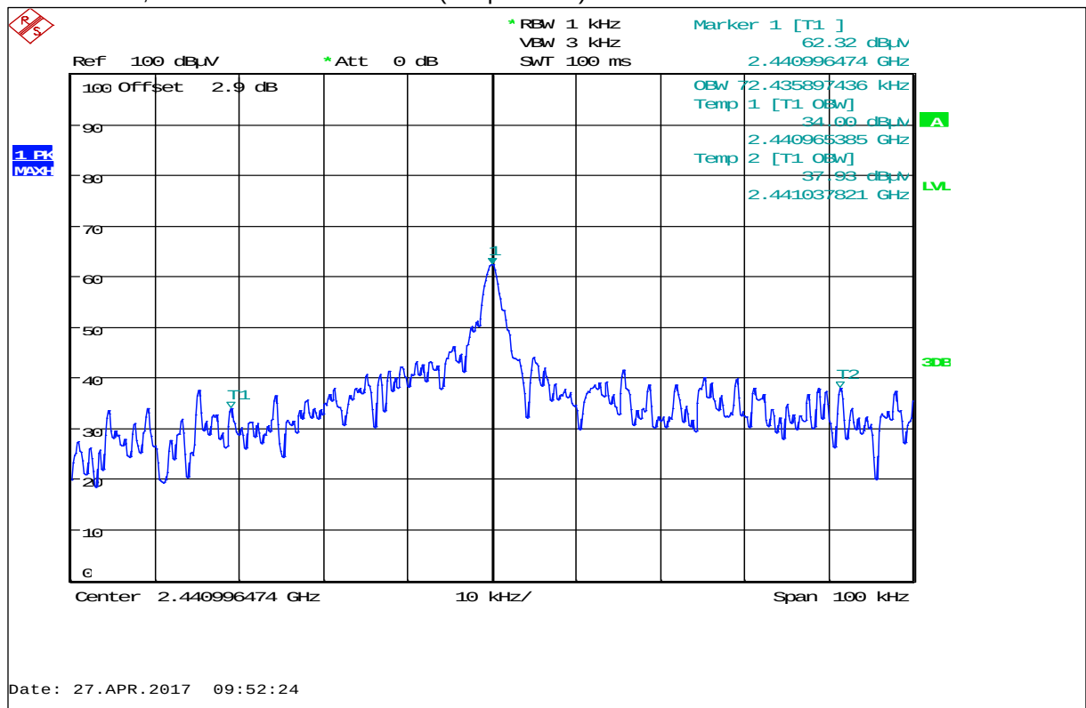
Plot 8: 99% OBW, MicroPolar Brix LB 565-02 (DC powered) with Flow cell sensor
