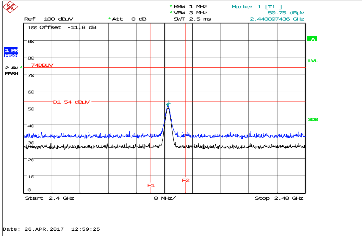
Plot 21: BEC, LB 565-01 (AC powered) with Tank sensor, horizontal / vertical polarization
