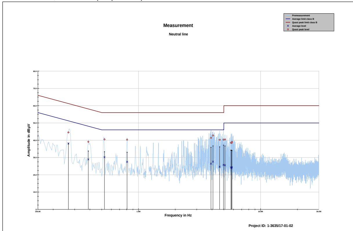
Plot 46: Neutral line, LB 565-01 (AC powered)
