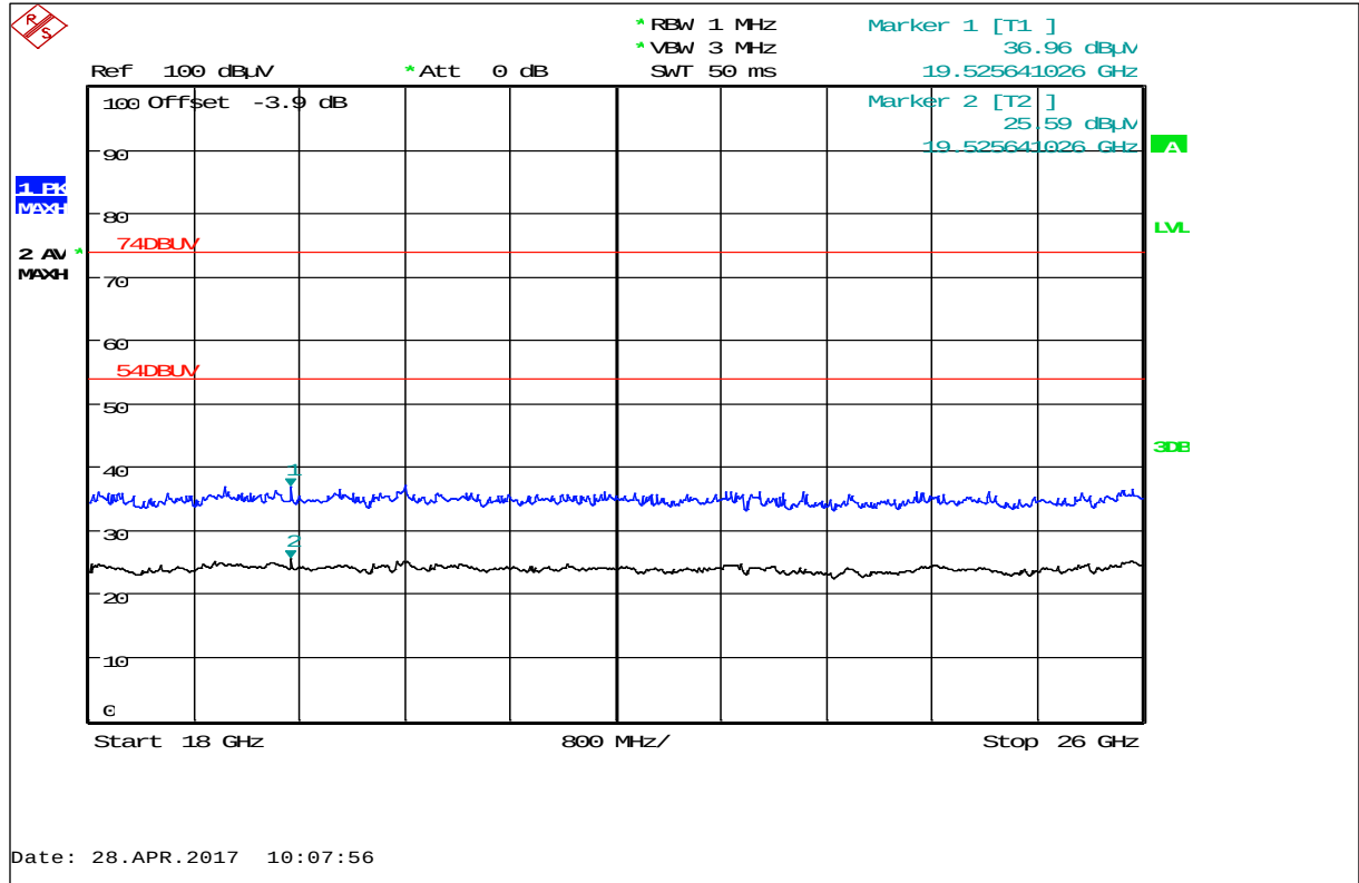
Plot 25: 18 GHz to 26 GHz, LB 565-01 (AC powered) with Tank sensor, horizontal / vertical polarization
