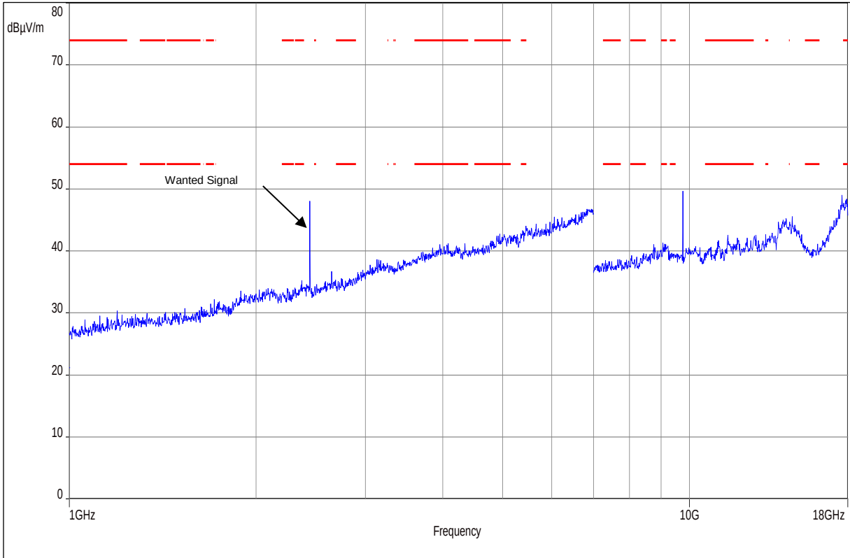
Plot 18: 1 GHz to 18 GHz, LB 565-01 (AC powered) with Flow cell sensor, horizontal / vertical polarization
