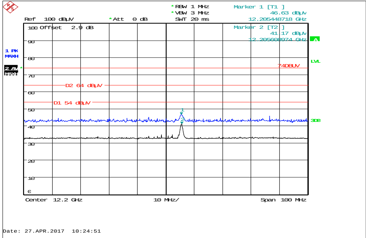
Plot 43: Harmonic 12.2 GHz, LB 565-02 (DC powered) with Tank sensor, horizontal / vertical polarization
