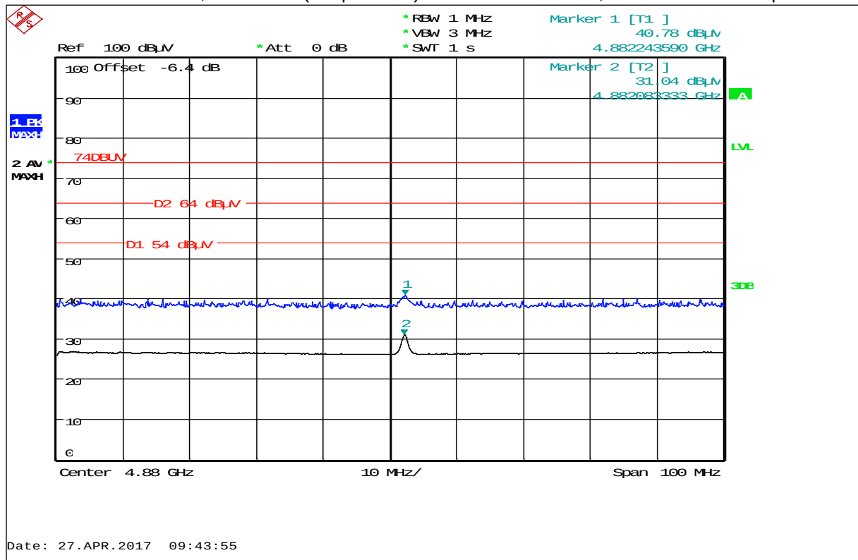
Plot 32: Harmonic 4.88 GHz, LB 565-02 (DC powered) with Flow cell sensor, horizontal / vertical polarization
