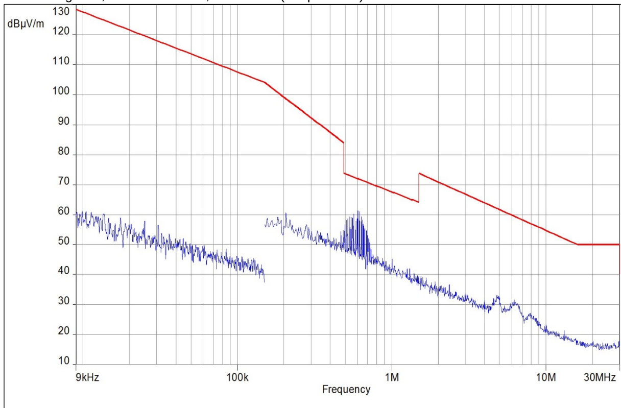
Plot 10: TX Magnetic, 9 kHz – 30 MHz, LB 565-01 (AC powered) with Flow cell sensor
