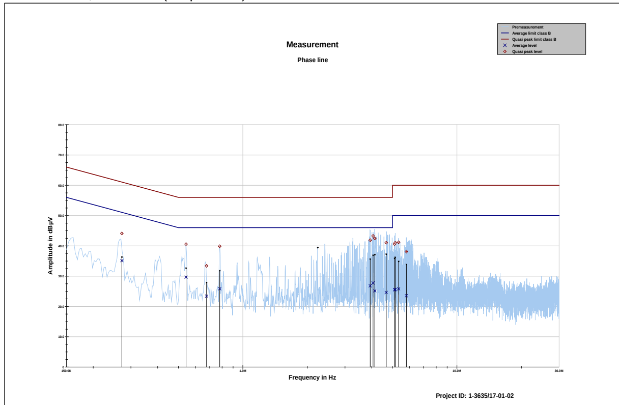
Plot 45: Phase line, LB 565-01 (AC powered)
