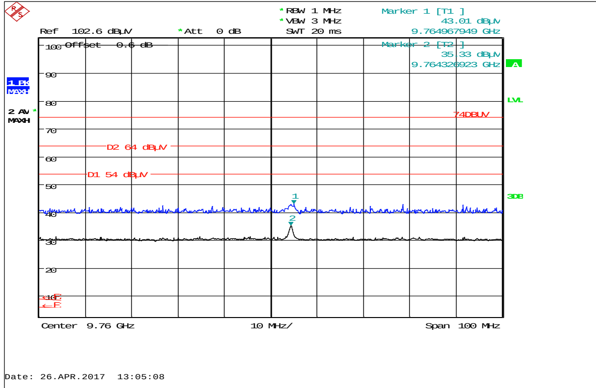
Plot 37: Harmonic 9.76 GHz, LB 565-01 (AC powered) with Tank sensor, horizontal / vertical polarization
