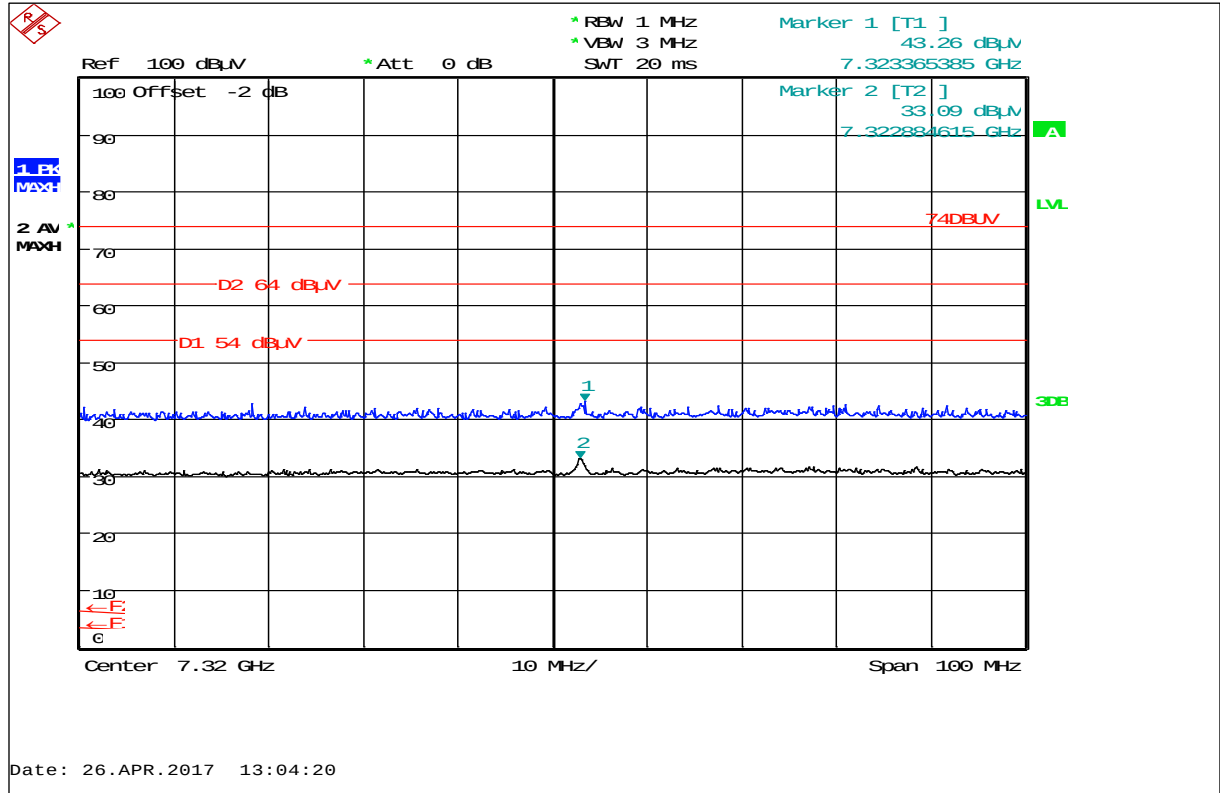
Plot 33: Harmonic 7.32 GHz, LB 565-01 (AC powered) with Tank sensor, horizontal / vertical polarization
