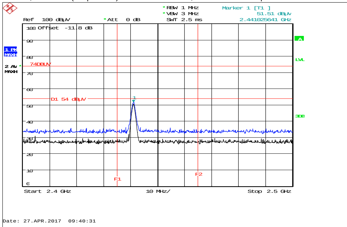
Plot 24: BEC, LB 565-02 (DC powered) with Flow cell sensor, horizontal / vertical polarization
