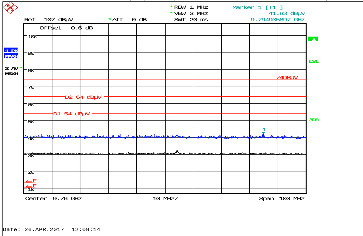
Plot 38: Harmonic 9.76 GHz, LB 565-01 (AC powered) with Flow cell sensor, horizontal / vertical polarization
