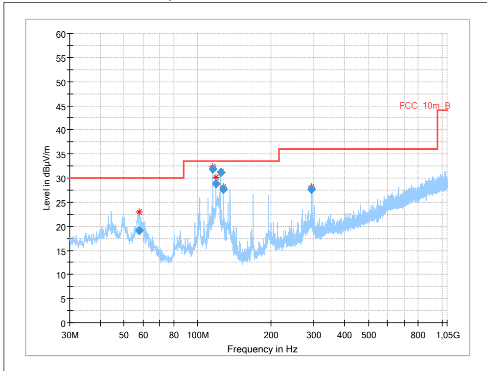
Plot 13: 30 MHz to 1 GHz, LB 565-01 (AC powered) with Tank sensor, horizontal / vertical polarization (115 V AC / 60 Hz; Ferrite on TP100 cable)
