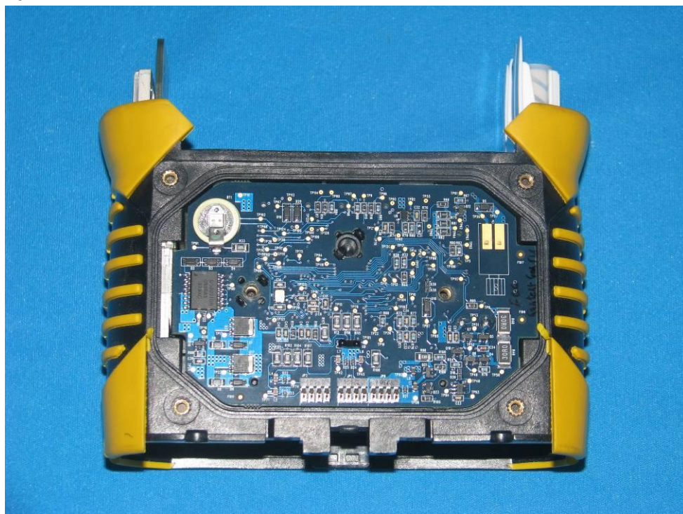
Main PCB
