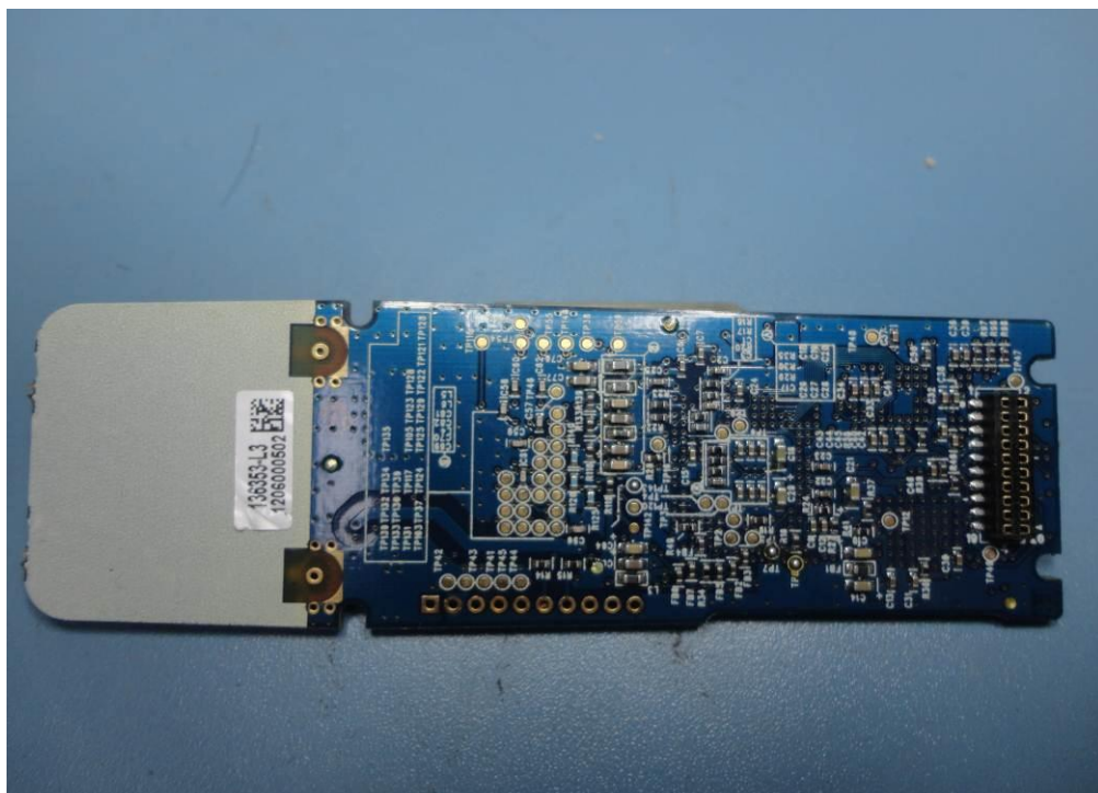
Module Unshielded - Bottom View
