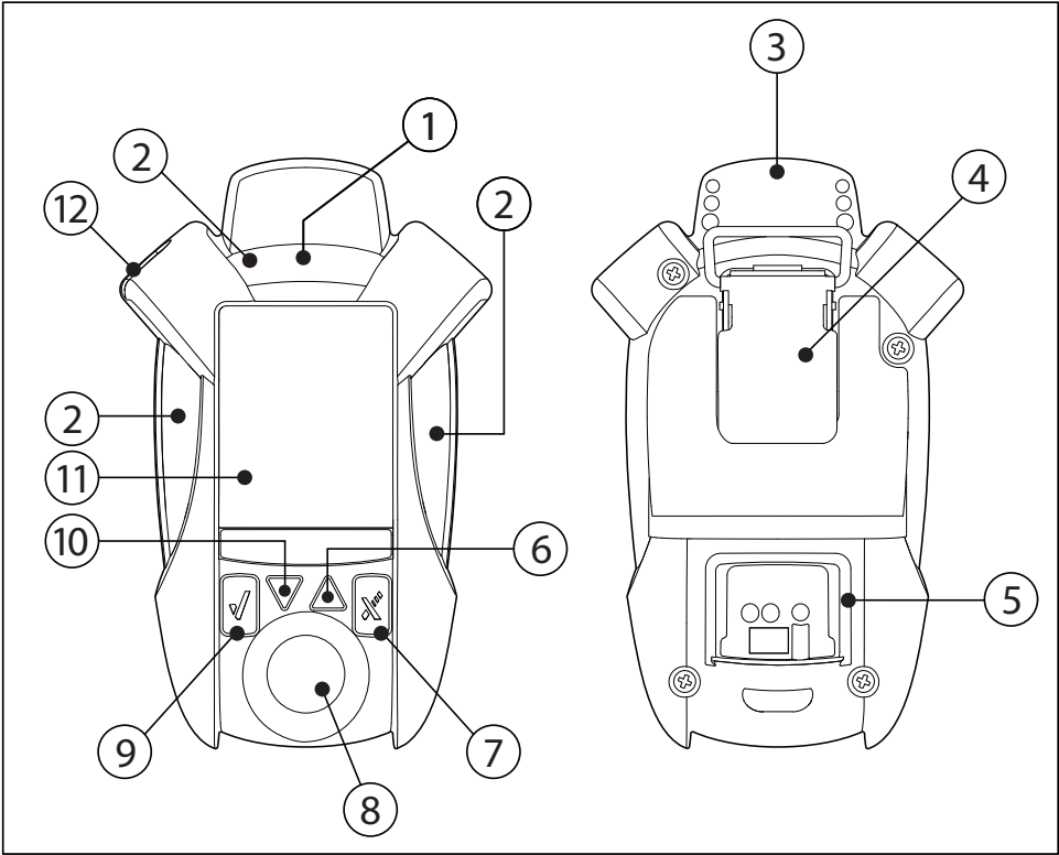
Figure 1. Parts of ConneX1
