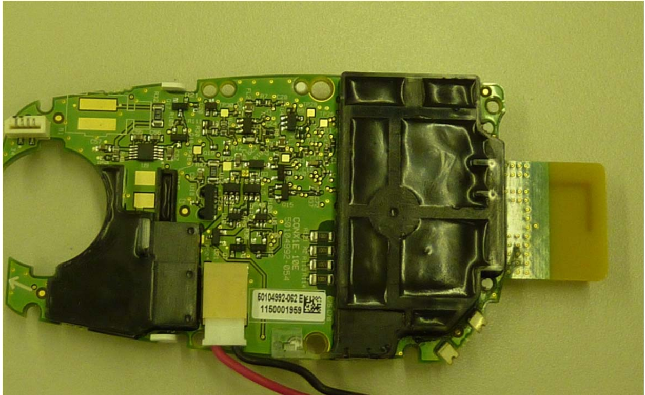
Production Model of ConneX1 with Radio module potted
