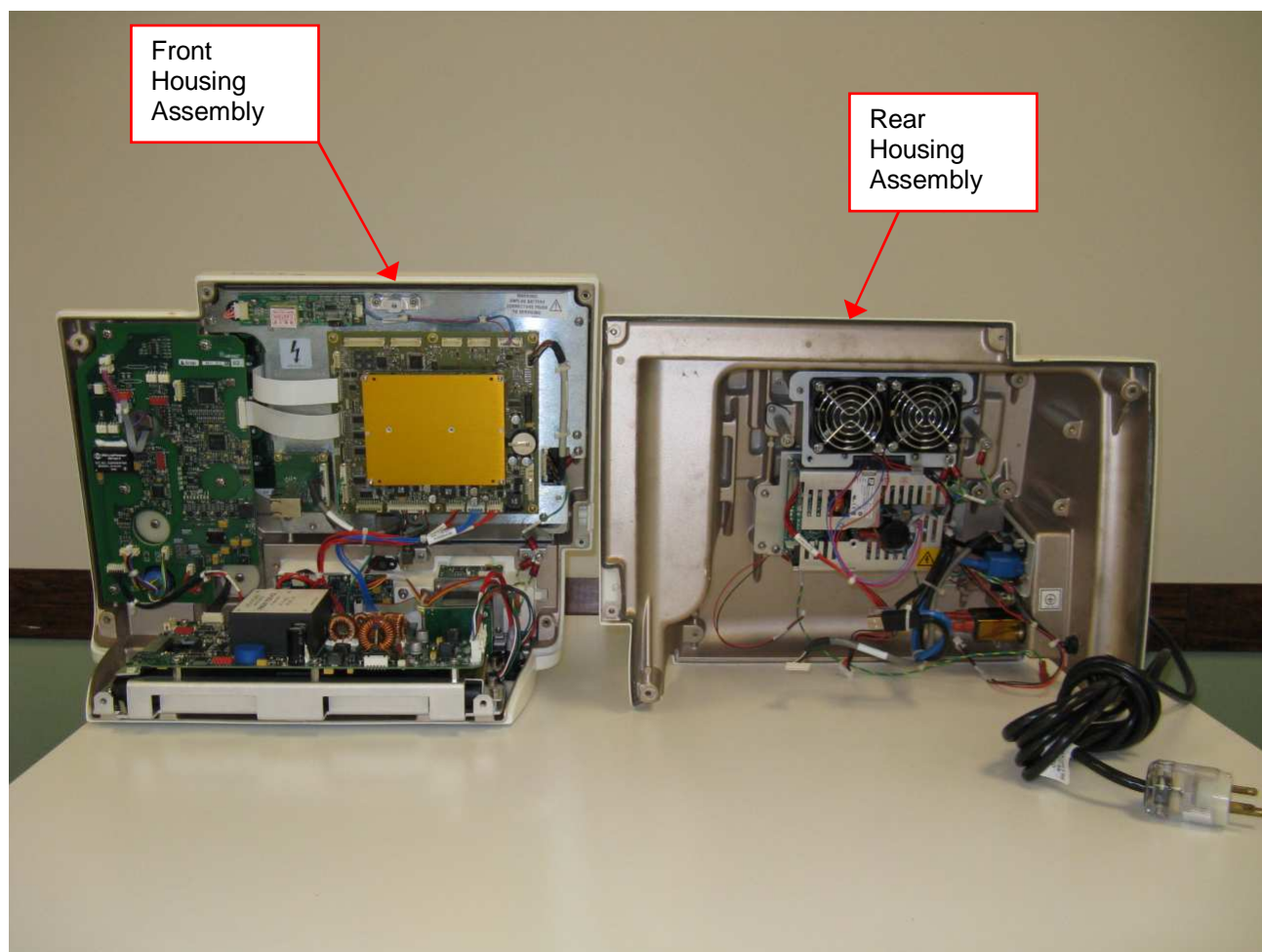
0042-4000 IMC Console – Front and Rear Housing Assemblies
