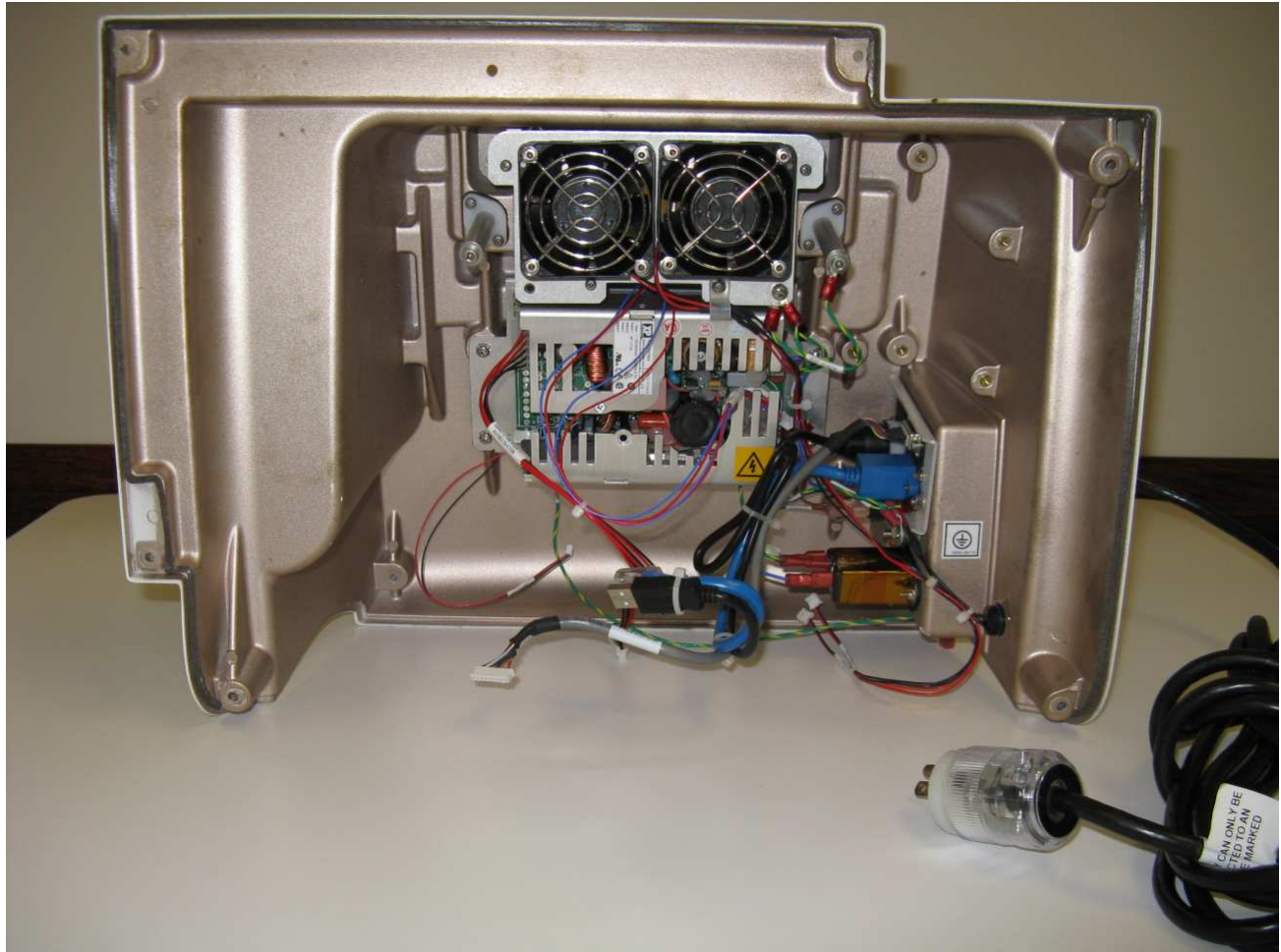
0042-4000 IMC Console – Rear Housing Assembly
