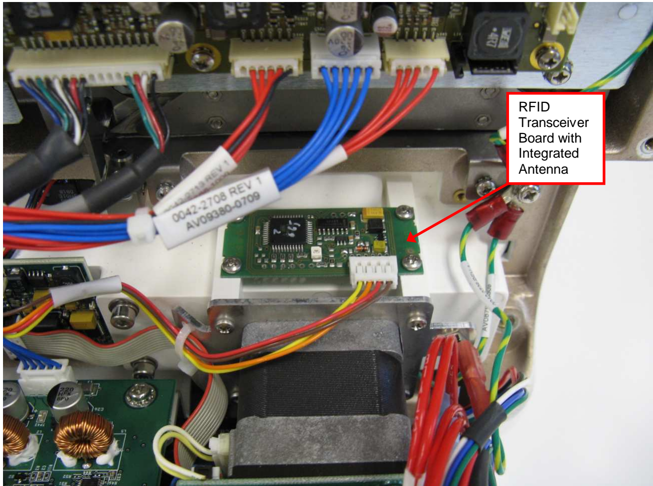
0042-4000 IMC Console – Front Housing Assembly Close-up of RFID Board with Integrated Loop Antenna
