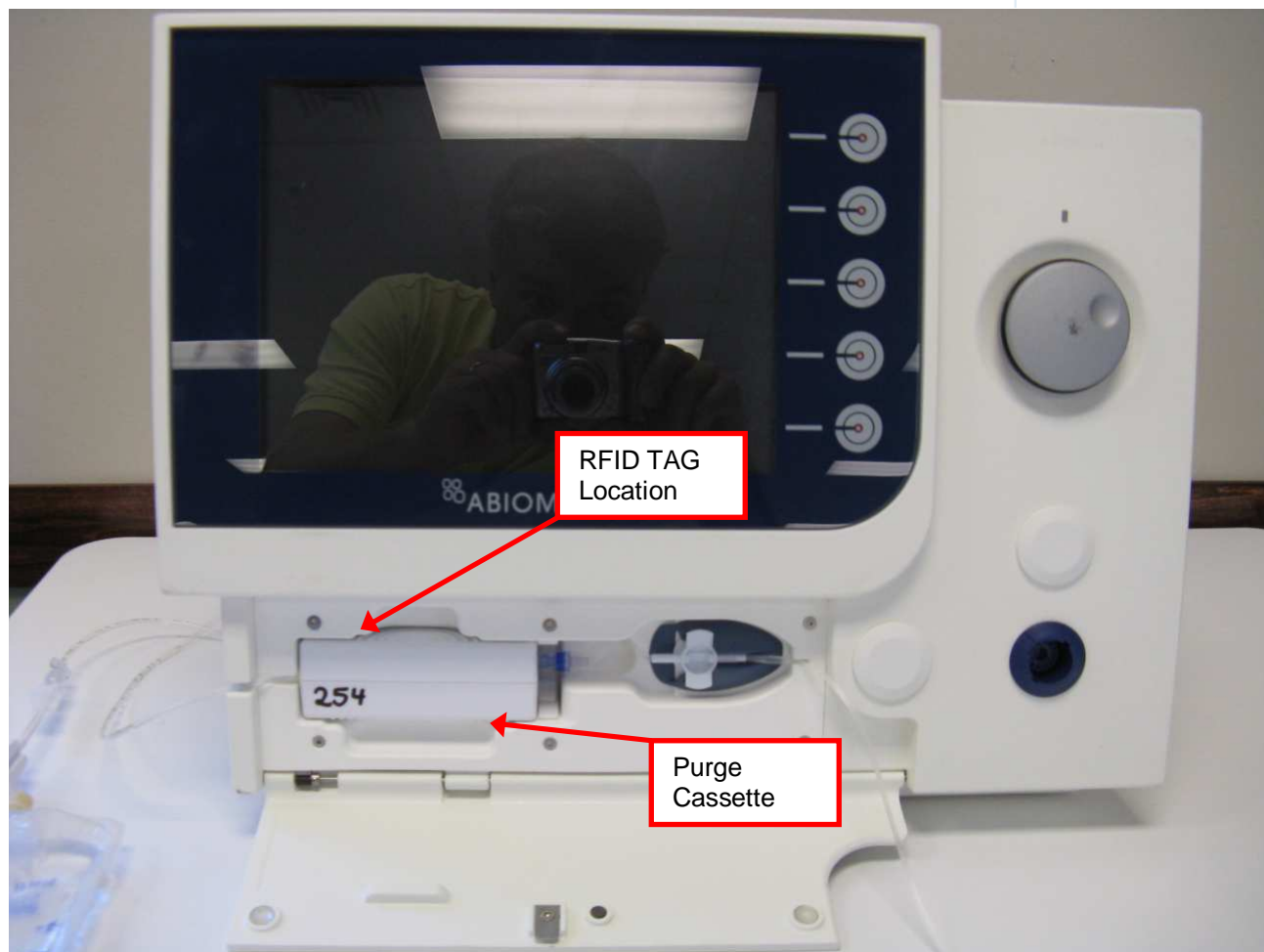
0042-4000 IMC Console – Front Housing Assembly (Front View)
