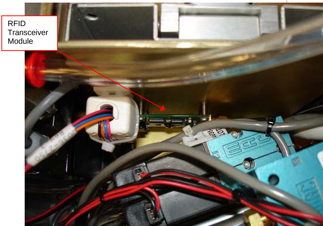
0036-0010 Recover BP – RFID Transceiver in Console (Close)
