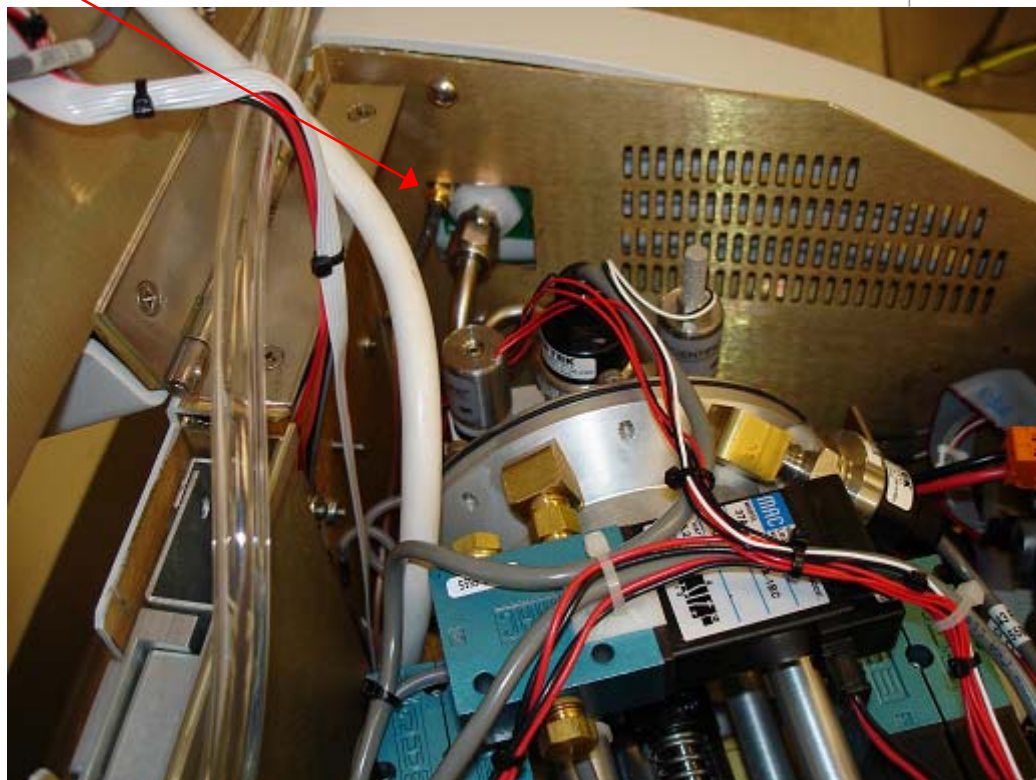
0036-0010 Recover BP – RFID Antenna & Coax Cable in Console (Close)
