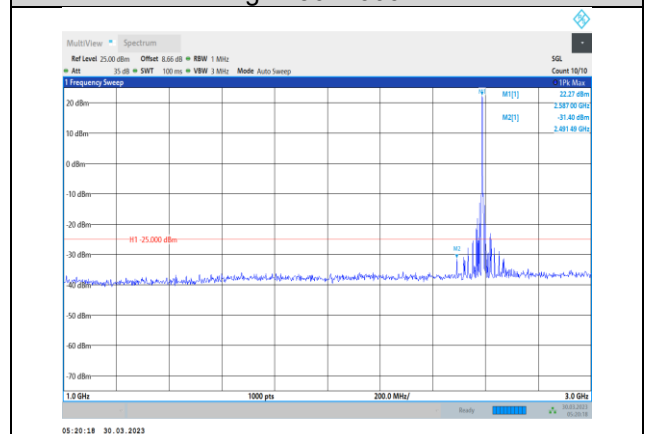
Band41-15MHz-64QAM-40620-1RB#0- Range2:1000~3000MHz
