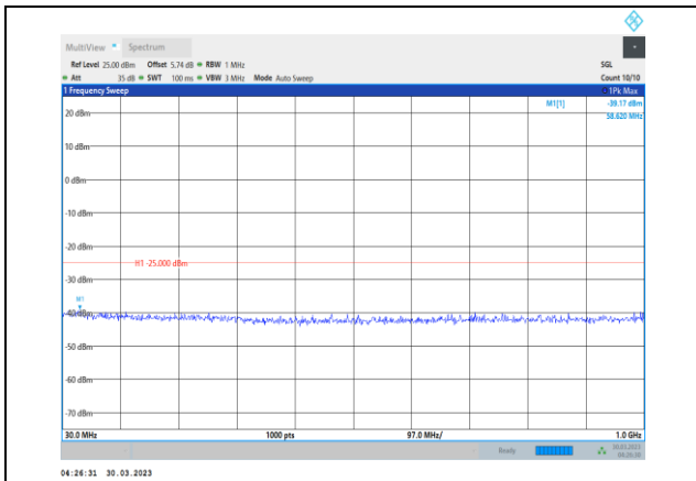
Band41-10MHz-16QAM-39700-1RB#0- Range1:30~1000MHz
