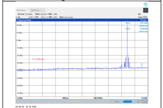
Band41-5MHz-16QAM-41565-1RB#0- Range2:1000~3000MHz
