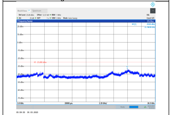
Band38-20MHz-64QAM-37850-1RB#0- Range3:3000~26500MHz
