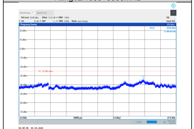
Band41-5MHz-16QAM-41565-1RB#0- Range3:3000~27000MHz
