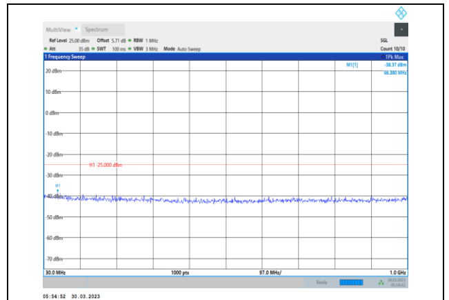
Band38-15MHz-64QAM-38000-1RB#0- Range1:30~1000MHz
