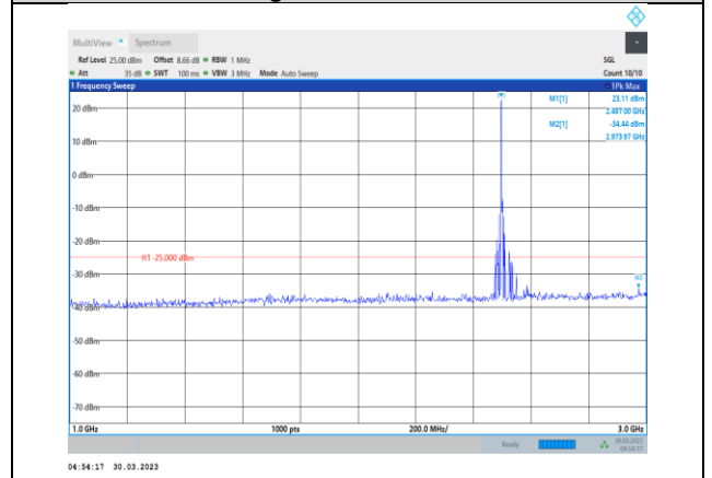
Band41-5MHz-16QAM-39675-1RB#0- Range2:1000~3000MHz
