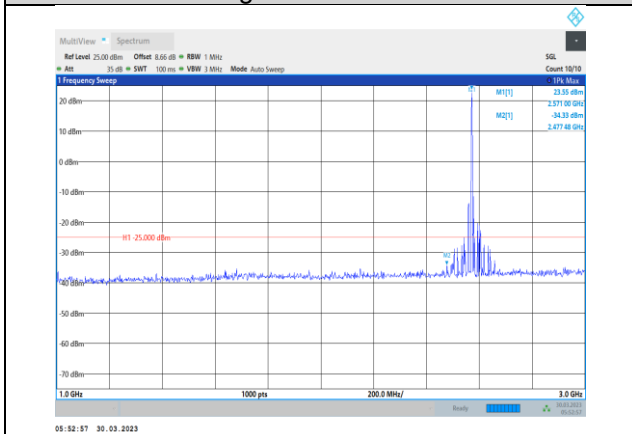
Band38-15MHz-64QAM-37825-1RB#0- Range2:1000~3000MHz
