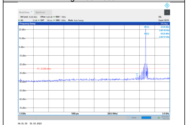
Band41-10MHz-64QAM-41540-1RB#0- Range2:1000~3000MHz
