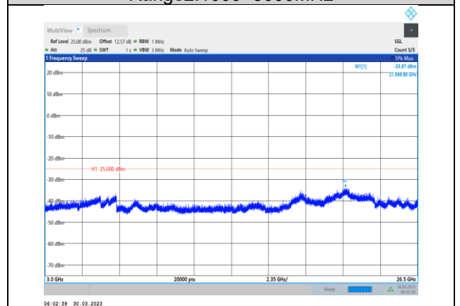
Band38-20MHz-QPSK-38150-1RB#0- Range3:3000~26500MHz
