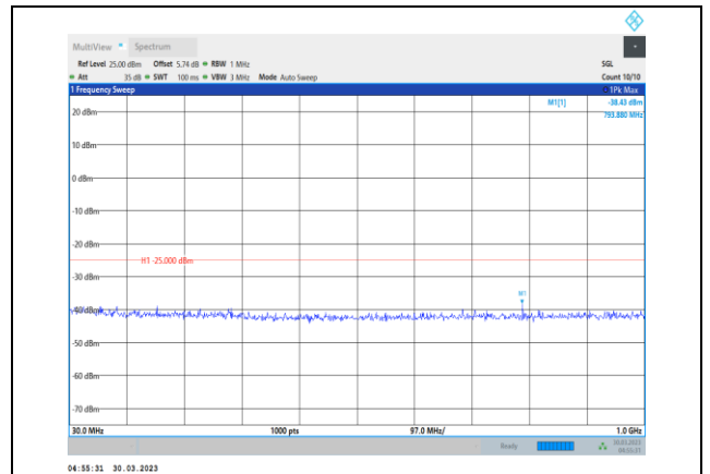
Band41-5MHz-QPSK-40620-1RB#0- Range1:30~1000MHz
