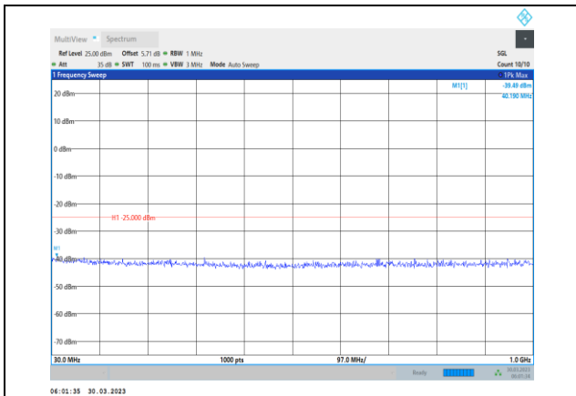
Band38-20MHz-64QAM-38000-1RB#0- Range1:30~1000MHz
