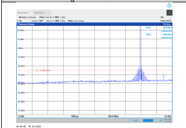
Band41-10MHz-64QAM-40620-1RB#0- Range2:1000~3000MHz
