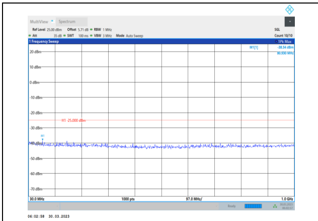
Band38-20MHz-16QAM-38150-1RB#0- Range1:30~1000MHz
