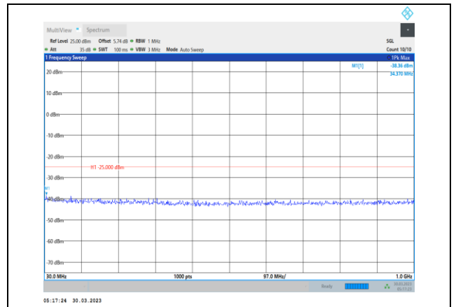
Band41-15MHz-16QAM-39725-1RB#0- Range1:30~1000MHz
