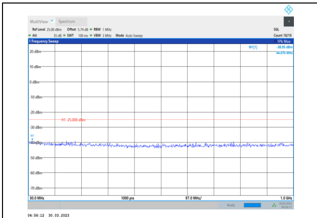
Band41-5MHz-16QAM-40620-1RB#0- Range1:30~1000MHz
