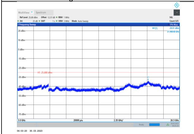
Band38-20MHz-16QAM-38150-1RB#0- Range3:3000~26500MHz
