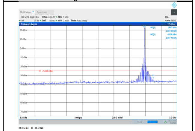
Band38-20MHz-16QAM-38000-1RB#0- Range2:1000~3000MHz
