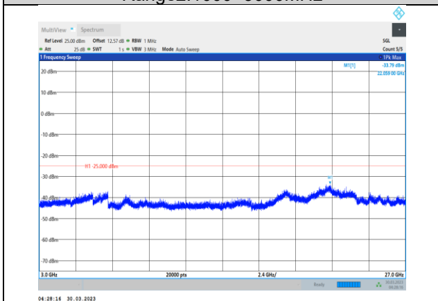
Band41-10MHz-QPSK-40620-1RB#0- Range3:3000~27000MHz
