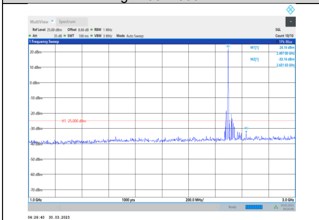
Band41-10MHz-16QAM-39700-1RB#0- Range2:1000~3000MHz
