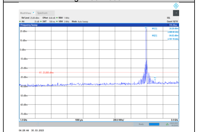
Band41-10MHz-16QAM-40620-1RB#0- Range2:1000~3000MHz
