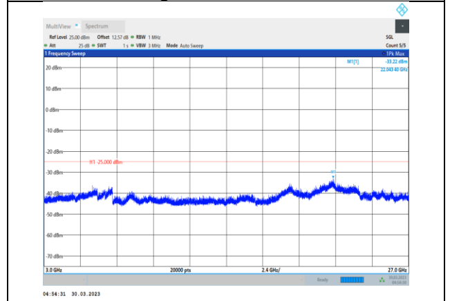
Band41-5MHz-16QAM-39675-1RB#0- Range3:3000~27000MHz
