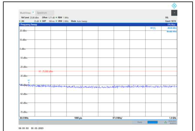
Band38-20MHz-16QAM-38000-1RB#0- Range1:30~1000MHz
