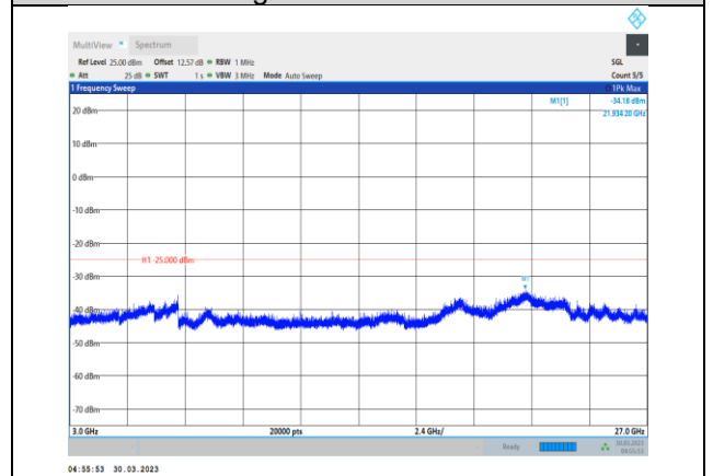
Band41-5MHz-QPSK-40620-1RB#0- Range3:3000~27000MHz
