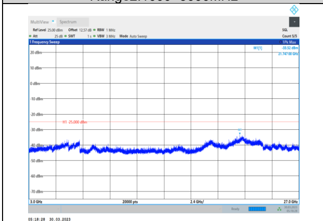
Band41-15MHz-64QAM-39725-1RB#0- Range3:3000~27000MHz
