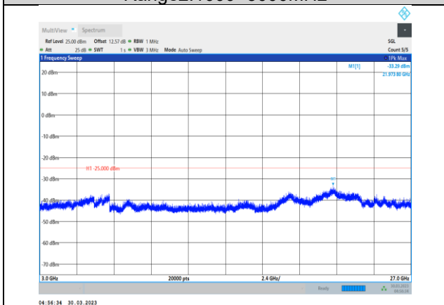
Band41-5MHz-16QAM-40620-1RB#0- Range3:3000~27000MHz
