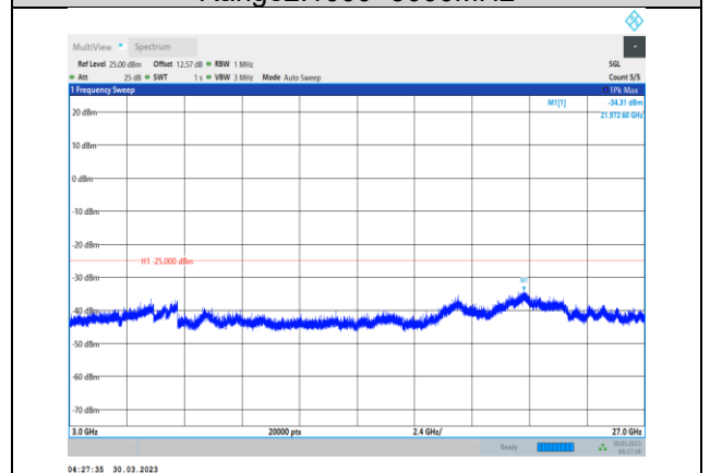
Band41-10MHz-64QAM-39700-1RB#0- Range3:3000~27000MHz
