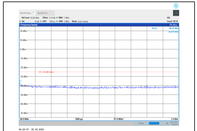
Band41-10MHz-QPSK-41540-1RB#0- Range1:30~1000MHz
