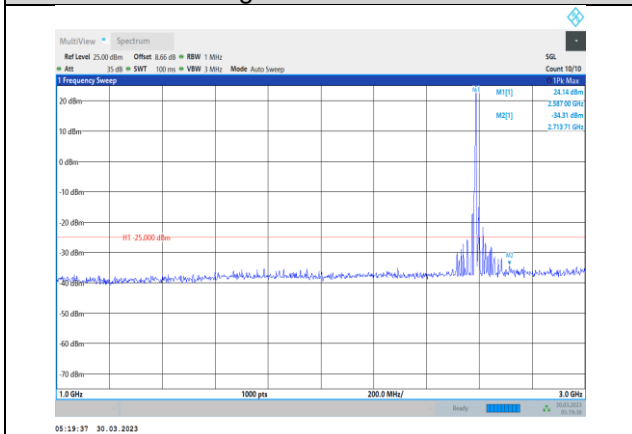
Band41-15MHz-16QAM-40620-1RB#0- Range2:1000~3000MHz
