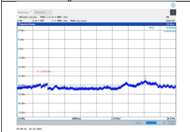
Band38-20MHz-16QAM-37850-1RB#0- Range3:3000~26500MHz
