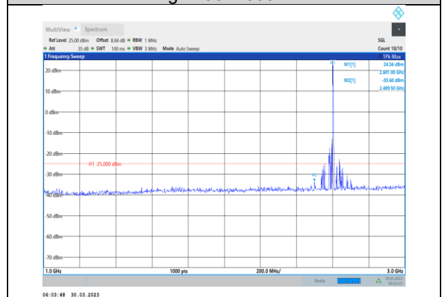
Band38-20MHz-64QAM-38150-1RB#0- Range2:1000~3000MHz
