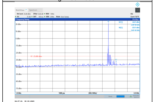
Band41-10MHz-64QAM-39700-1RB#0- Range2:1000~3000MHz
