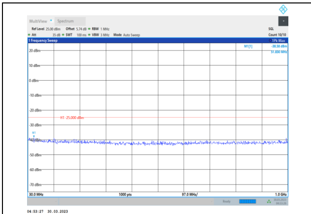
Band41-5MHz-QPSK-39675-1RB#0- Range1:30~1000MHz
