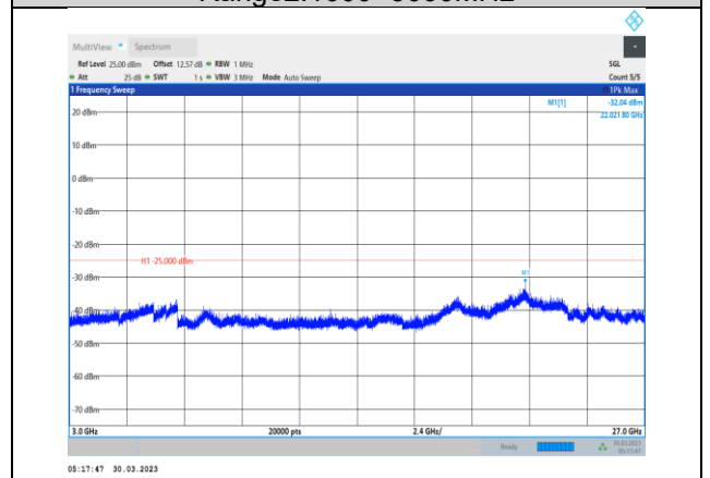
Band41-15MHz-16QAM-39725-1RB#0- Range3:3000~27000MHz
