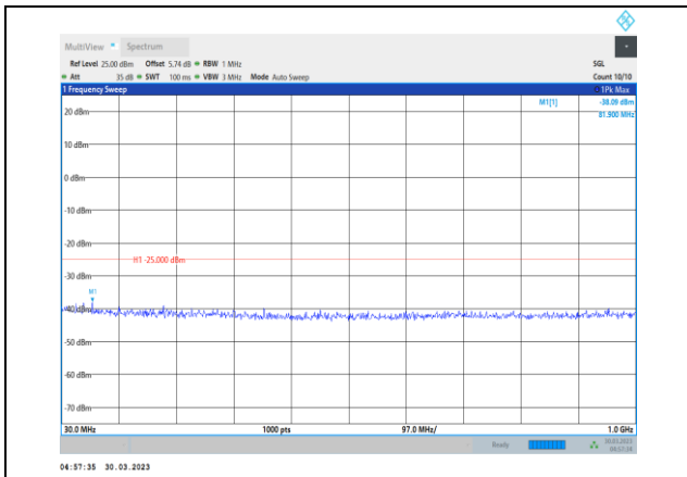
Band41-5MHz-QPSK-41565-1RB#0- Range1:30~1000MHz
