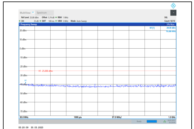
Band41-15MHz-64QAM-40620-1RB#0- Range1:30~1000MHz
