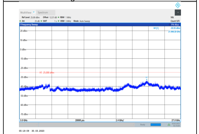
Band41-15MHz-QPSK-40620-1RB#0- Range3:3000~27000MHz
