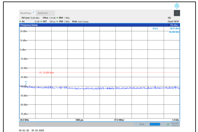
Band41-15MHz-16QAM-41515-1RB#0- Range1:30~1000MHz
