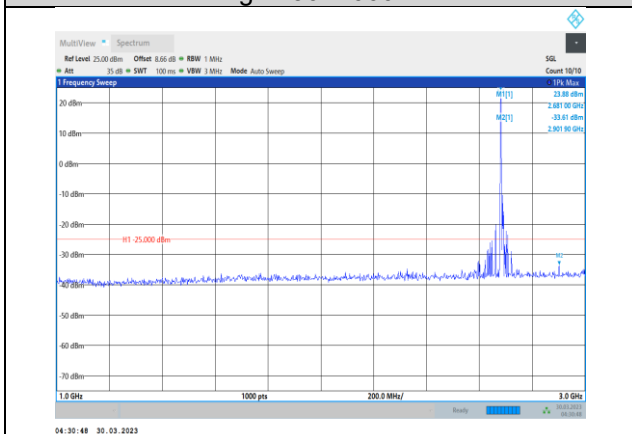
Band41-10MHz-16QAM-41540-1RB#0- Range2:1000~3000MHz
