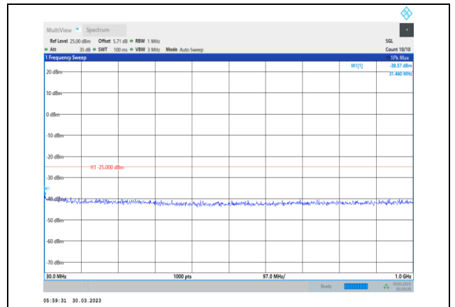
Band38-20MHz-64QAM-37850-1RB#0- Range1:30~1000MHz
