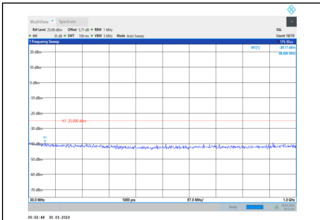
Band38-15MHz-64QAM-37825-1RB#0- Range1:30~1000MHz
