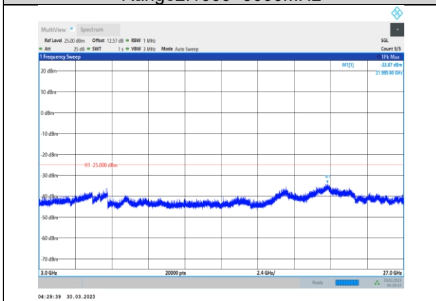
Band41-10MHz-64QAM-40620-1RB#0- Range3:3000~27000MHz
