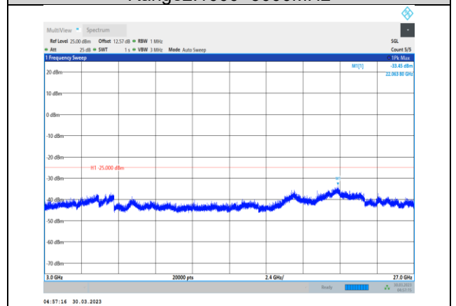
Band41-5MHz-64QAM-40620-1RB#0- Range3:3000~27000MHz
