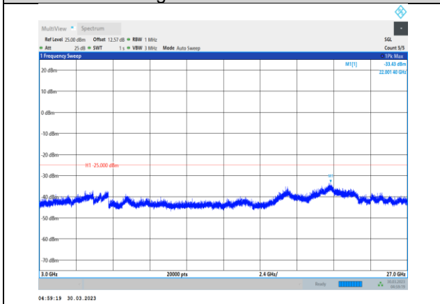
Band41-5MHz-64QAM-41565-1RB#0- Range3:3000~27000MHz
