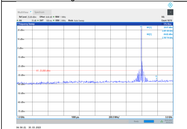
Band41-5MHz-16QAM-40620-1RB#0- Range2:1000~3000MHz
