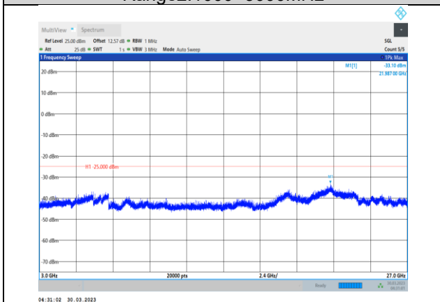
Band41-10MHz-16QAM-41540-1RB#0- Range3:3000~27000MHz
