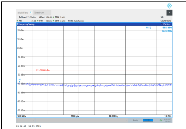
Band41-15MHz-QPSK-39725-1RB#0- Range1:30~1000MHz
