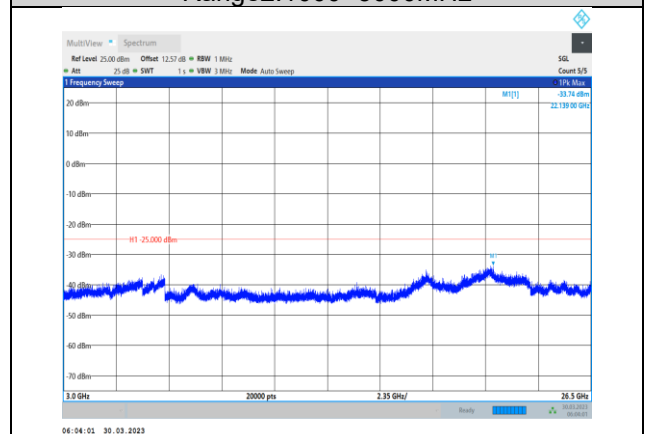
Band38-20MHz-64QAM-38150-1RB#0- Range3:3000~26500MHz
