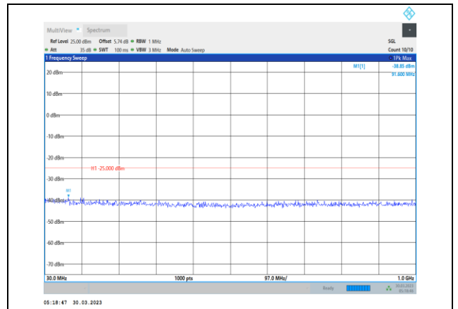
Band41-15MHz-QPSK-40620-1RB#0- Range1:30~1000MHz
