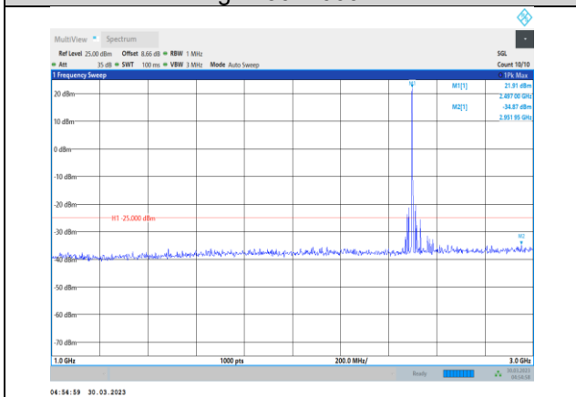
Band41-5MHz-64QAM-39675-1RB#0- Range2:1000~3000MHz
