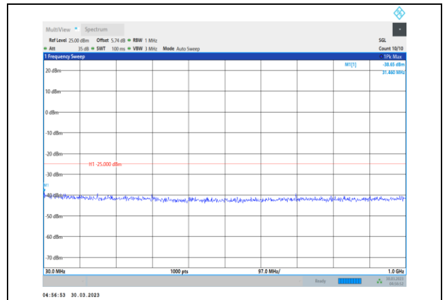
Band41-5MHz-64QAM-40620-1RB#0- Range1:30~1000MHz
