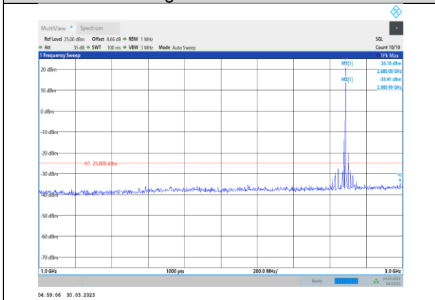
Band41-5MHz-64QAM-41565-1RB#0- Range2:1000~3000MHz
