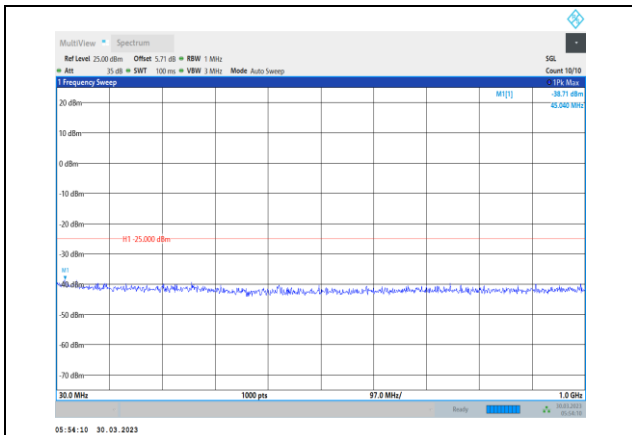
Band38-15MHz-16QAM-38000-1RB#0- Range1:30~1000MHz
