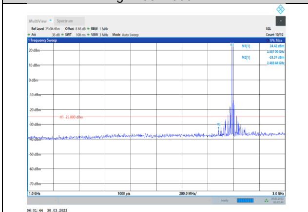
Band38-20MHz-64QAM-38000-1RB#0- Range2:1000~3000MHz
