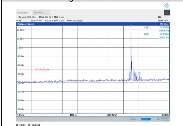
Band41-15MHz-64QAM-39725-1RB#0- Range2:1000~3000MHz
