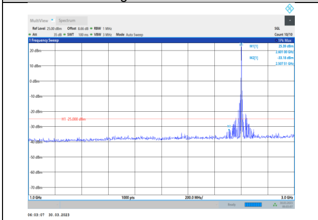
Band38-20MHz-16QAM-38150-1RB#0- Range2:1000~3000MHz
