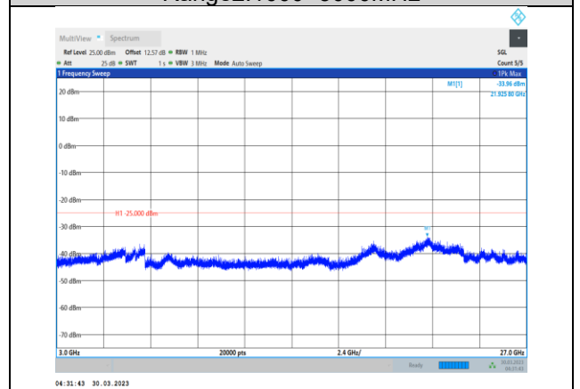
Band41-10MHz-64QAM-41540-1RB#0- Range3:3000~27000MHz
