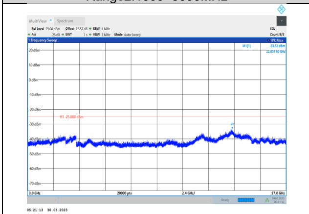
Band41-15MHz-QPSK-41515-1RB#0- Range3:3000~27000MHz
