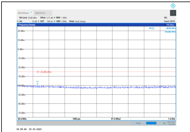
Band38-20MHz-16QAM-37850-1RB#0- Range1:30~1000MHz
