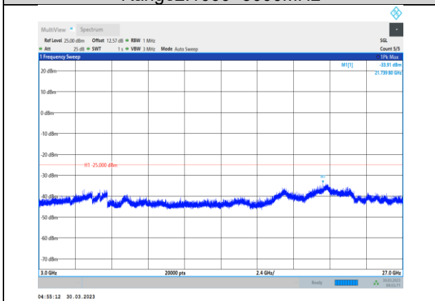
Band41-5MHz-64QAM-39675-1RB#0- Range3:3000~27000MHz
