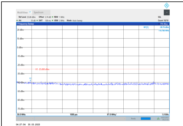
Band41-10MHz-QPSK-40620-1RB#0- Range1:30~1000MHz
