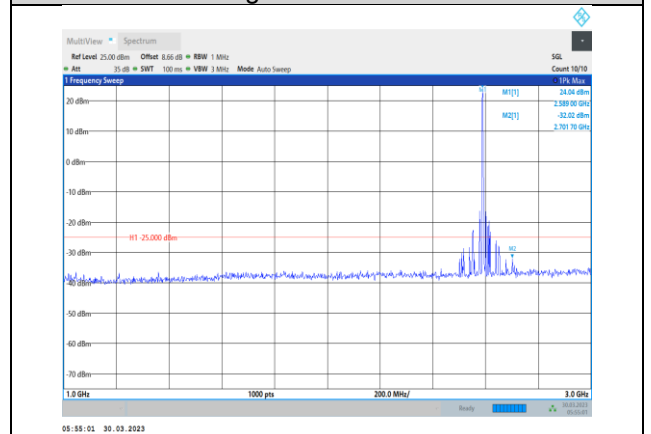
Band38-15MHz-64QAM-38000-1RB#0- Range2:1000~3000MHz
