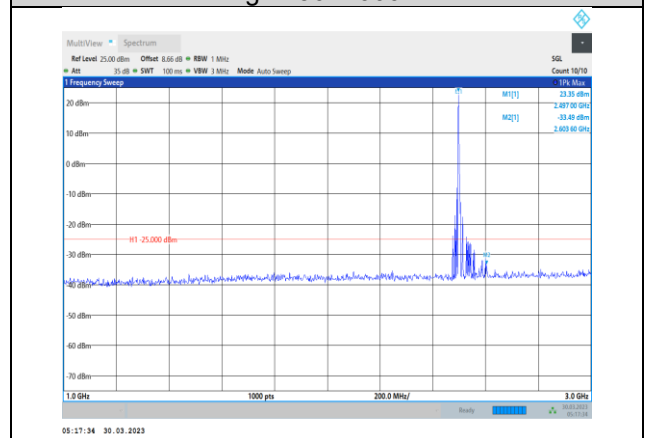
Band41-15MHz-16QAM-39725-1RB#0- Range2:1000~3000MHz
