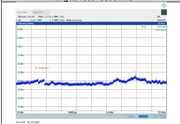
Band41-10MHz-16QAM-39700-1RB#0- Range3:3000~27000MHz
