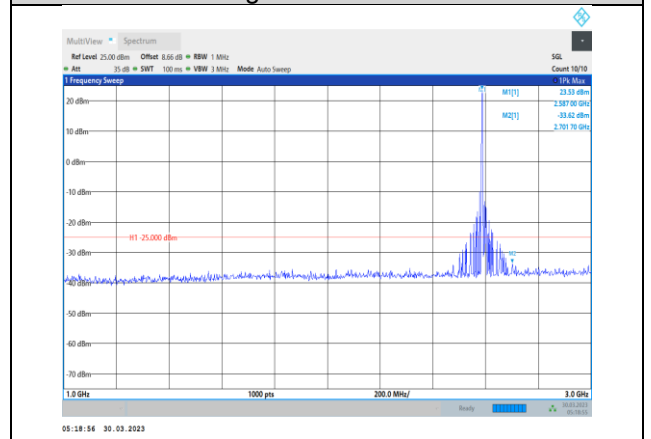
Band41-15MHz-QPSK-40620-1RB#0- Range2:1000~3000MHz
