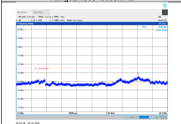
Band38-20MHz-QPSK-38000-1RB#0- Range3:3000~26500MHz
