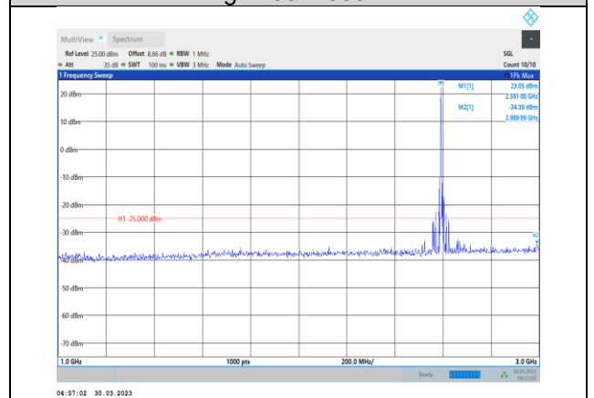
Band41-5MHz-64QAM-40620-1RB#0- Range2:1000~3000MHz
