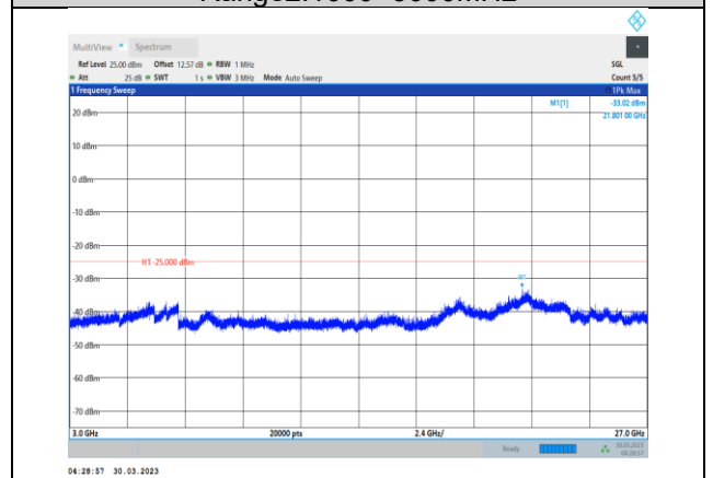
Band41-10MHz-16QAM-40620-1RB#0- Range3:3000~27000MHz
