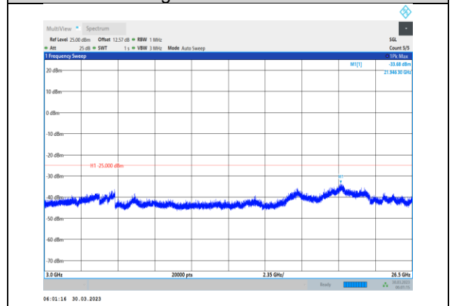
Band38-20MHz-16QAM-38000-1RB#0- Range3:3000~26500MHz
