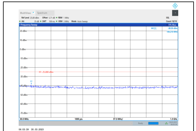
Band38-20MHz-64QAM-38150-1RB#0- Range1:30~1000MHz
