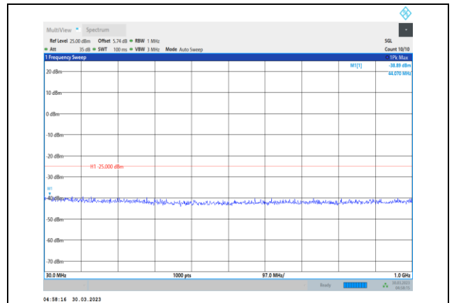
Band41-5MHz-16QAM-41565-1RB#0- Range1:30~1000MHz
