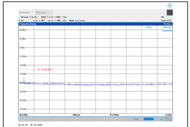
Band41-10MHz-64QAM-41540-1RB#0- Range1:30~1000MHz
