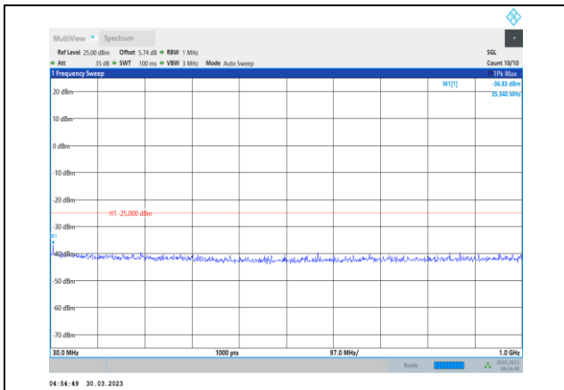
Band41-5MHz-64QAM-39675-1RB#0- Range1:30~1000MHz
