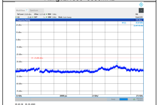
Band41-15MHz-64QAM-40620-1RB#0- Range3:3000~27000MHz
