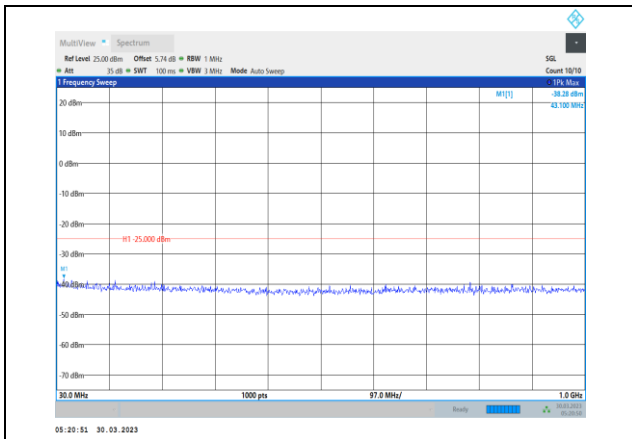
Band41-15MHz-QPSK-41515-1RB#0- Range1:30~1000MHz
