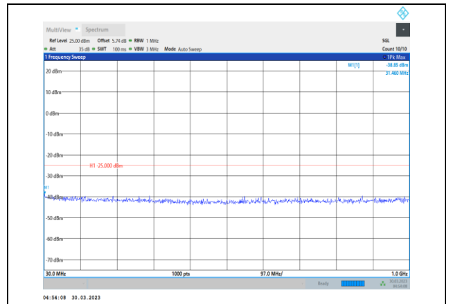
Band41-5MHz-16QAM-39675-1RB#0- Range1:30~1000MHz
