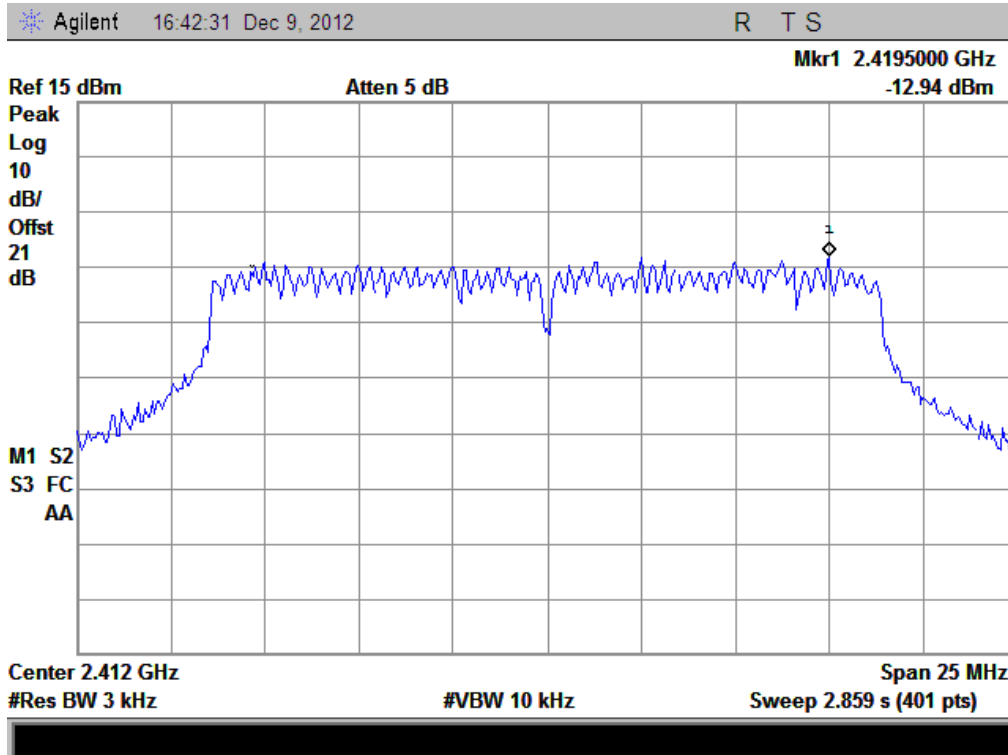
(Plot A: Channel = 1 @ 802.11n)
