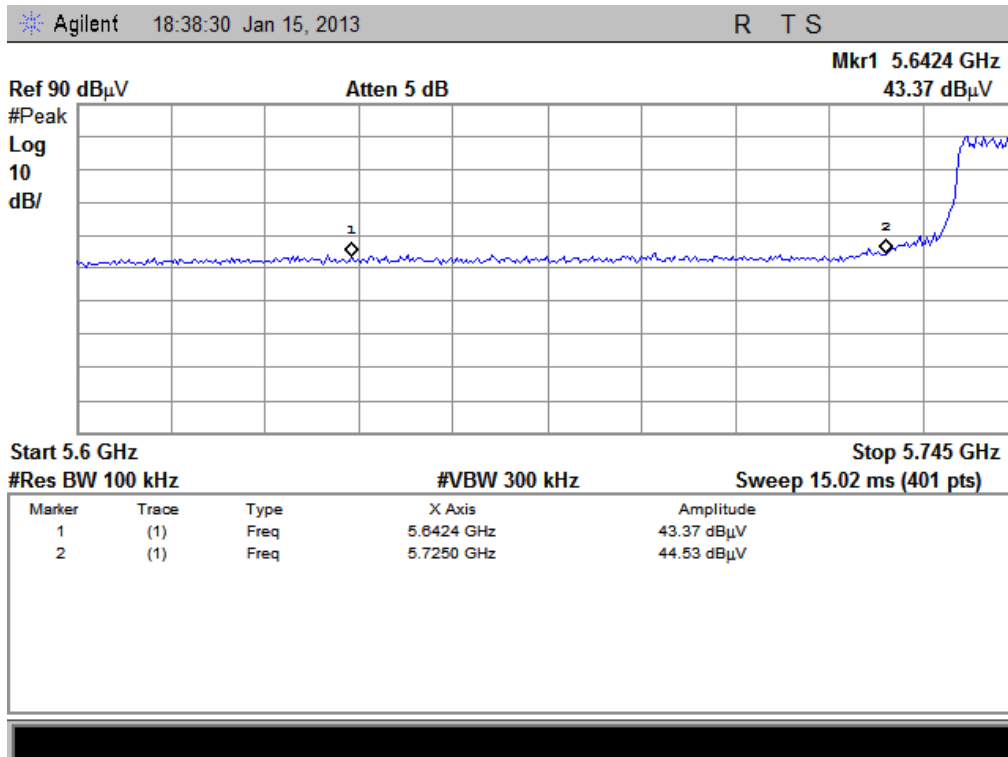
(Plot E1: Channel = 149 PEAK @ 802.11n-20)
