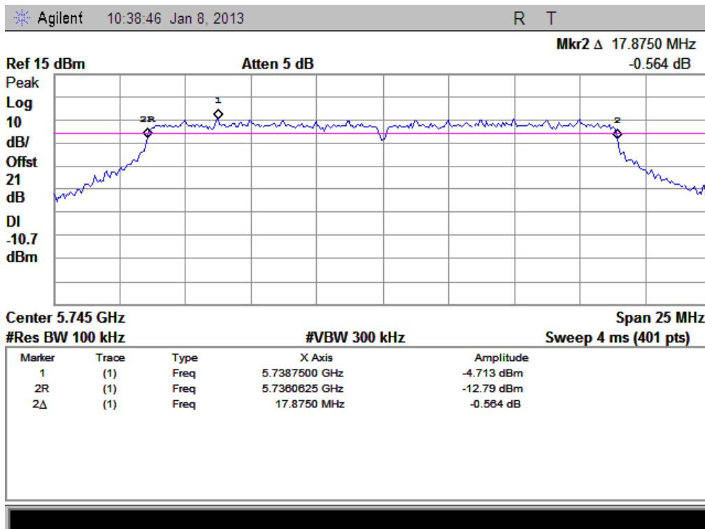
(Plot G: Channel 149: 5745MHz @ 802.11n-20)
