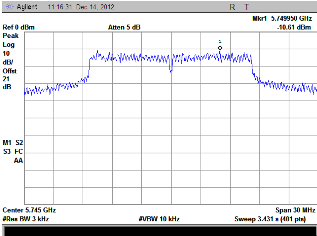
(Plot A: Channel = 149 @ 802.11a)
