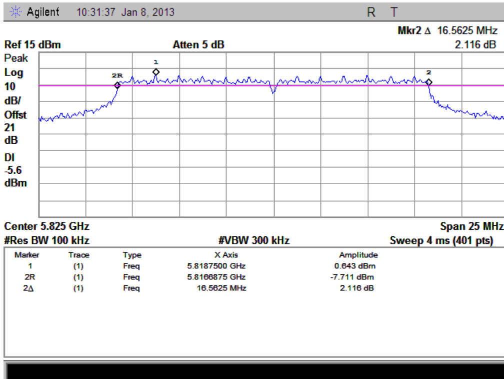
(Plot C: Channel 165: 5825MHz @ 802.11a)
