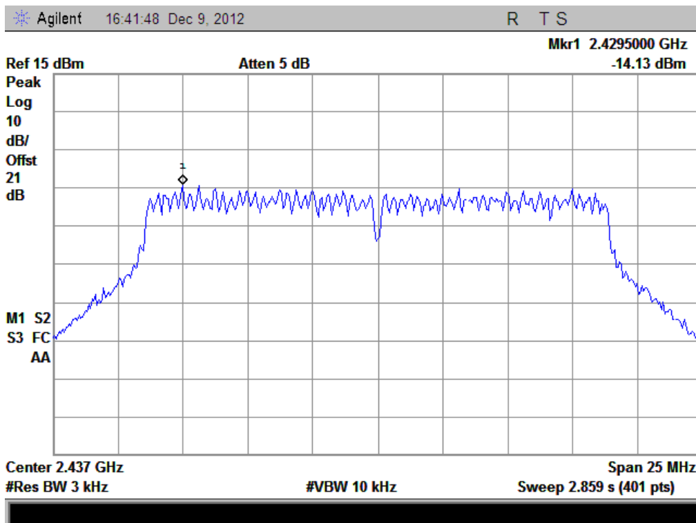
(Plot B: Channel = 6 @ 802.11n)
