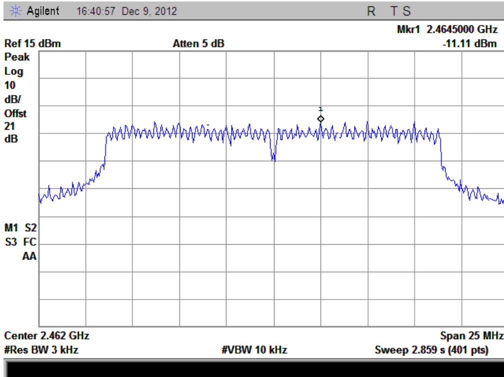
(Plot C: Channel = 11 @ 802.11n)
