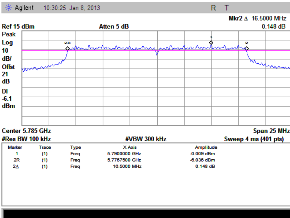
(Plot B: Channel 157: 5785MHz @ 802.11a)
