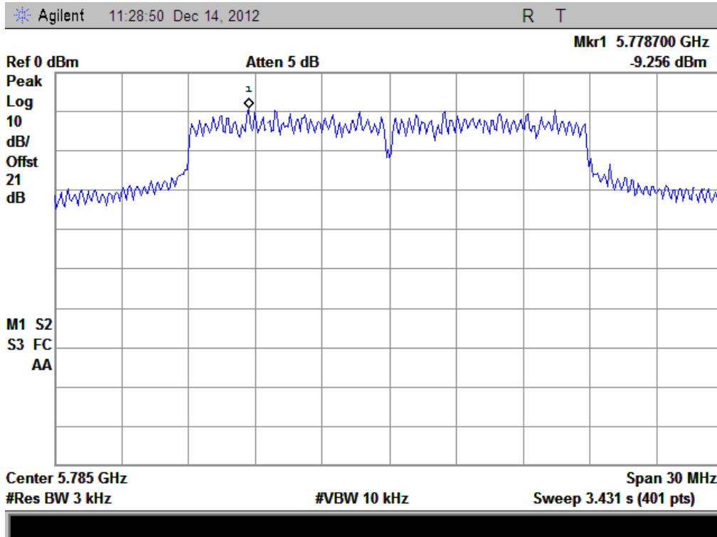
(Plot E: Channel = 157 @ 802.11n)
