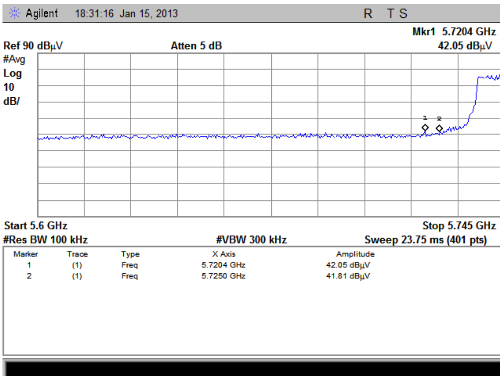
(Plot A2: Channel = 149 AVG @ 802.11b)
