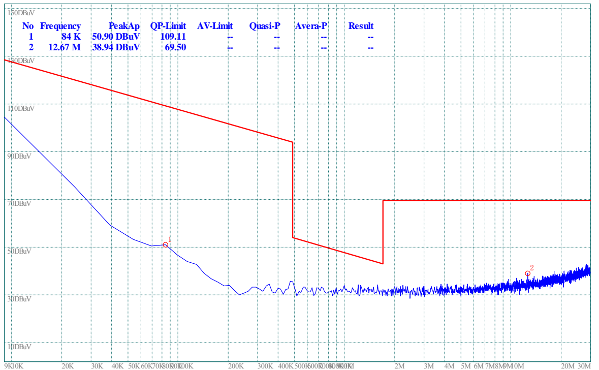
(Plot J.1: 9kHz to 30MHz)
