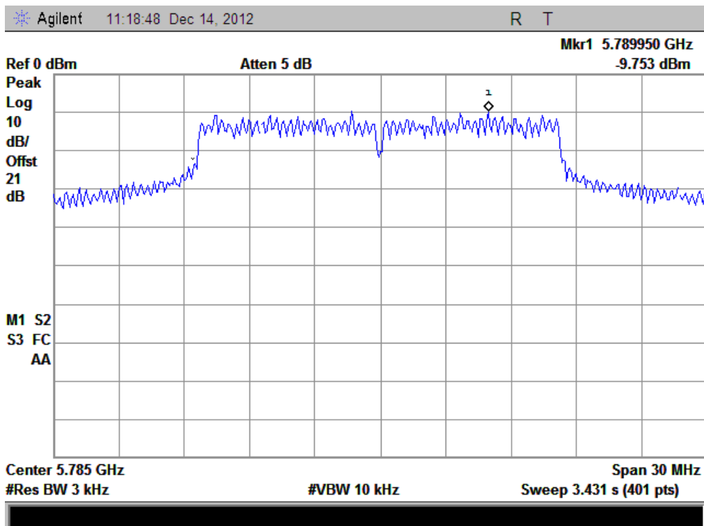
(Plot B: Channel = 157 @ 802.11a)
