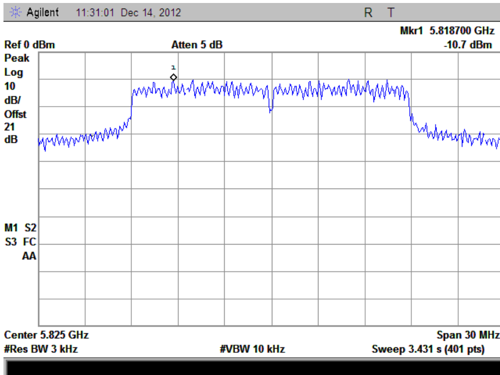
(Plot F: Channel = 165 @ 802.11n)
