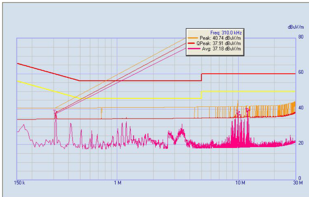
(Plot C: L Phase)
