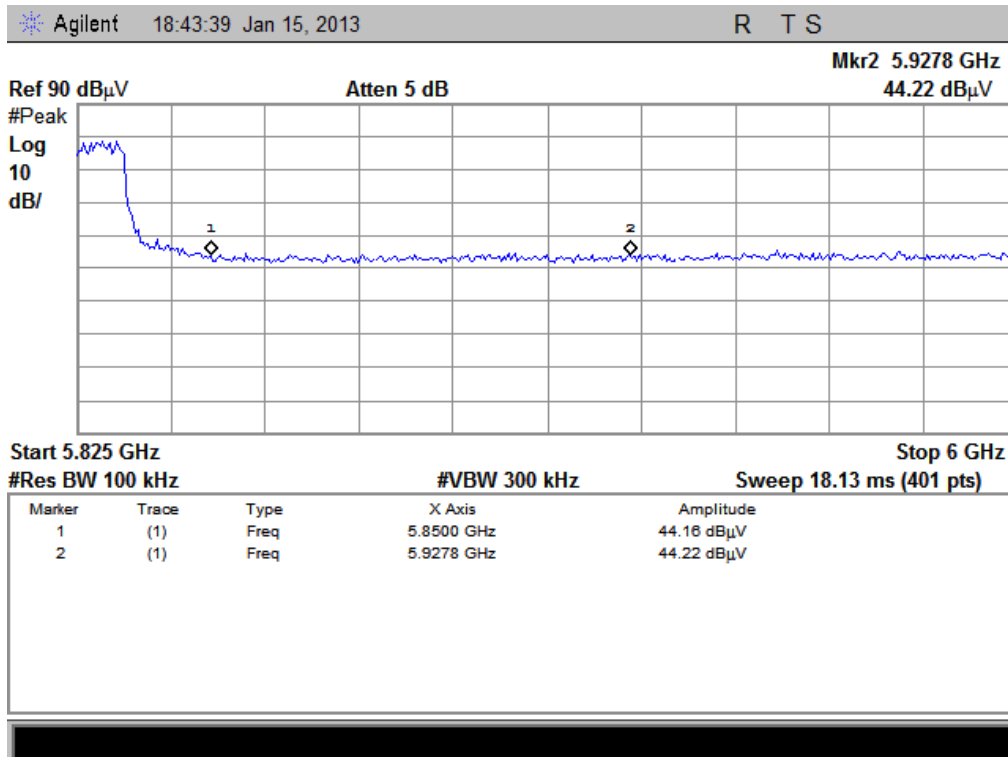
(Plot F1: Channel = 165 PEAK @ 802.11n-20)
