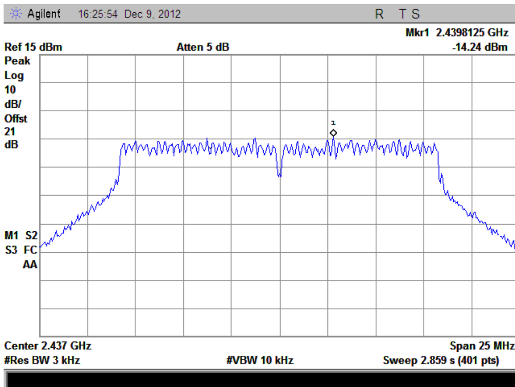
(Plot B: Channel = 6 @ 802.11g)
