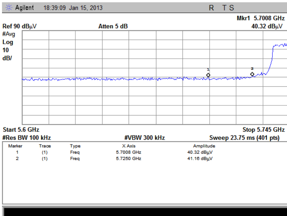
(Plot E2: Channel = 149 AVG @ 802.11n-20)
