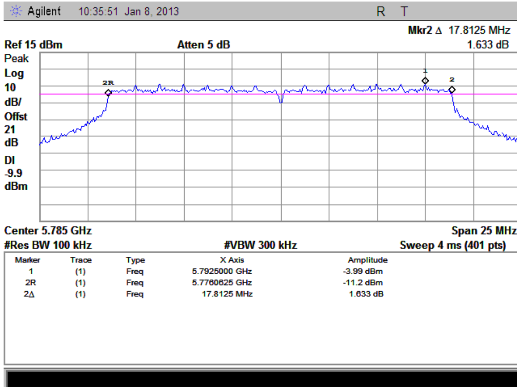
(Plot H: Channel 157: 5785MHz @ 802.11n-20)
