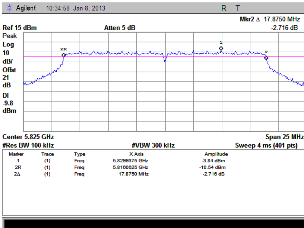
(Plot I: Channel 165: 5825MHz @ 802.11n-20)
