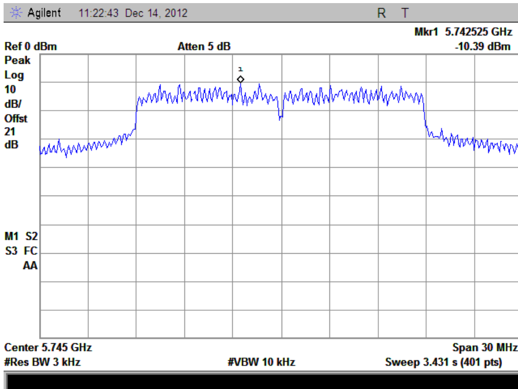
(Plot D: Channel = 149 @ 802.11n)
