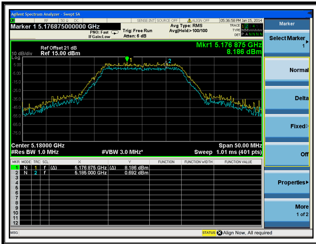
(Channel 36: 5180MHz @ 802.11a)
