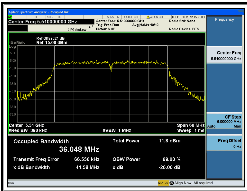
(Channel 102: 5510MHz @ 802.11n-40MHz)
