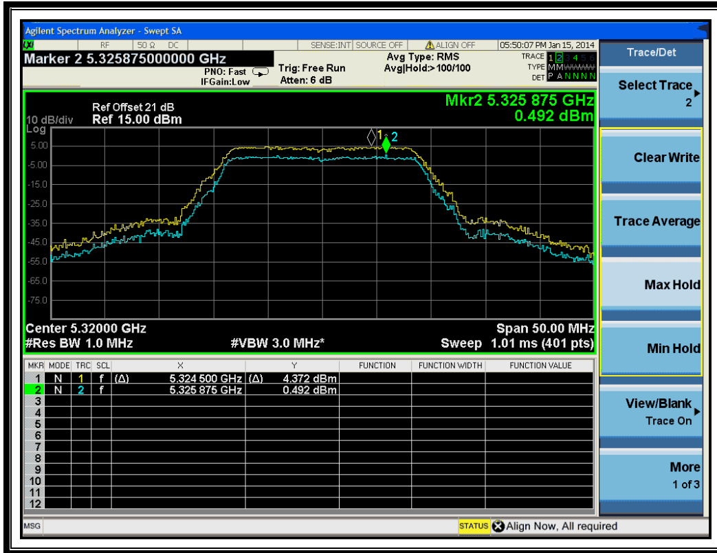
(Channel 64: 5320MHz @ 802.11n-20MHz)
