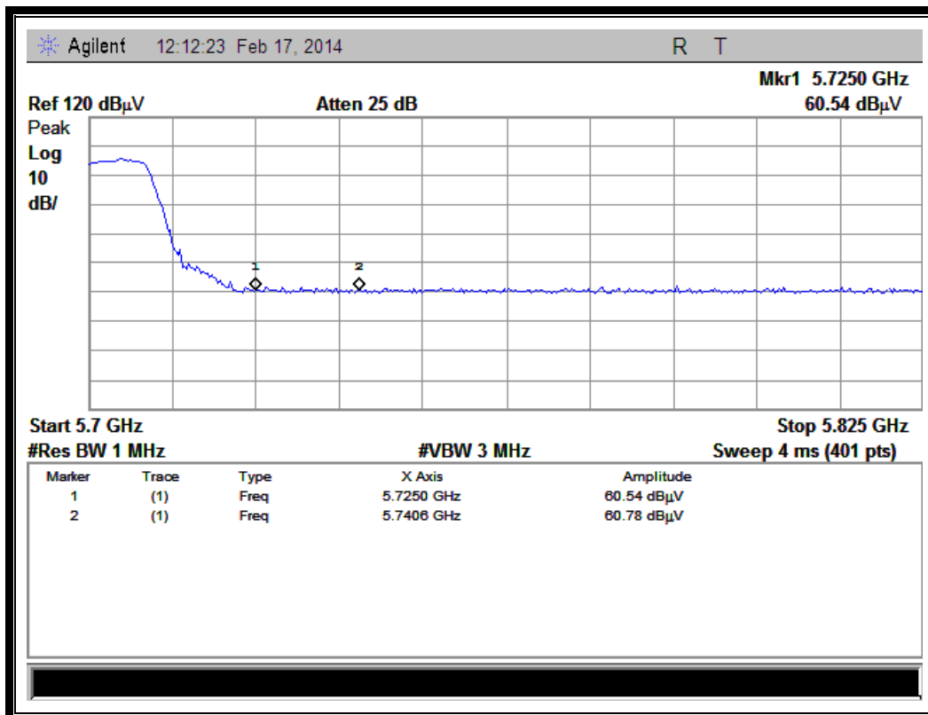
(Channel = 140 PEAK @ 802.11n-20MHz)
