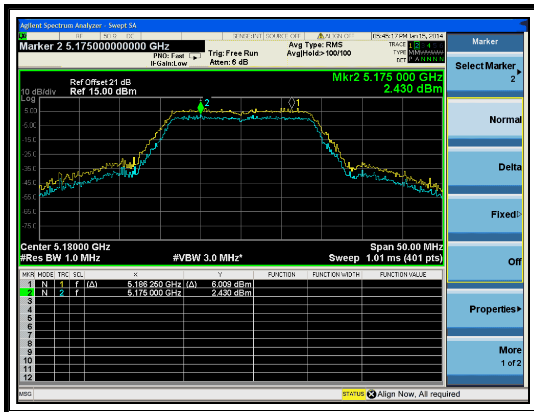
(Channel 36: 5180MHz @ 802.11n-20MHz)
