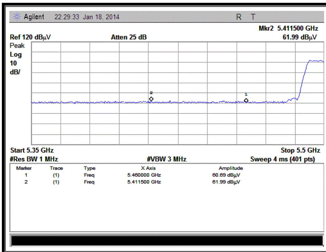
(Channel = 100 PEAK @ 802.11ac-20MHz)
