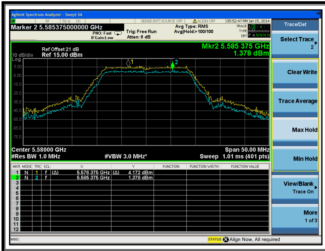
(Channel 116: 5580 MHz @ 802.11n-20MHz)
