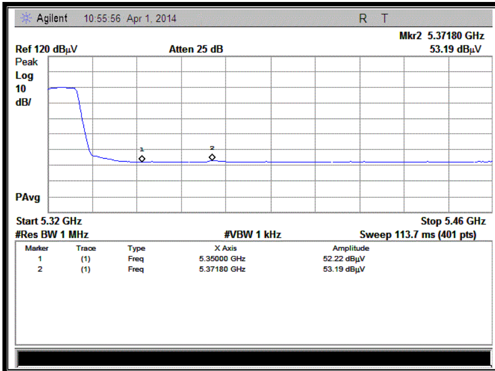
(Channel = 64 AVG @ 802.11ac-20MHz)
