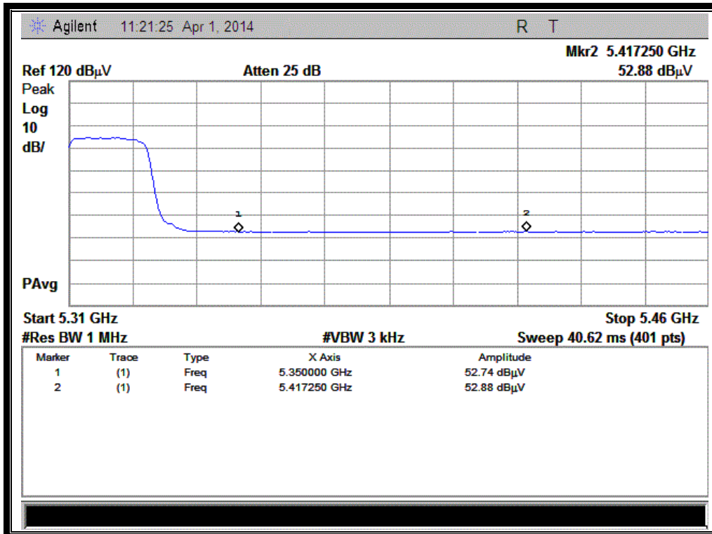
(Channel = 62 AVG @ 802.11 ac-40MHz)
