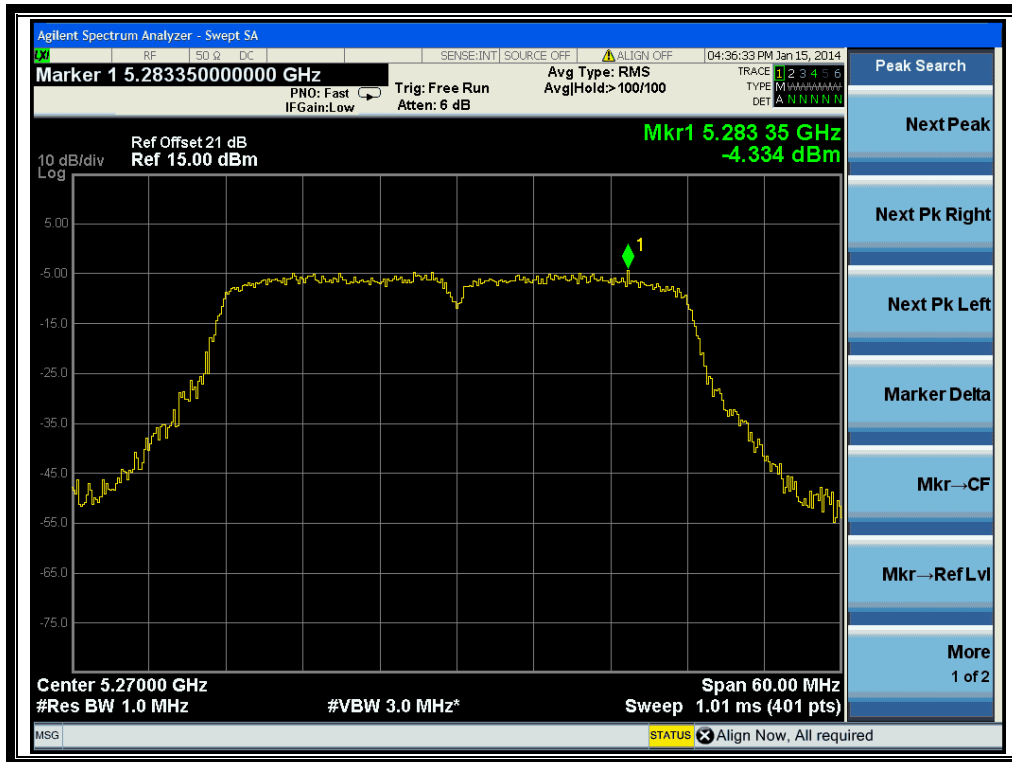
(Channel 54: 5270MHz @ 802.11ac-40MHz)
