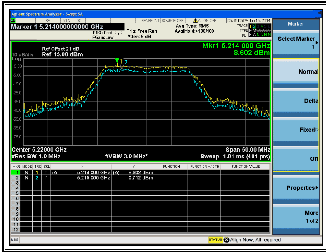
(Channel 44: 5220 MHz @ 802.11n-20MHz)
