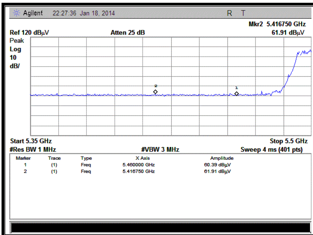
(Channel = 102 PEAK @ 802.11ac-40MHz)
