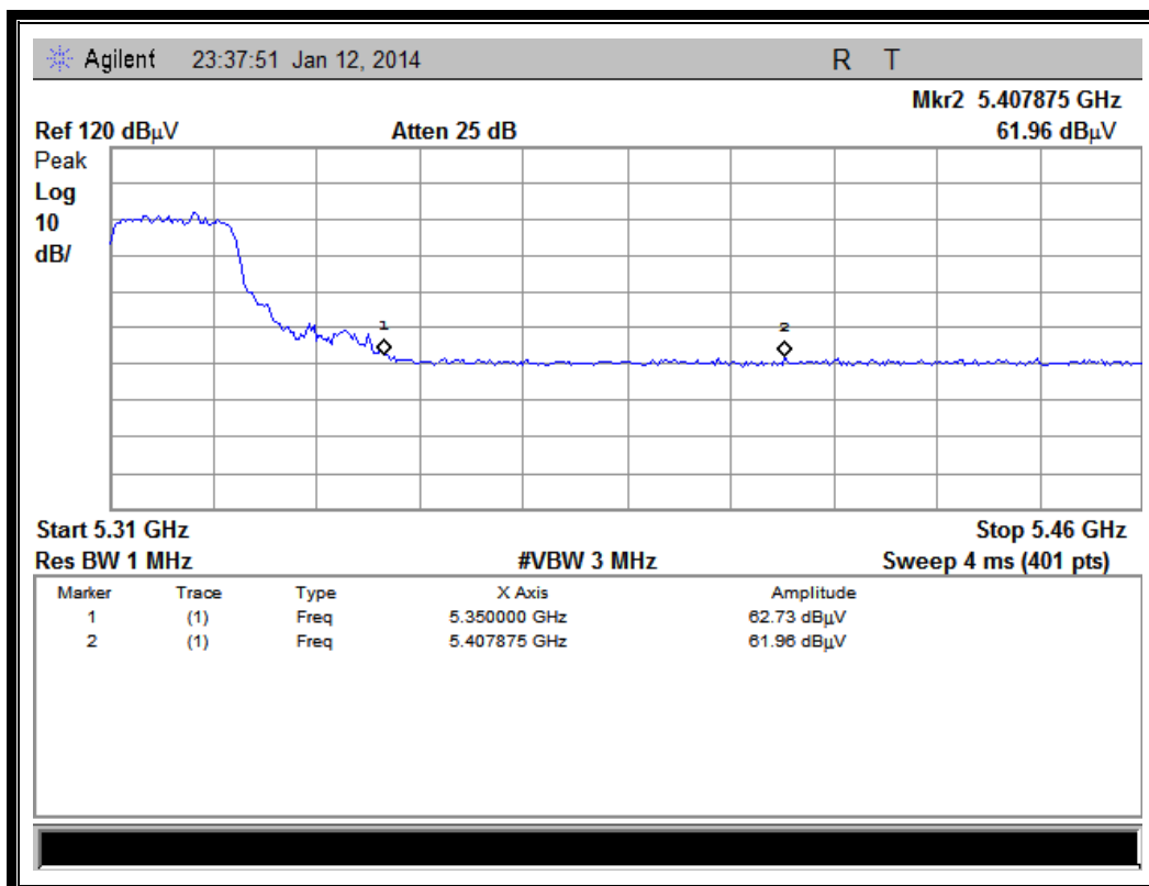
(Channel = 62 PEAK @ 802.11 ac-40MHz)
