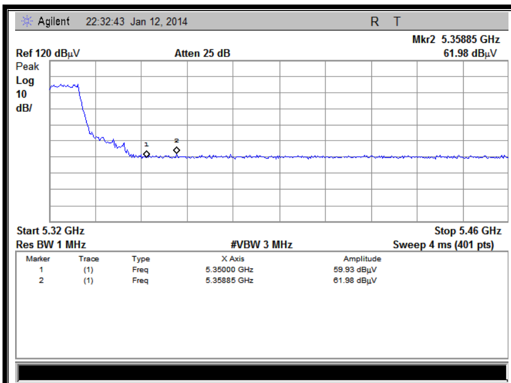
(Channel = 64 PEAK @ 802.11n-20MHz)
