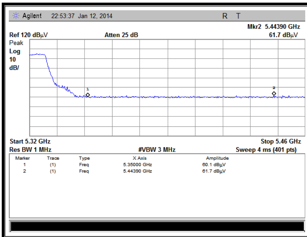
(Channel = 64 PEAK @ 802.11a)
