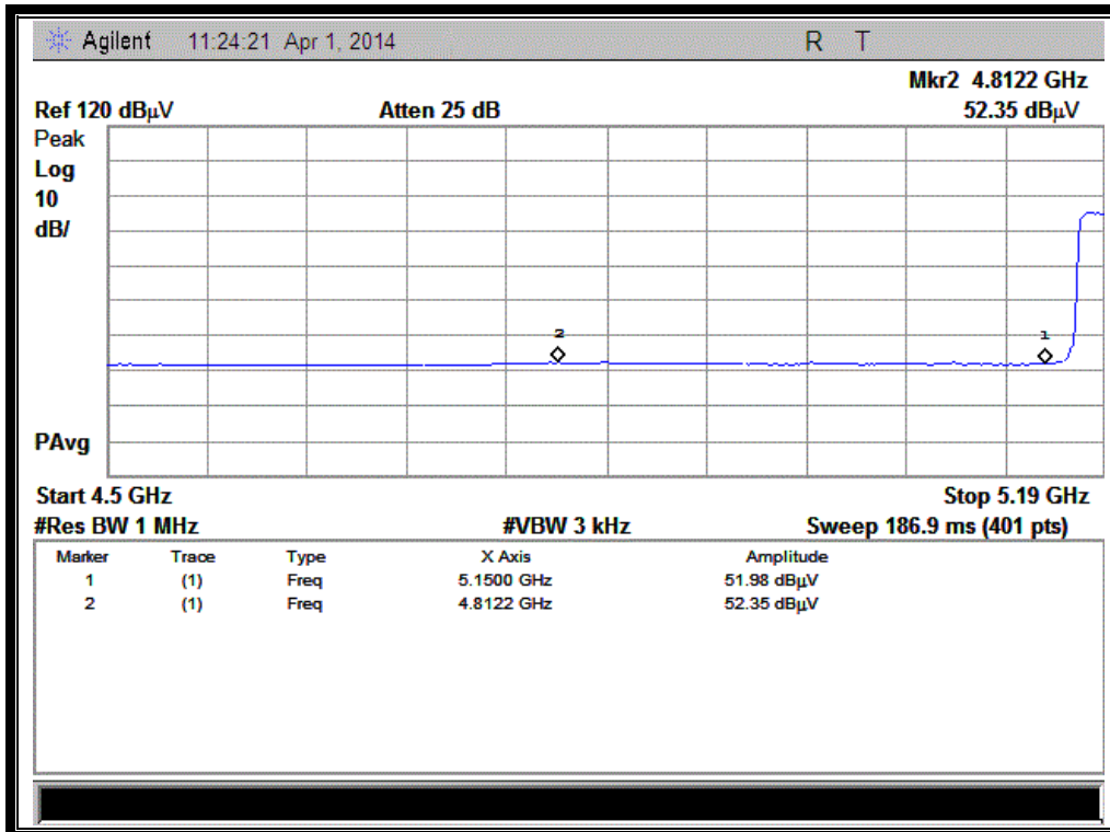
(Channel = 38 AVG @ 802.11ac-40MHz)
