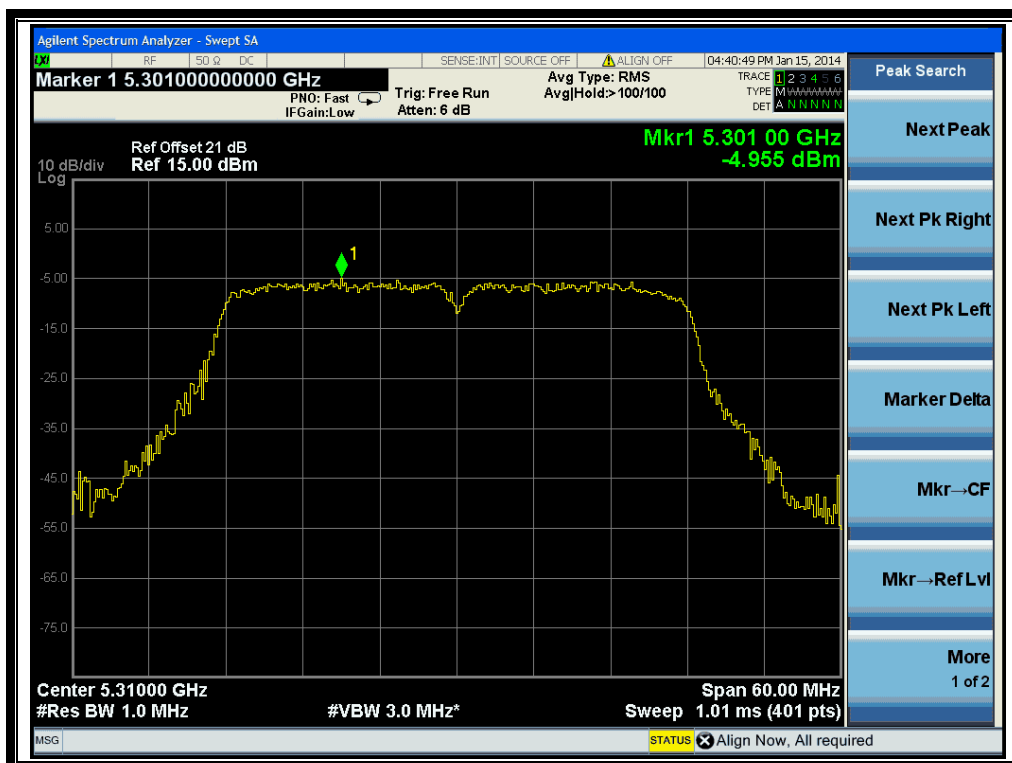
(Channel 62: 5310MHz @ 802.11ac-40MHz)
