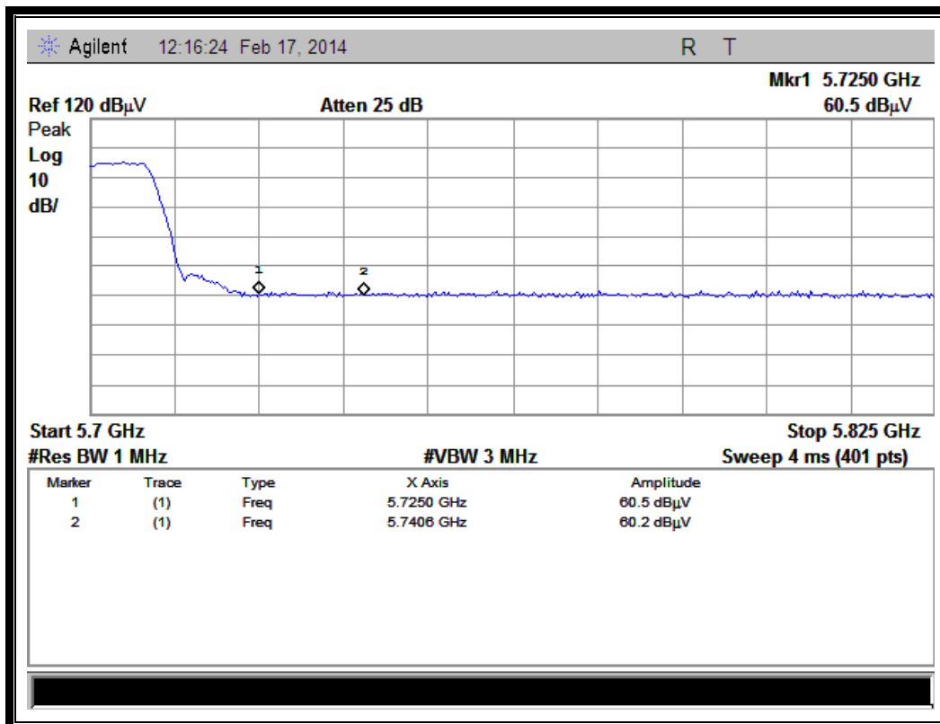
(Channel = 140 PEAK @ 802.11ac-20MHz)
