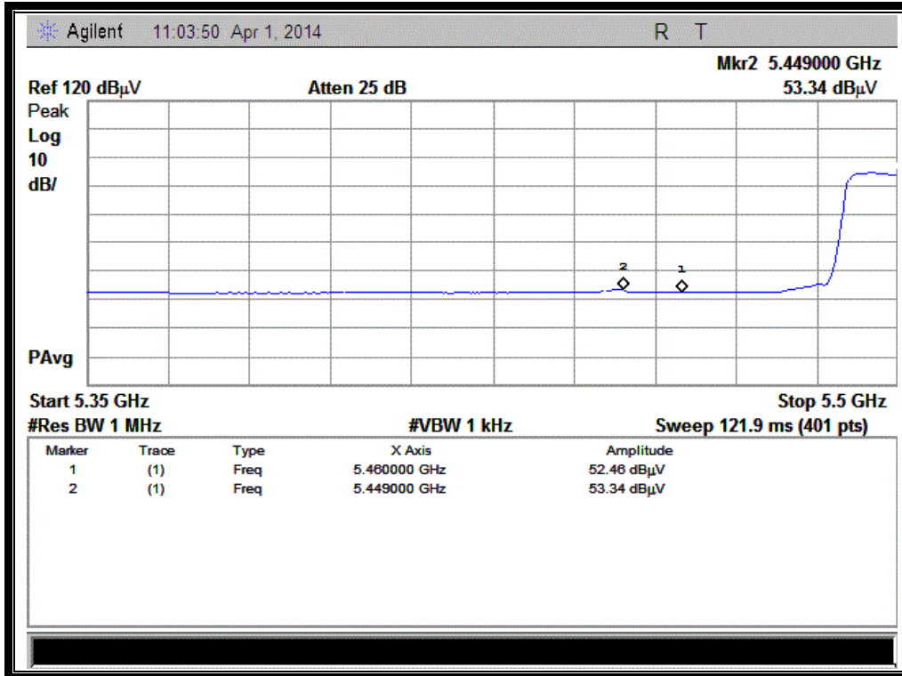
(Channel = 100 AVG @ 802.11ac-20MHz)
