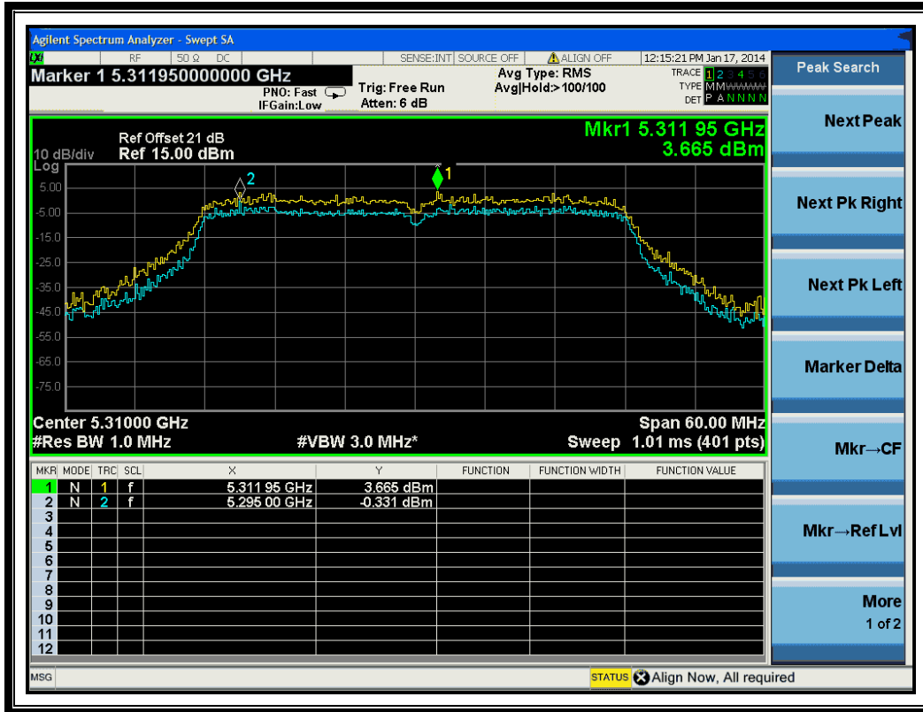
(Channel 62: 5310MHz @ 802.11n-40MHz)
