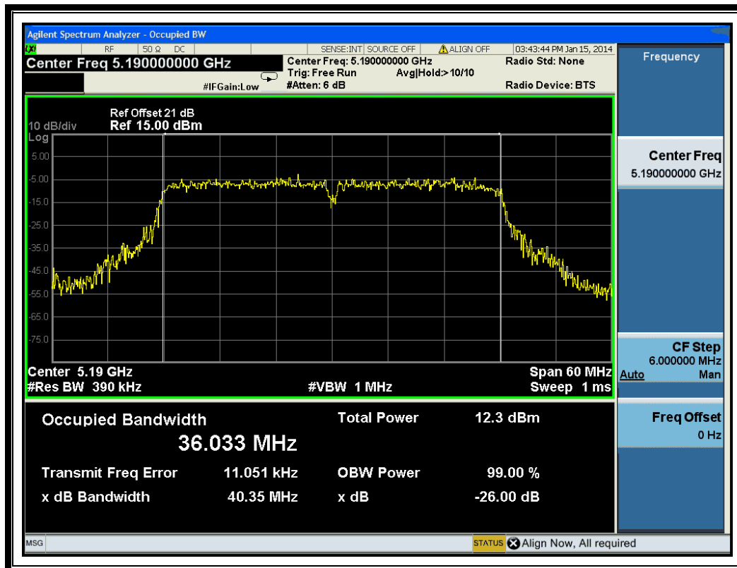
(Channel 38: 5190MHz @ 802.11n-40MHz)
