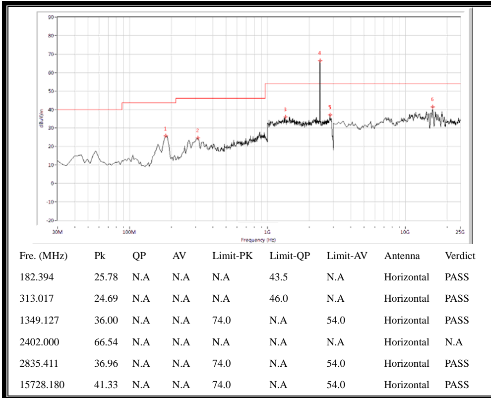
(Plot A.2: Antenna Horizontal, 30MHz to 25GHz)
