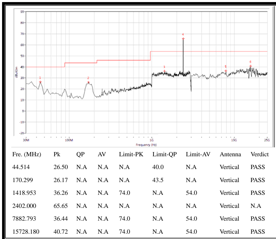
(Plot A.3: Antenna Vertical, 30MHz to 25GHz)
