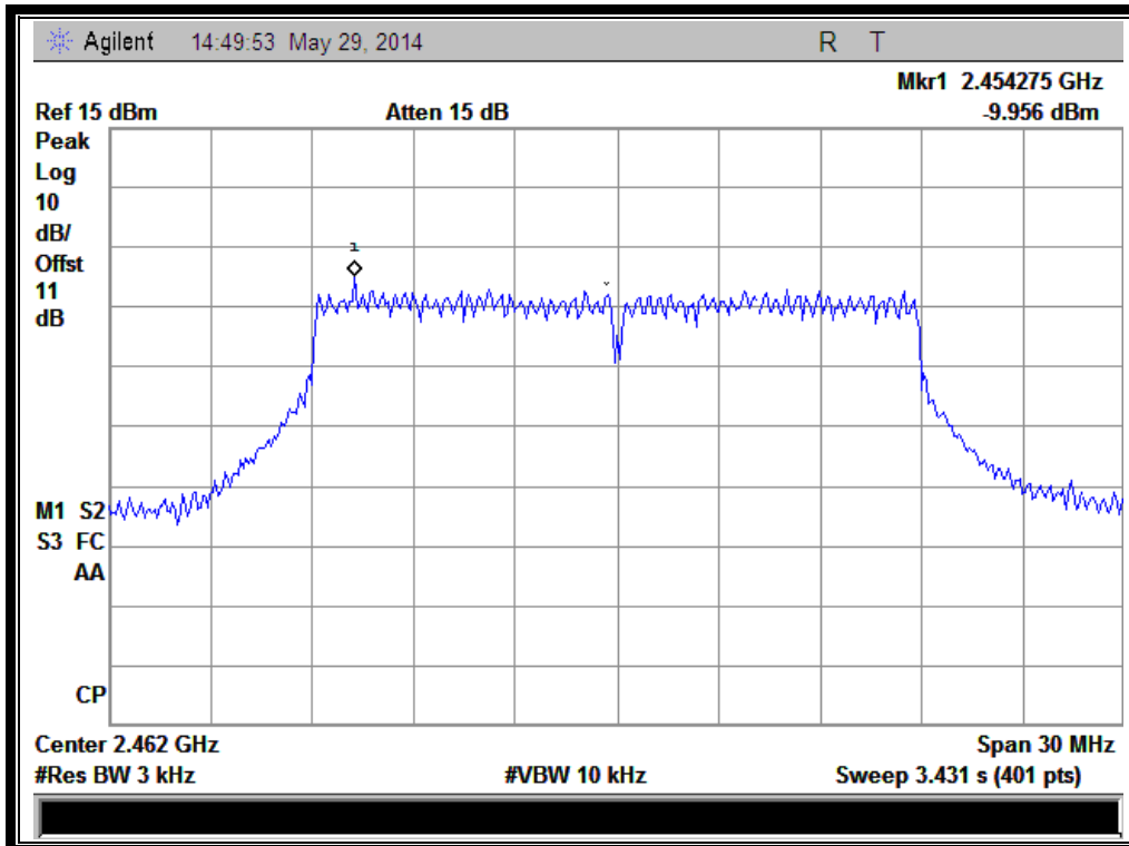
(Plot I: Channel = 11 @ 802.11n-20MHz)
