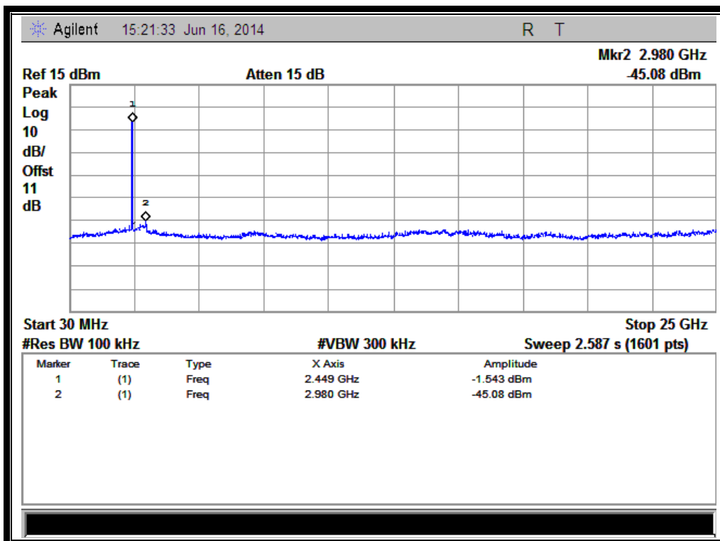
(Plot E.1: Channel = 6, 30MHz to 25GHz)
