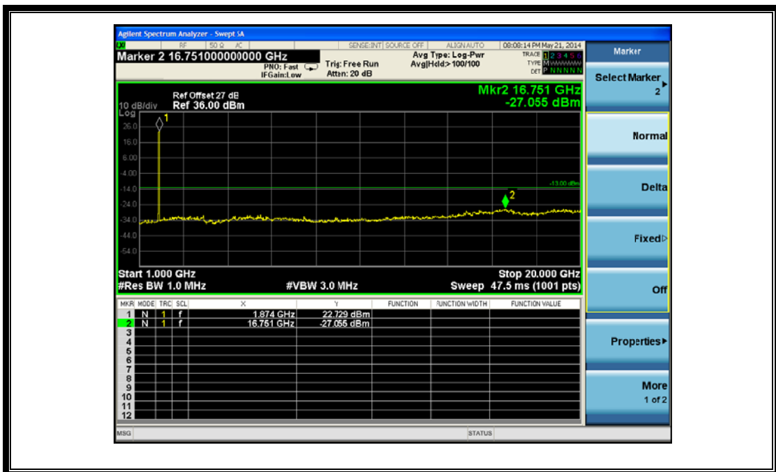
(Plot L2.1: HSPA+1900MHz Channel = 9400, 1GHz to 20GHz)
