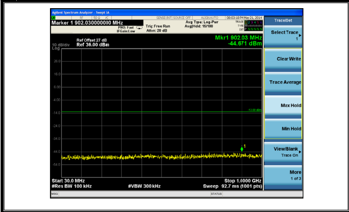
(Plot L 2: HSPA+1900MHz Channel = 9400, 30MHz to 1GHz)
