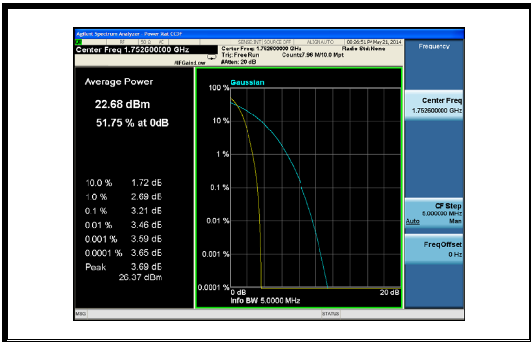
(Plot D3: WCDMA 1700MHz Channel = 1513)
