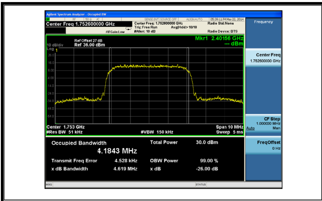
(Plot V1: HSPA+1700 MHz Channel = 1513)
