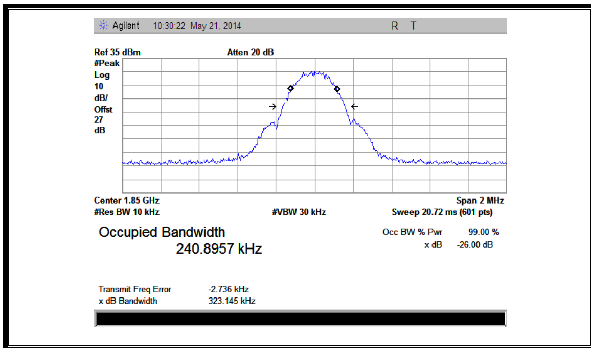
(Plot Z1:GPRS 1900MHz Channel = 512)
