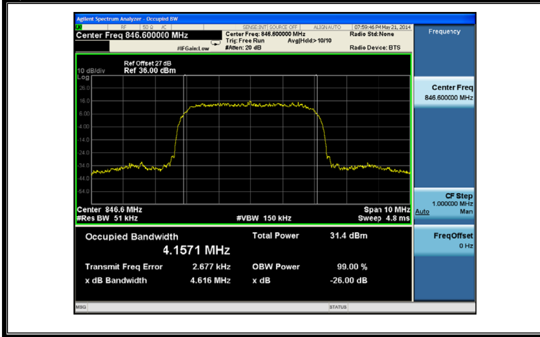
(Plot A1:HSPA+ 850 MHz Channel = 4233)
