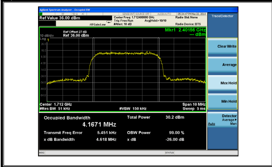
(Plot K1: WCDMA 1700MHz Channel = 1312)
