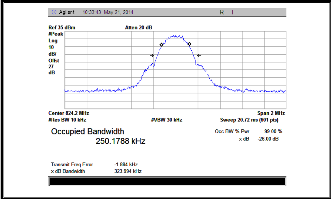
(Plot W1: GPRS 850MHz Channel = 128)
