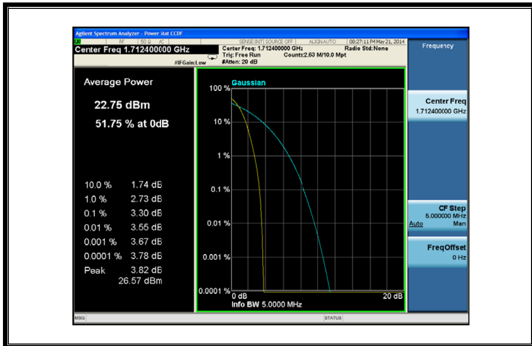
(Plot D1: WCDMA 1700MHz Channel = 1312)
