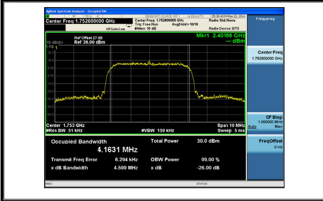
(Plot S1: HSUPA 1700 MHz Channel = 1513)
