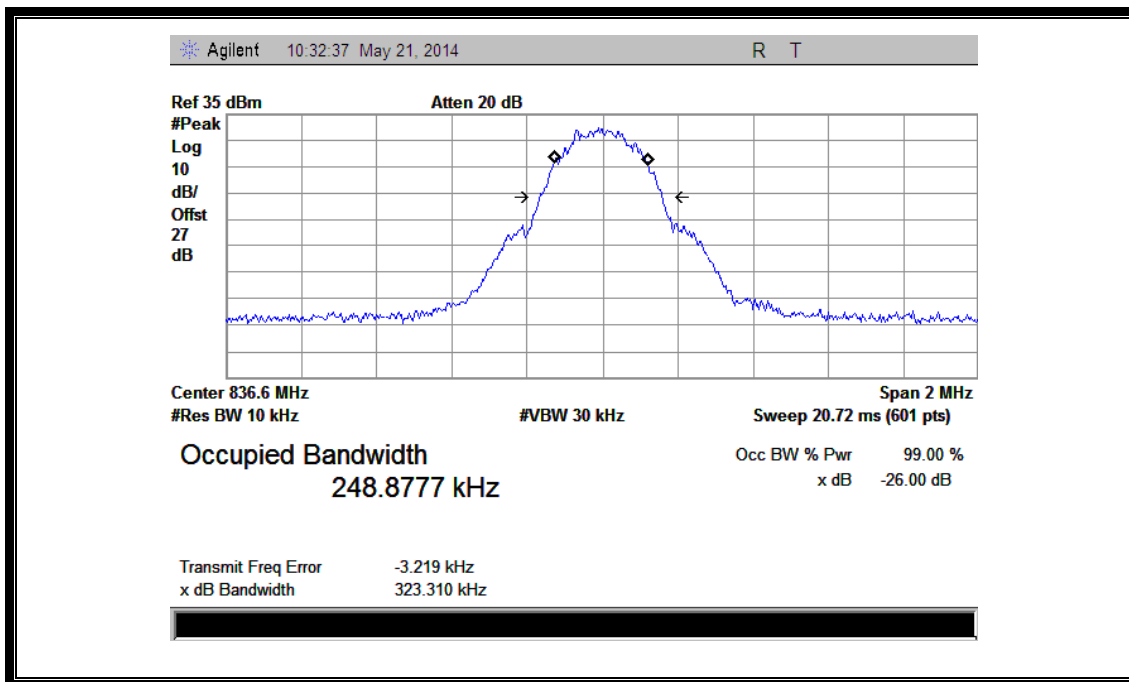
(Plot X1: GPRS 850MHz Channel = 190)
