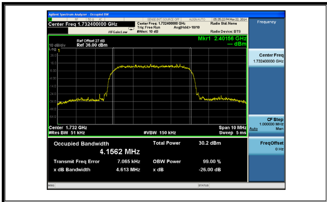
(Plot L1: WCDMA 1700 MHz Channel = 1412)
