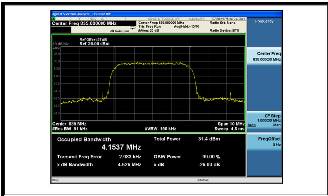
(Plot Z: HSPA+850 MHz Channel = 4175)
