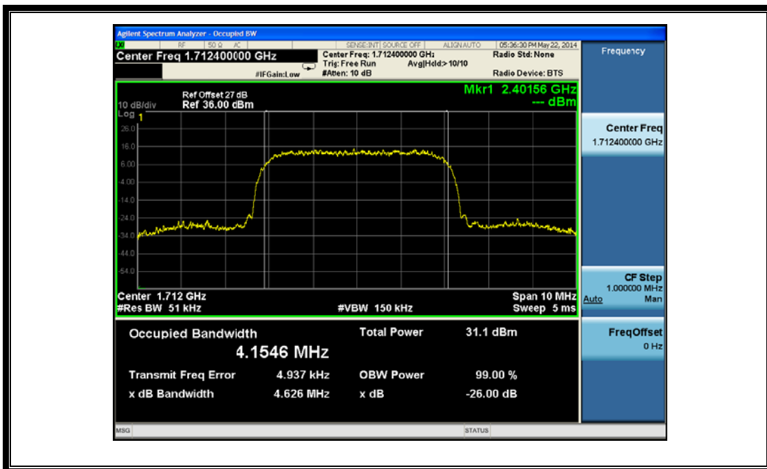
(Plot N1: HSDPA 1700MHz Channel = 1312)
