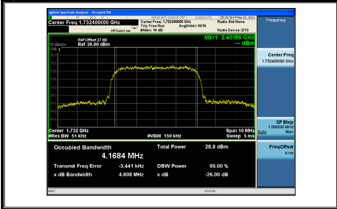
(Plot U1: HSPA+1700 MHz Channel = 1412)
