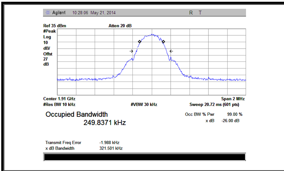
(Plot B2: GPRS 1900MHz Channel = 810)
