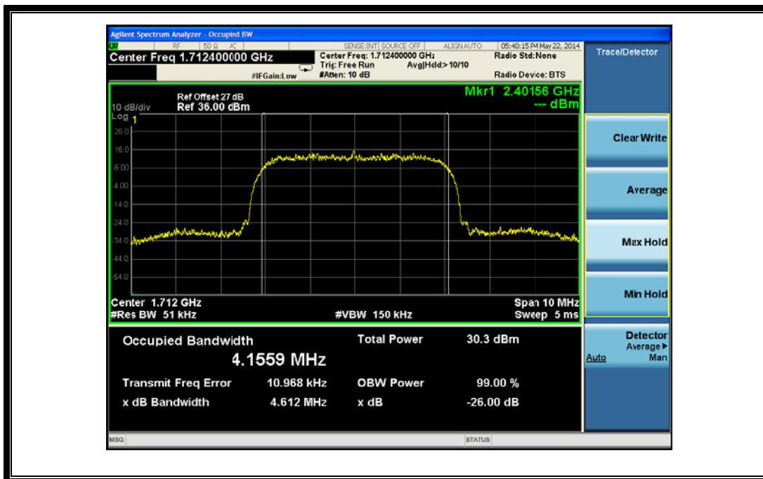
(Plot T1:HSPA+1700 MHz Channel = 1312)
