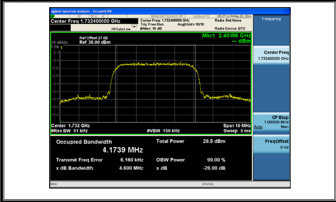
(Plot O1: HSDPA 1700 MHz Channel = 1412)
