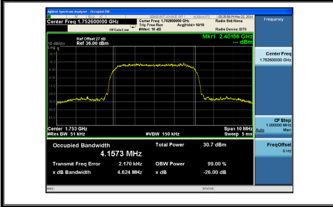
(Plot M1: WCDMA 1700MHz Channel = 1513)
