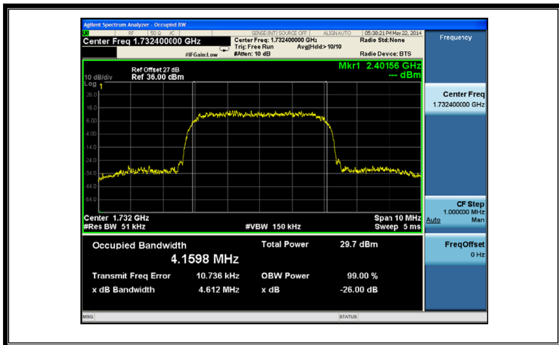
(Plot R1: HSUPA1700 MHz Channel = 1412)
