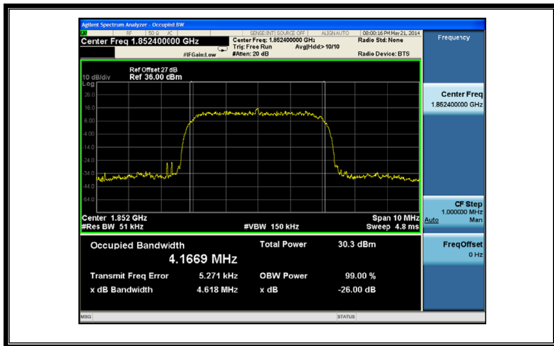
(Plot B1: HSPA+1900 MHz Channel = 9262)
