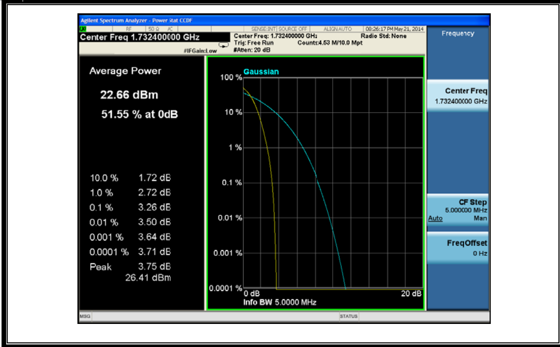
(Plot D2: WCDMA 1700MHz Channel = 1412)
