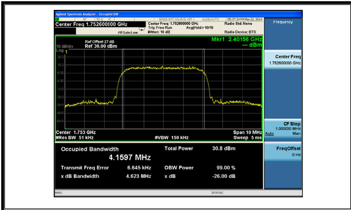
(Plot P1: HSDPA 1700MHz Channel = 1513)
