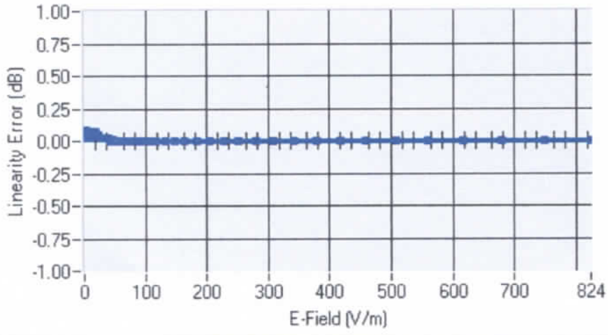
Linearity
