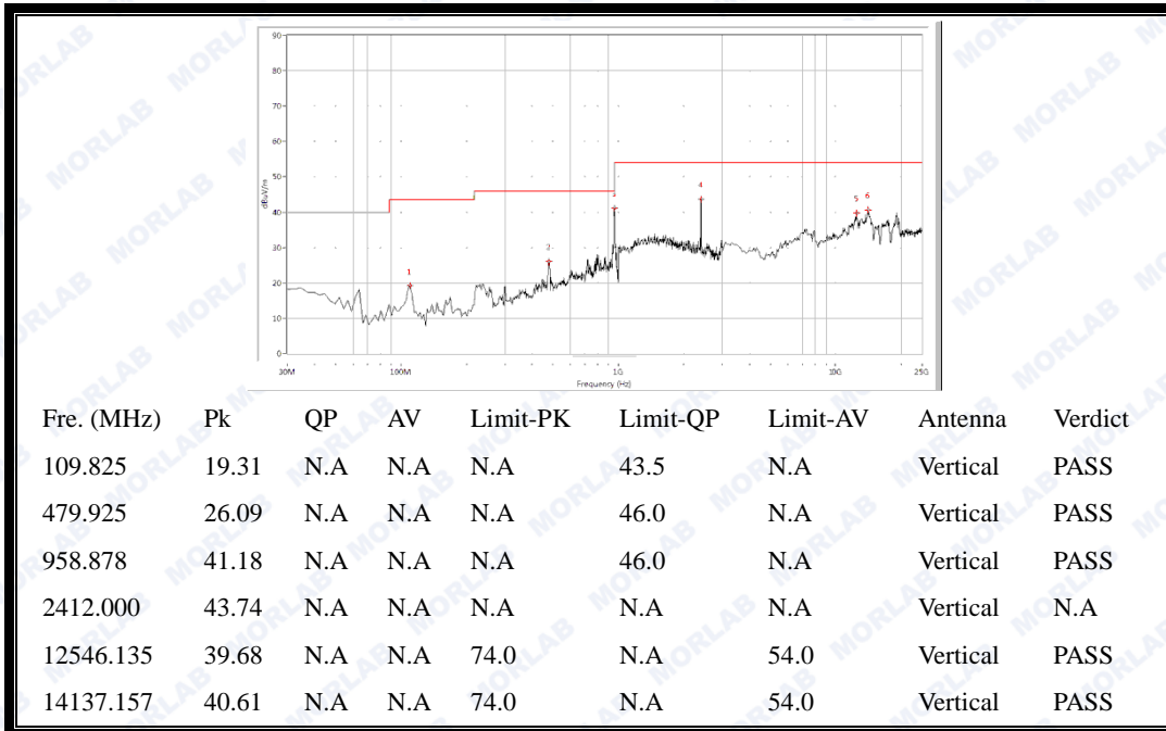
(Antenna Vertical, 30MHz to 25GHz)
