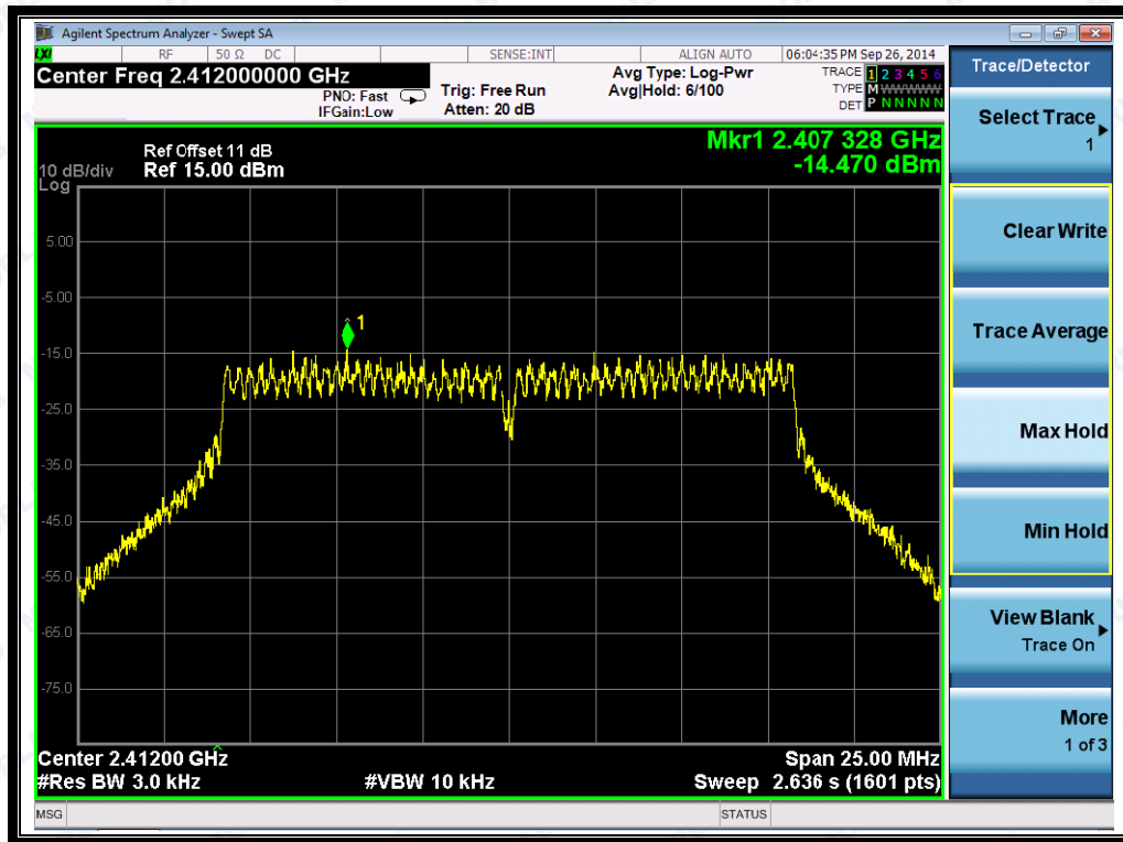
(Channel = 1 @ 802.11g)
