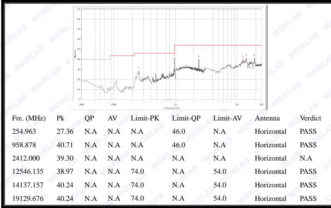
(Antenna Horizontal, 30MHz to 25GHz)
