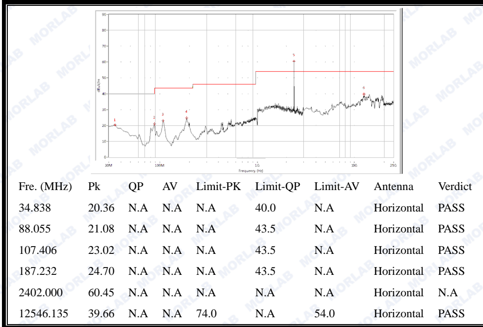
(30MHz to 25GHz, Antenna Horizontal @ GFSK, channel 0)
