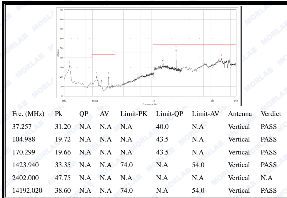
(30MHz to 25GHz, Antenna Vertical @8-DPSK, channel 0)
