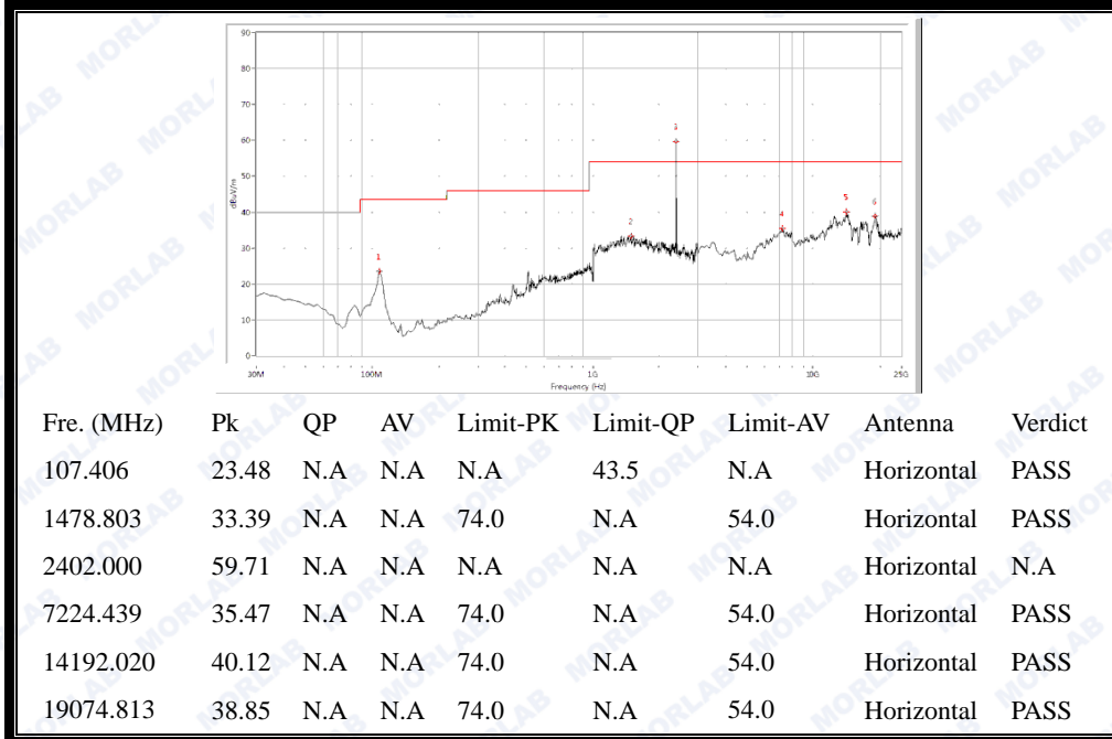
(30MHz to 25GHz, Antenna Horizontal @ \pi/4 -DQPSK, channel 0)
