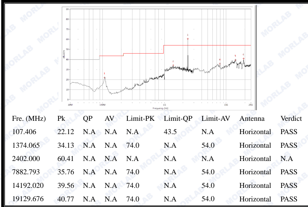
(30MHz to 25GHz, Antenna Horizontal @8-DPSK, channel 0)
