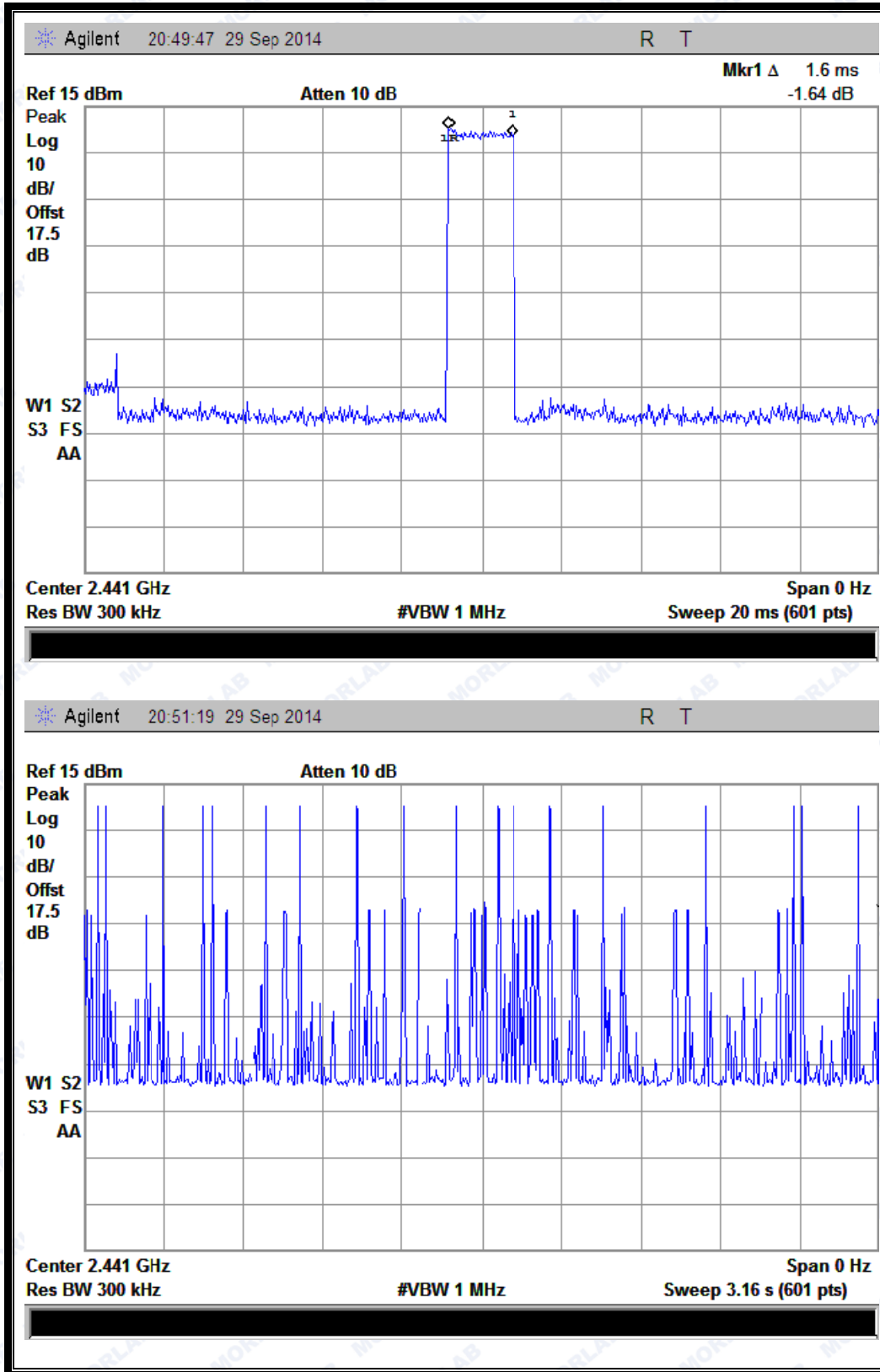
(Plot H: DH3 @ 8-DPSK)
