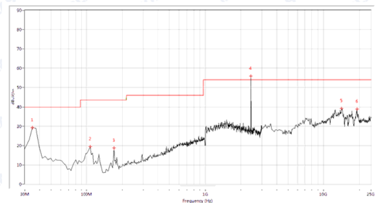
(30MHz to 25GHz, Antenna Horizontal @ \pi/4 -DQPSK, channel 39)
