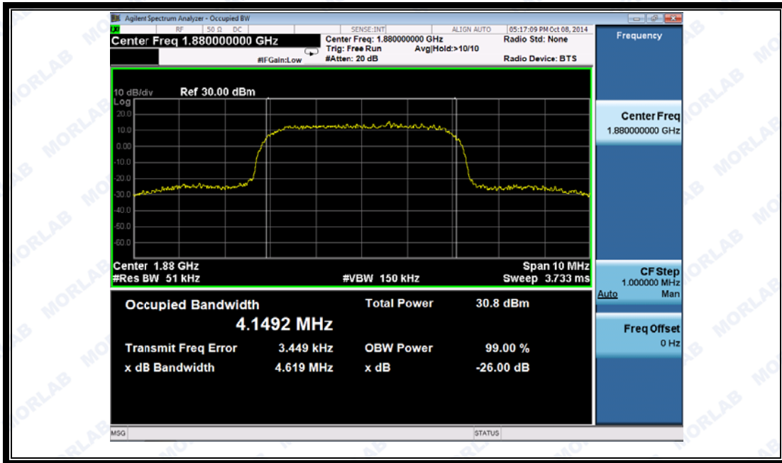
(Plot W: HSUPA1900 MHz Channel = 9400)
