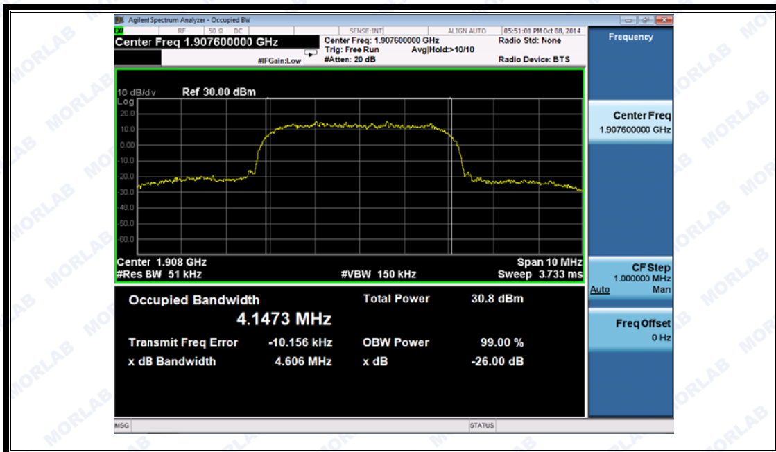
(Plot D1: HSPA+1900 MHz Channel = 9538)
