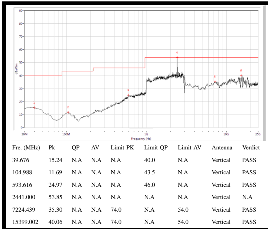
(30MHz to 25GHz, Antenna Vertical @8-DPSK, channel 39)
