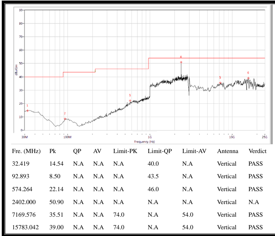
(30MHz to 25GHz, Antenna Vertical @ GFSK, channel 0)
