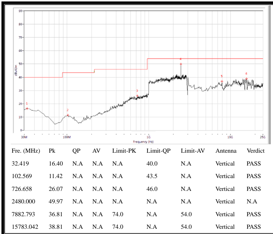
(30MHz to 25GHz, Antenna Vertical @ \pi/4 -DQPSK, channel 78)
