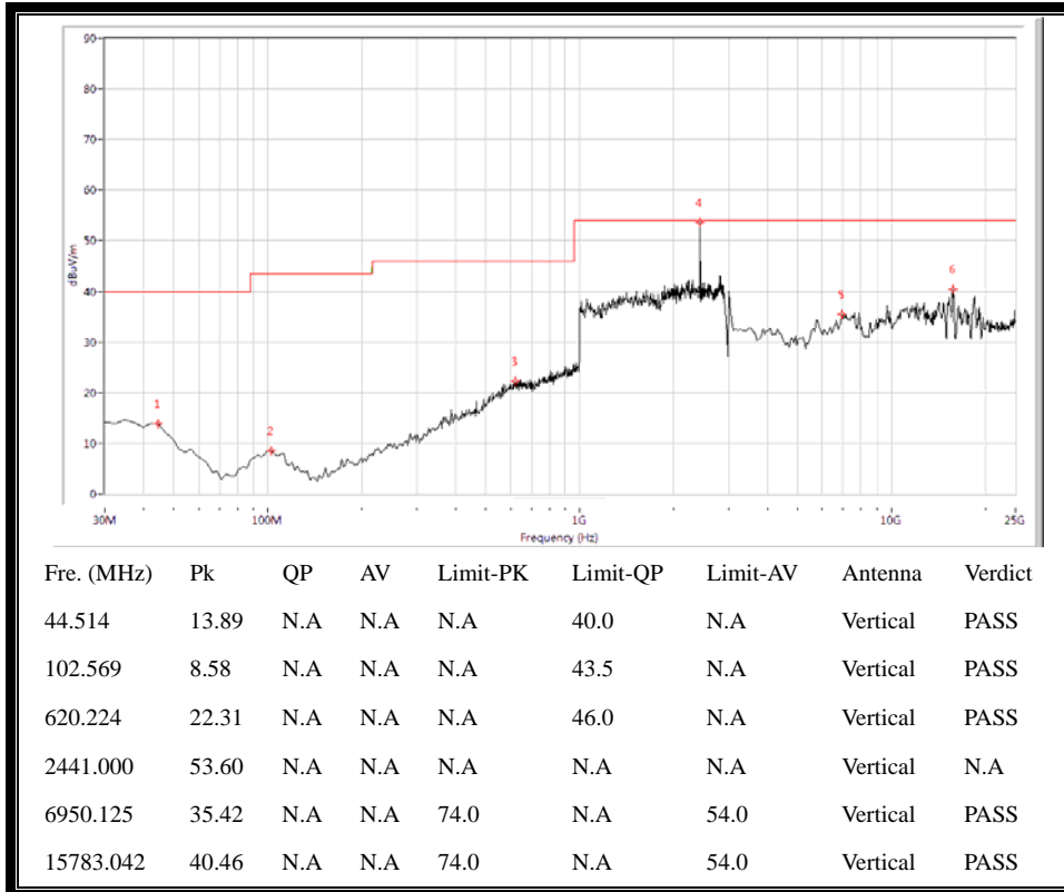
(30MHz to 25GHz, Antenna Vertical @ GFSK, channel 39)
