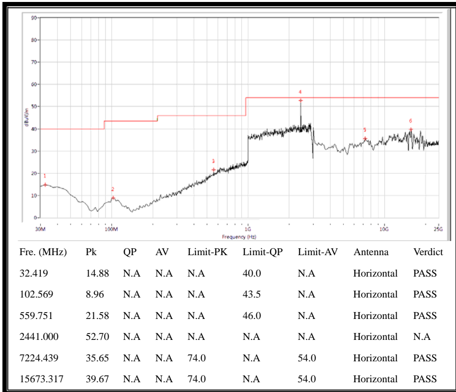
(30MHz to 25GHz, Antenna Horizontal @ \pi/4 -DQPSK, channel 39)
