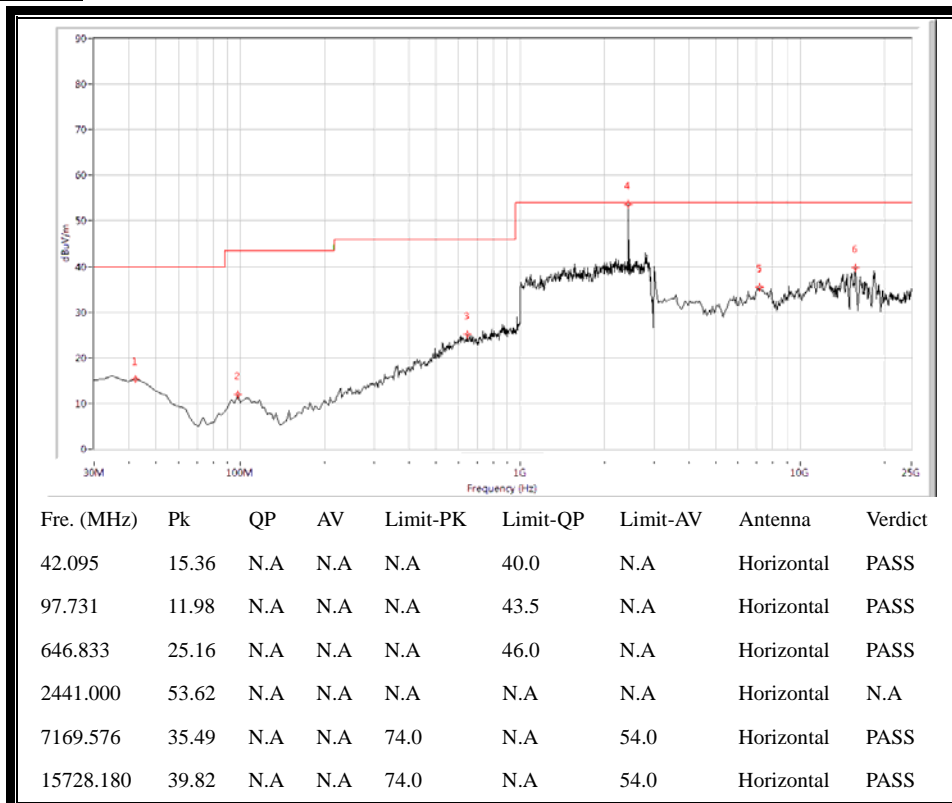
(30MHz to 25GHz, Antenna Horizontal @ GFSK, channel 39)
