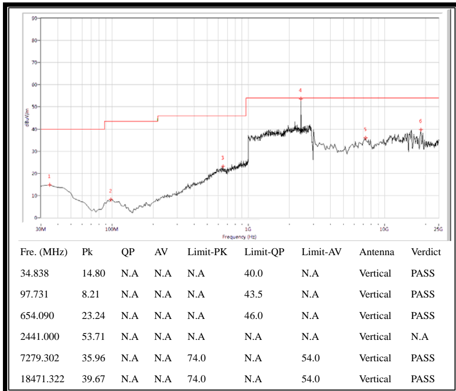
(30MHz to 25GHz, Antenna Vertical @ \pi/4 -DQPSK, channel 39)
