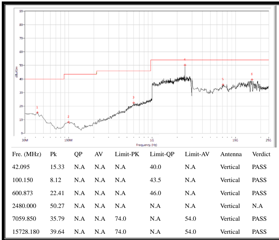
(30MHz to 25GHz, Antenna Vertical @ GFSK, channel 78)
