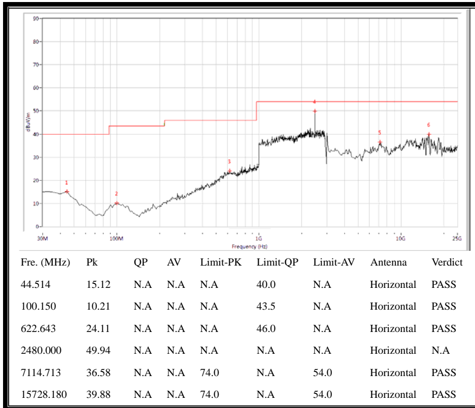
(30MHz to 25GHz, Antenna Horizontal @8-DPSK, channel 78)
