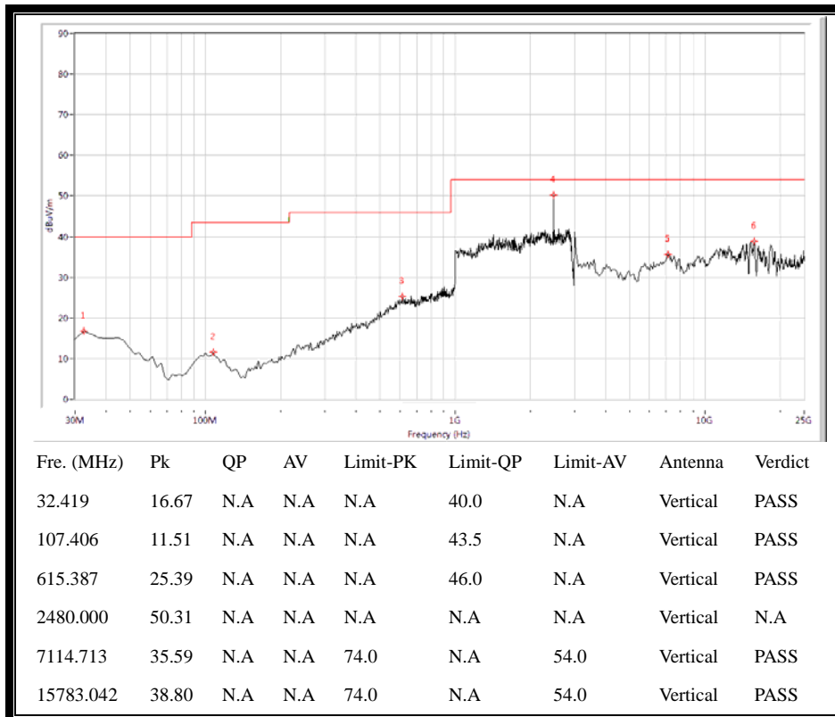
(30MHz to 25GHz, Antenna Vertical @8-DPSK, channel 78)
