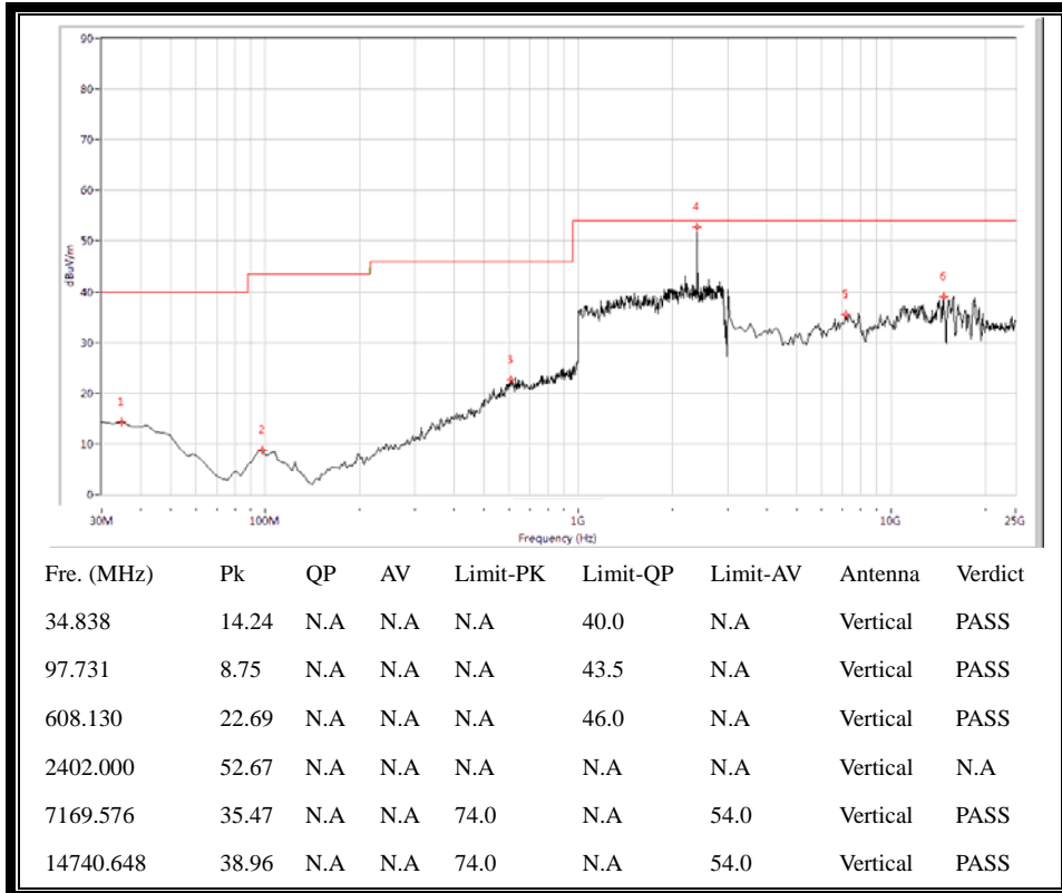
(30MHz to 25GHz, Antenna Vertical @8-DPSK, channel 0)
