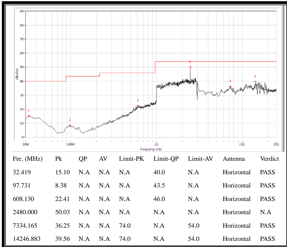
(30MHz to 25GHz, Antenna Horizontal @ \pi/4 -DQPSK, channel 78)
