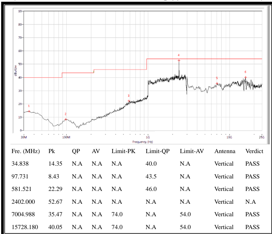
(30MHz to 25GHz, Antenna Vertical @ \pi/4 -DQPSK, channel 0)
