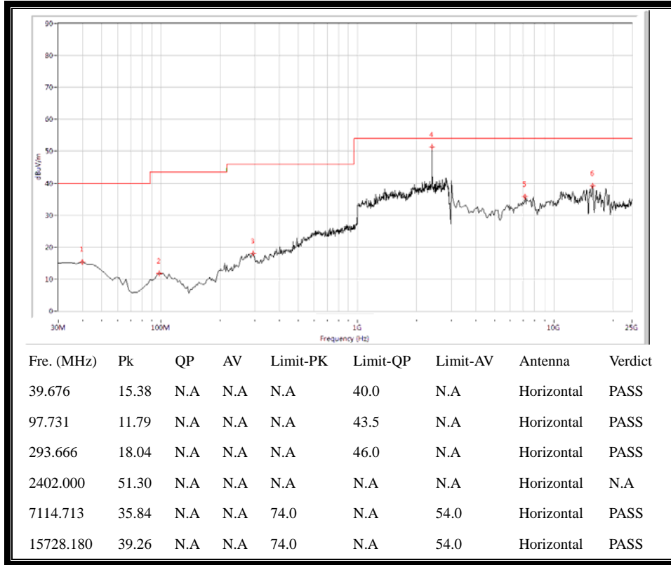
(30MHz to 25GHz, Antenna Horizontal @8-DPSK, channel 0)
