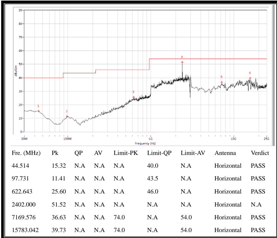
(30MHz to 25GHz, Antenna Horizontal @ \pi/4 -DQPSK, channel 0)
