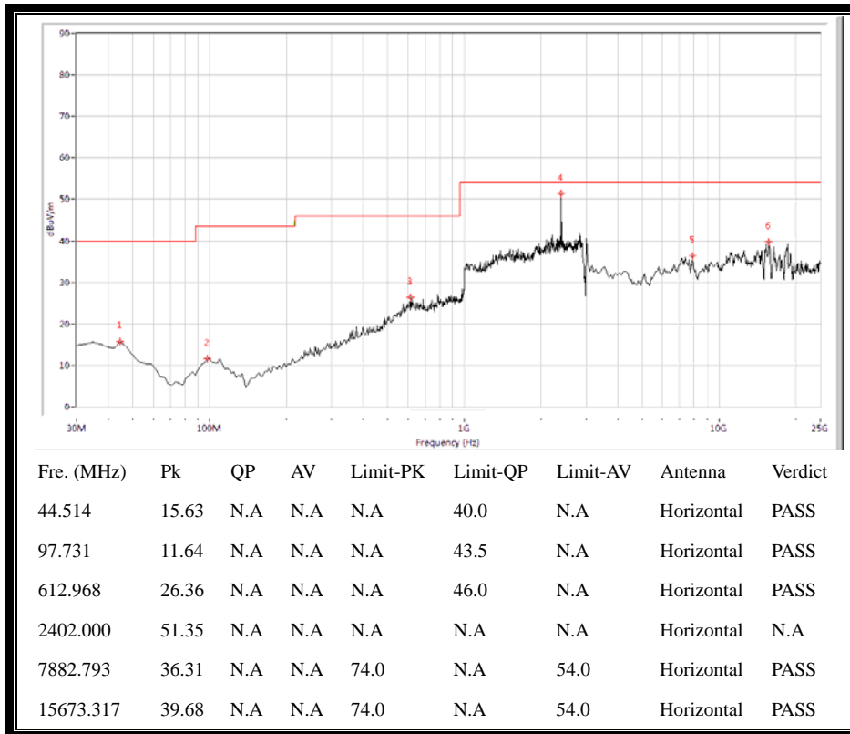
(30MHz to 25GHz, Antenna Horizontal @ GFSK, channel 0)
