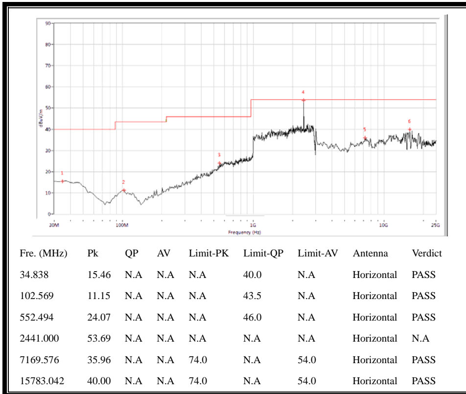
(30MHz to 25GHz, Antenna Horizontal @8-DPSK, channel 39)
