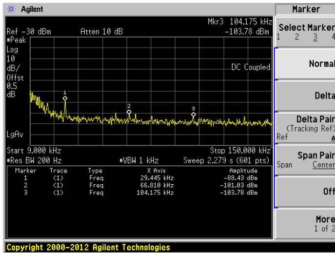
MIDDLE CHANNEL, SPURIOUS 9 kHz ~ 150 kHz
