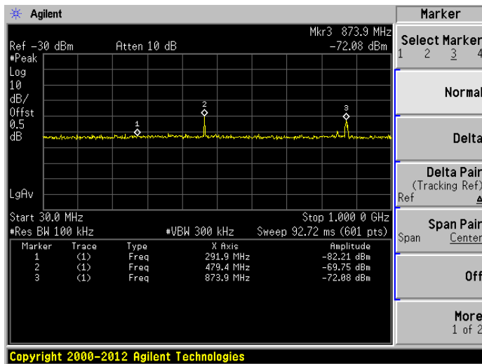
MIDDLE CHANNEL, SPURIOUS 30 MHz ~ 1 GHz
