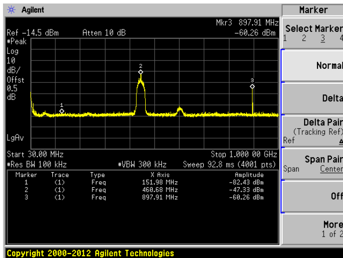
HIGH CHANNEL, SPURIOUS 30 MHz ~ 1 GHz
