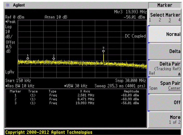
HIGH CHANNEL, SPURIOUS 150 kHz ~ 30 MHz
