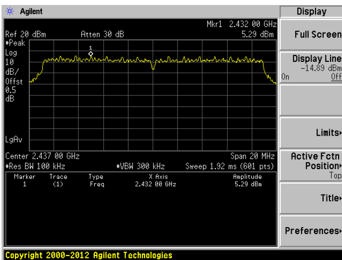
802.11n-20 MHz MIDDLE CHANNEL CARRIER LEVEL
