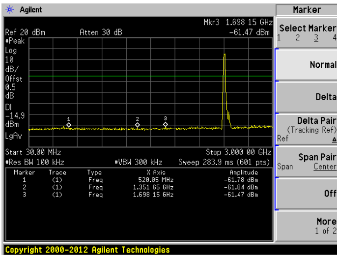
802.11n-20 MHz LOW CHANNEL, SPURIOUS 30 MHz ~ 3 GHz
