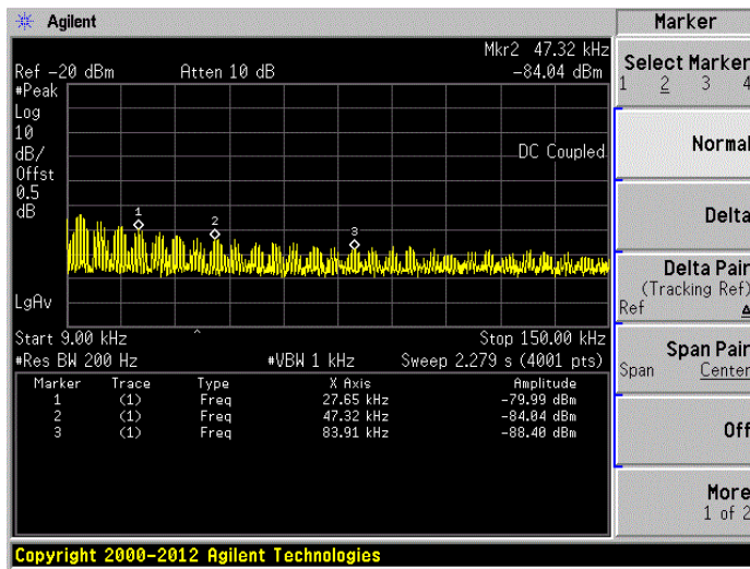
HIGH CHANNEL, SPURIOUS 9 kHz ~ 150 kHz
