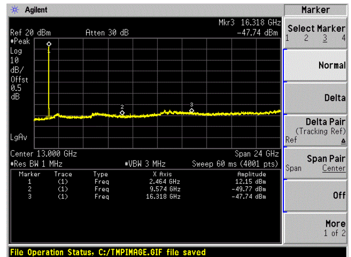
HIGH CHANNEL, SPURIOUS 1 GHz ~ 25 GHz
