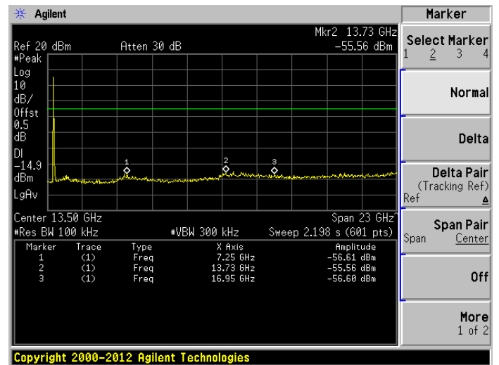
802.11n-20 MHz LOW CHANNEL, SPURIOUS 2 GHz ~ 25 GHz
