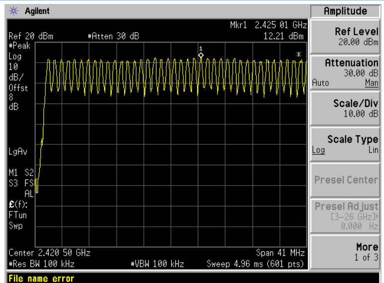
GFSK 2.4 GHz ~ 2.4415 GHz
