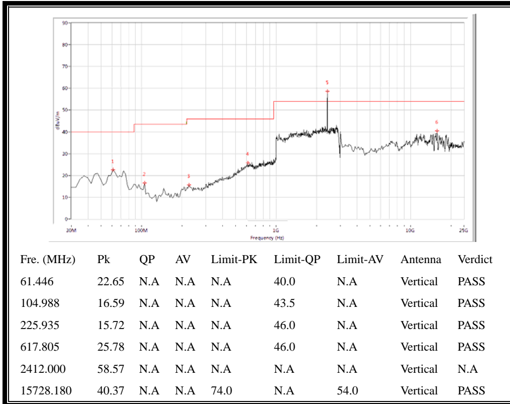
(Antenna Vertical, 30MHz to 25GHz)
