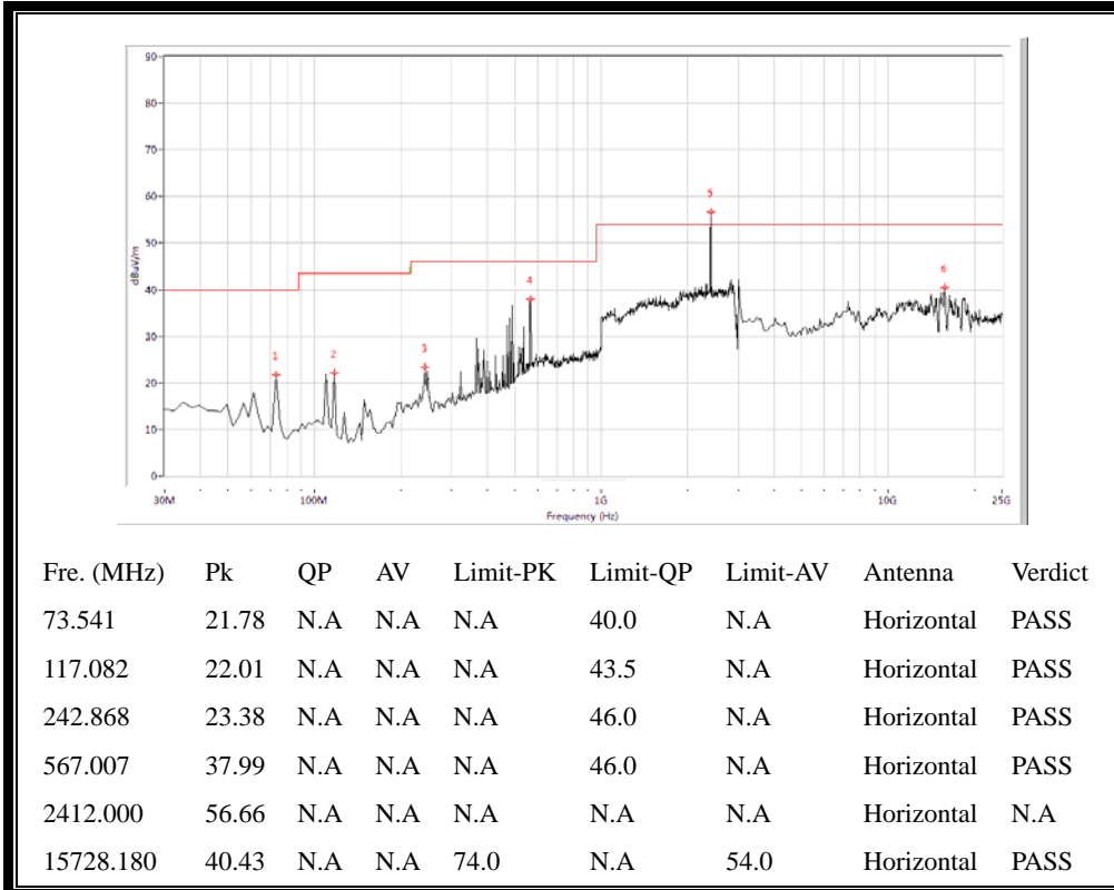
(Antenna Horizontal, 30MHz to 25GHz)
