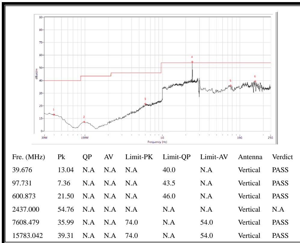
(Antenna Vertical, 30MHz to 25GHz)
