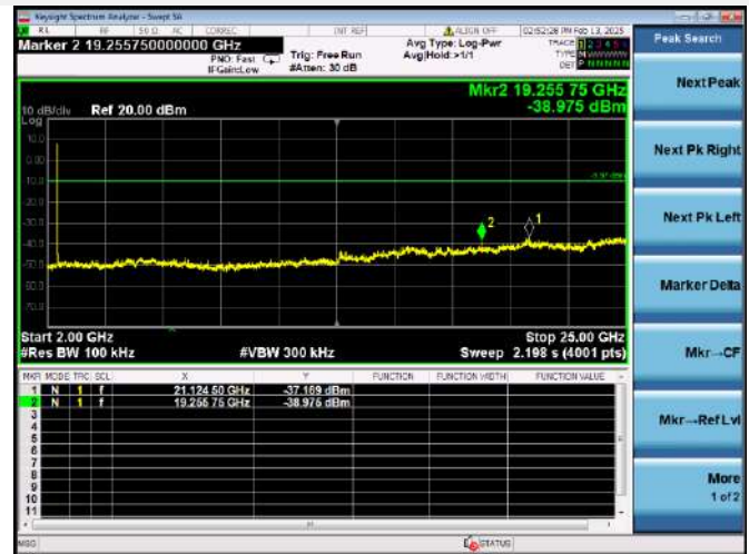
802.11b CHANNEL 2, SPURIOUS 2 GHz ~ 25 GHz
