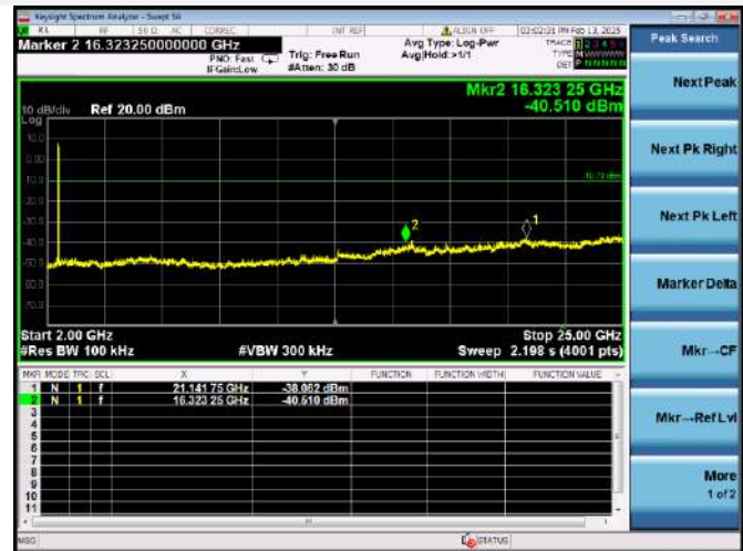
802.11b CHANNEL 11, SPURIOUS 2 GHz ~ 25 GHz
