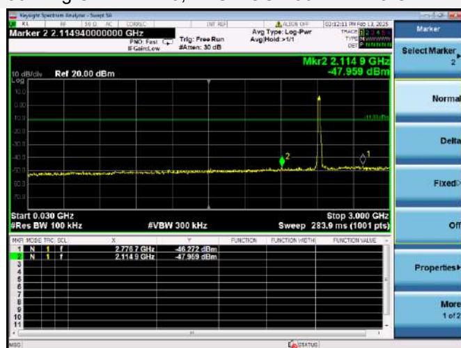
802.11g CHANNEL 3, SPURIOUS 30 MHz ~ 3 GHz
