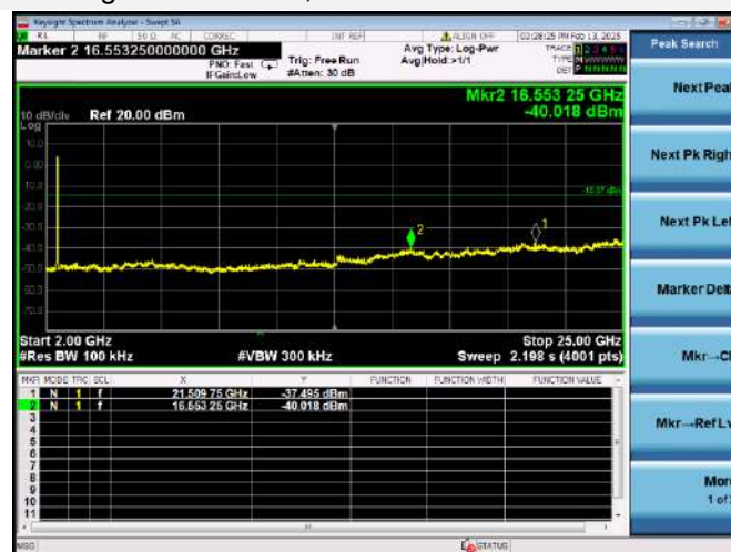
802.11g CHANNEL 11, SPURIOUS 2 GHz ~ 25 GHz
