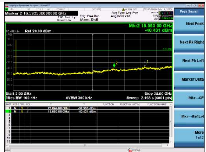
802.11b CHANNEL 6, SPURIOUS 2 GHz ~ 25 GHz
