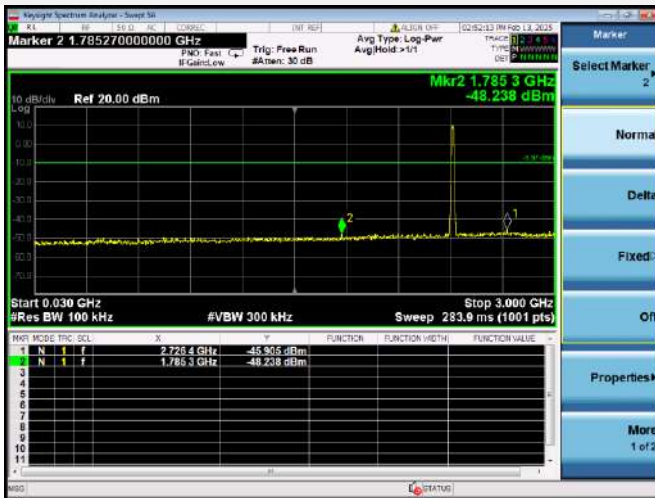
802.11b CHANNEL 2, SPURIOUS 30 MHz ~ 3 GHz
