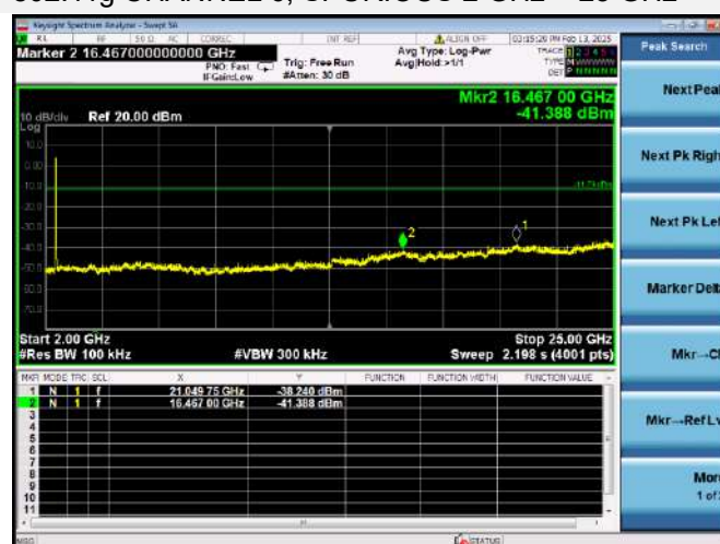
802.11g CHANNEL 6, SPURIOUS 2 GHz ~ 25 GHz
