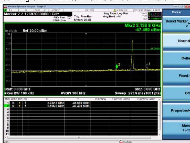
802.11g CHANNEL 6, SPURIOUS 30 MHz ~ 3 GHz
