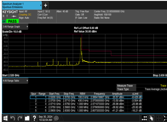
N7(20M)_DFT-s- OFDM_BPSK_Edge_1RB_Right_High_CH
