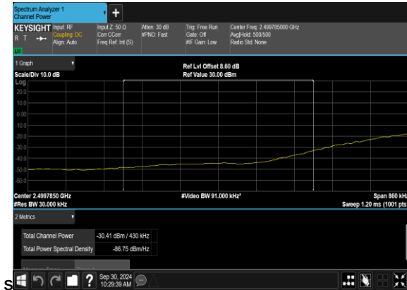
N7(20M)_DFT-s- OFDM_BPSK_Edge_1RB_Left_Low_CH_CHP_PAS
