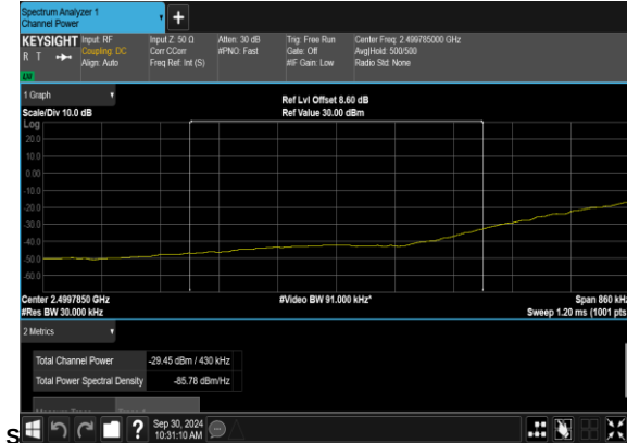
N7(20M)_DFT-s- OFDM_QPSK_Edge_1RB_Left_Low_CH_CHP_PAS
