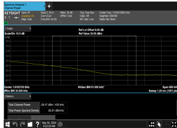
N2(40M)_DFT-s- OFDM_QPSK_Edge_1RB_Right_High_CH_CHP_P ASS
