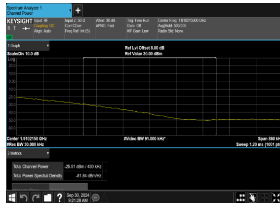
N2(40M)_DFT-s- OFDM_BPSK_Edge_1RB_Right_High_CH_CHP_P ASS
