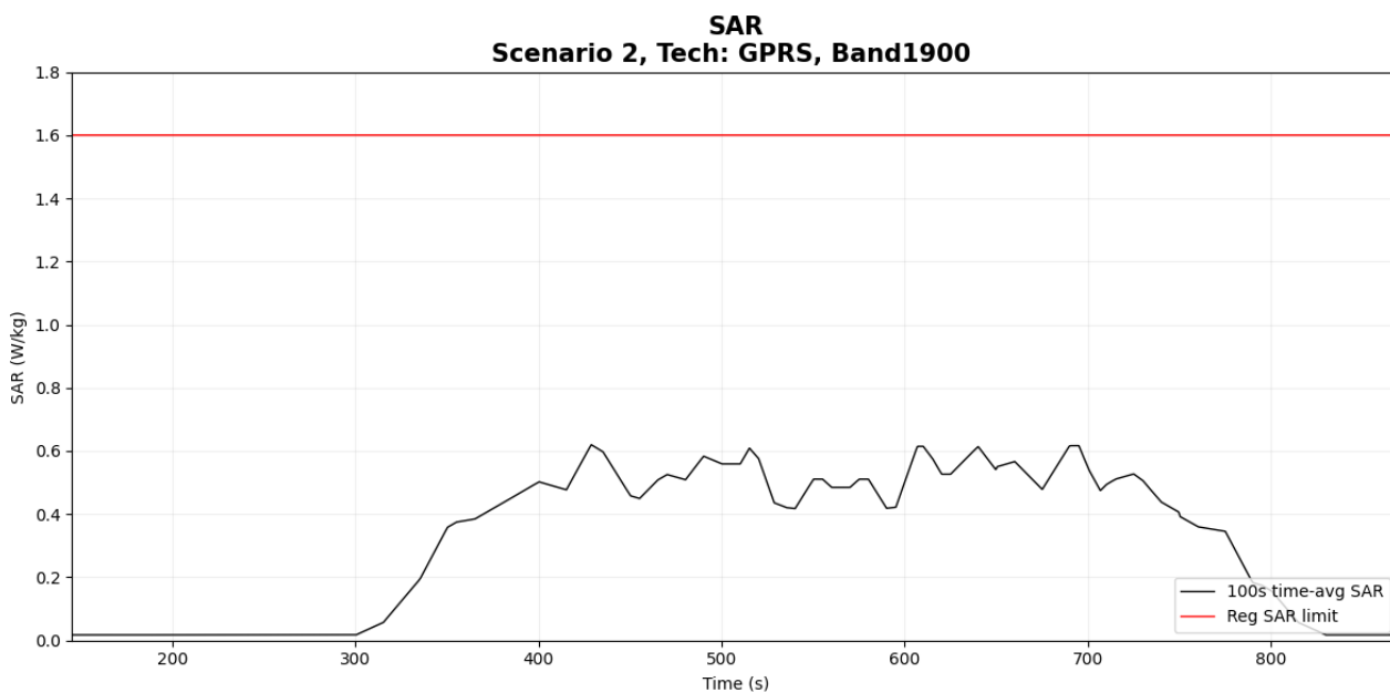
Figure 6- 14 Time-averaged SAR
