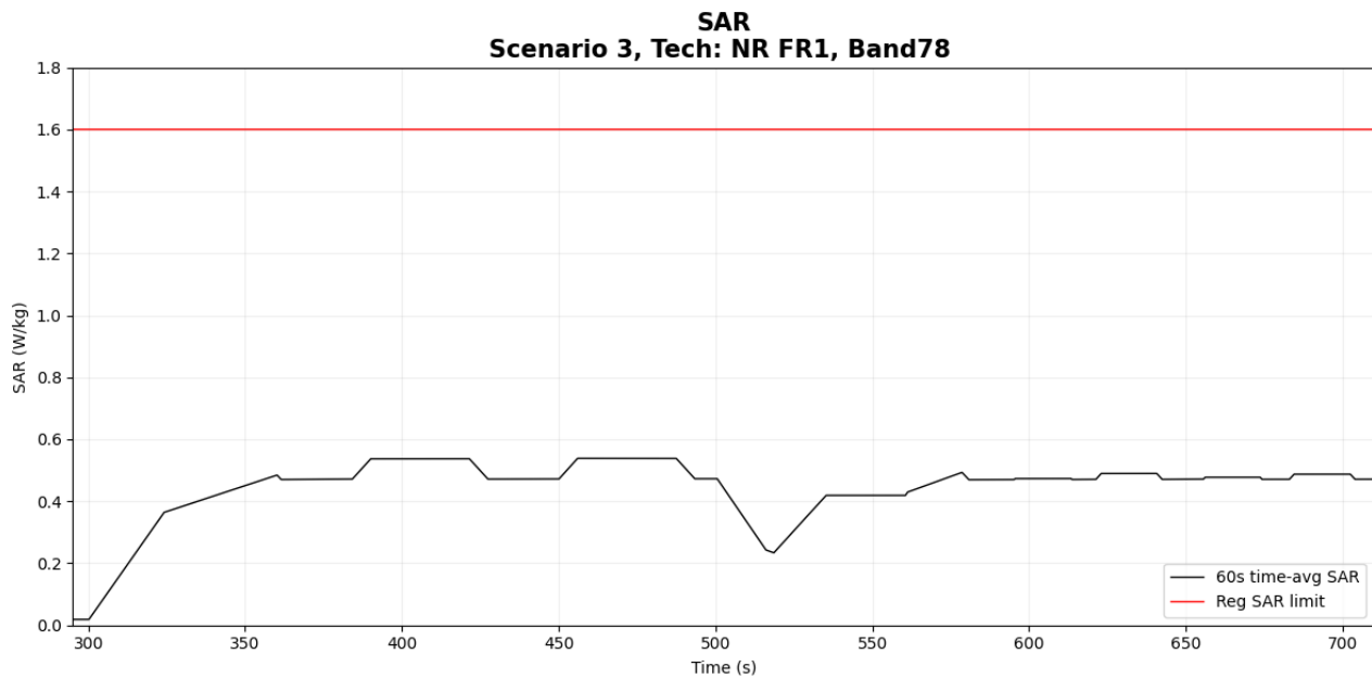
Figure 6- 40 Time-averaged SAR
