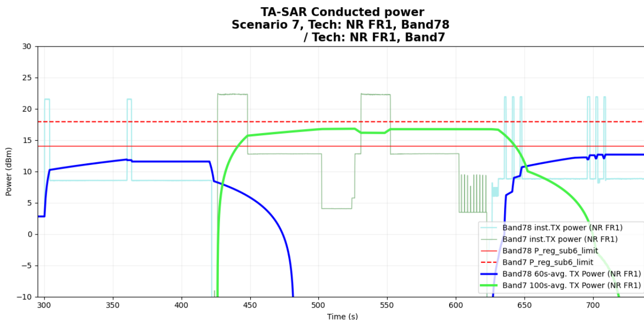
Figure 6- 45 Time-averaged conducted TX power over time
