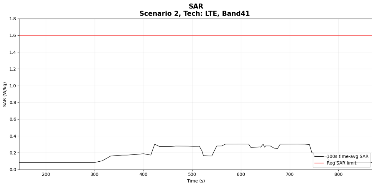
Figure 6- 30 Time-averaged SAR
